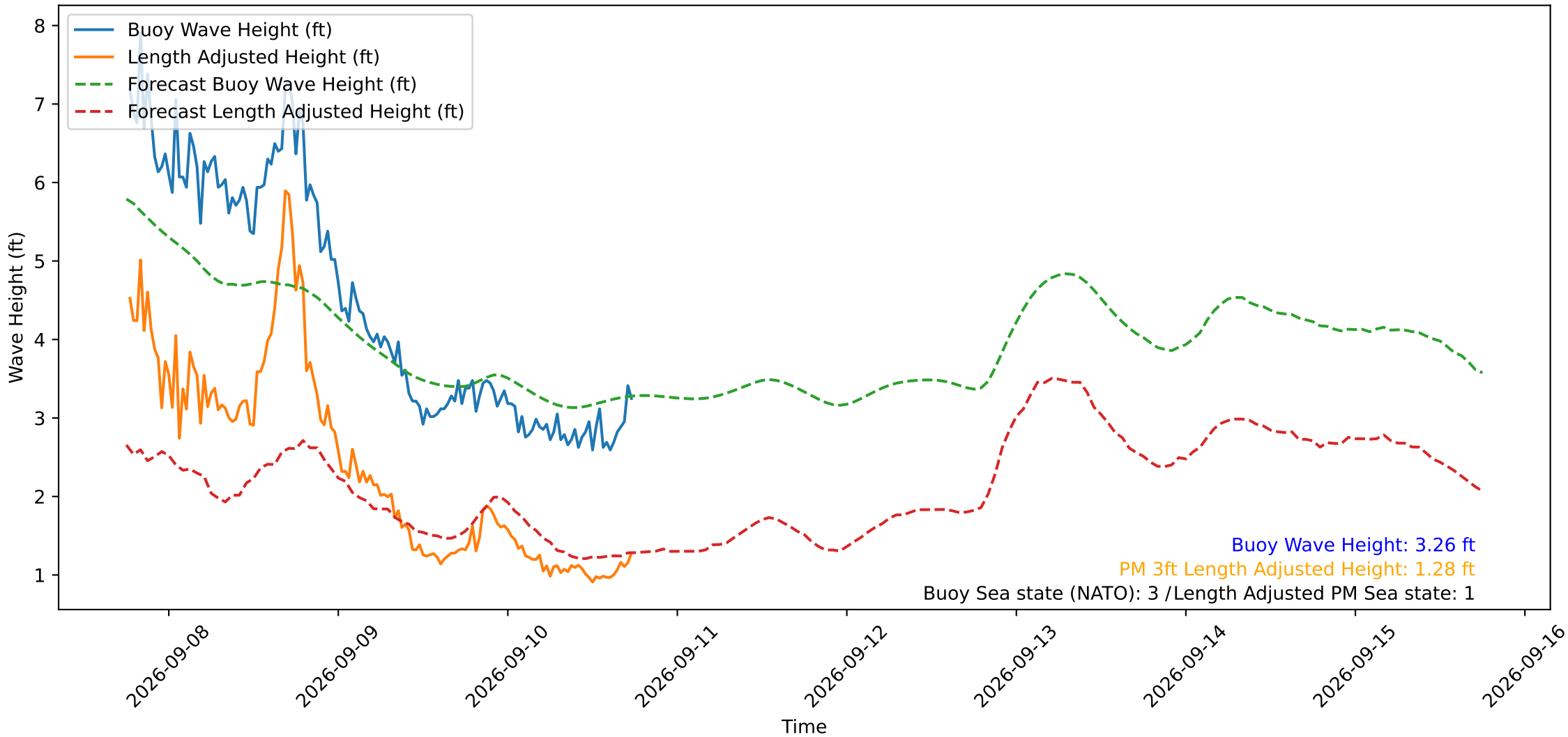
Wave Heights over Time for Green Beach at 2026-09-10 18:21:15
