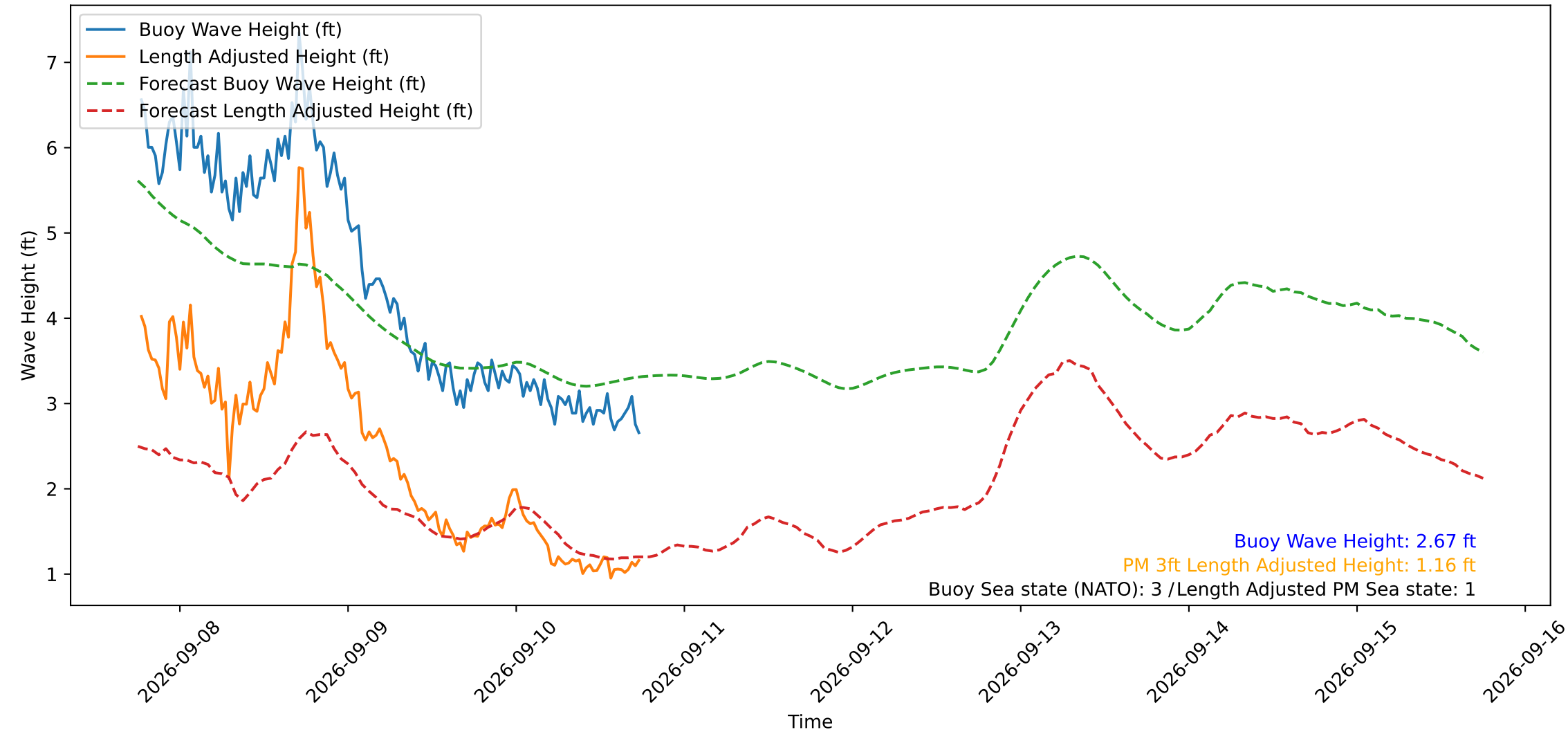
Wave Heights over Time for Oceanside Harbor at 2026-09-10 18:20:29
