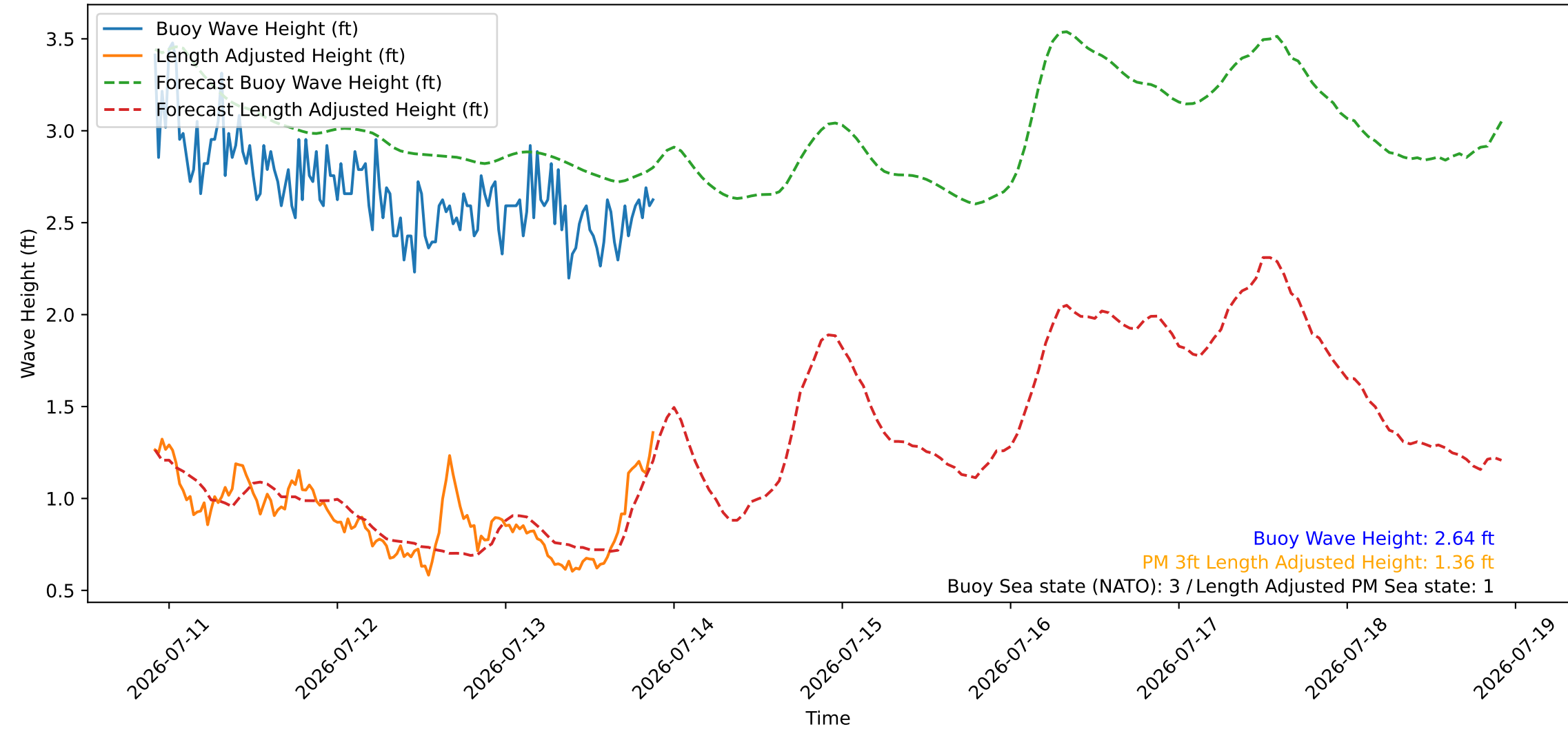
Wave Heights over Time for Green Beach at 2026-07-13 21:51:10
