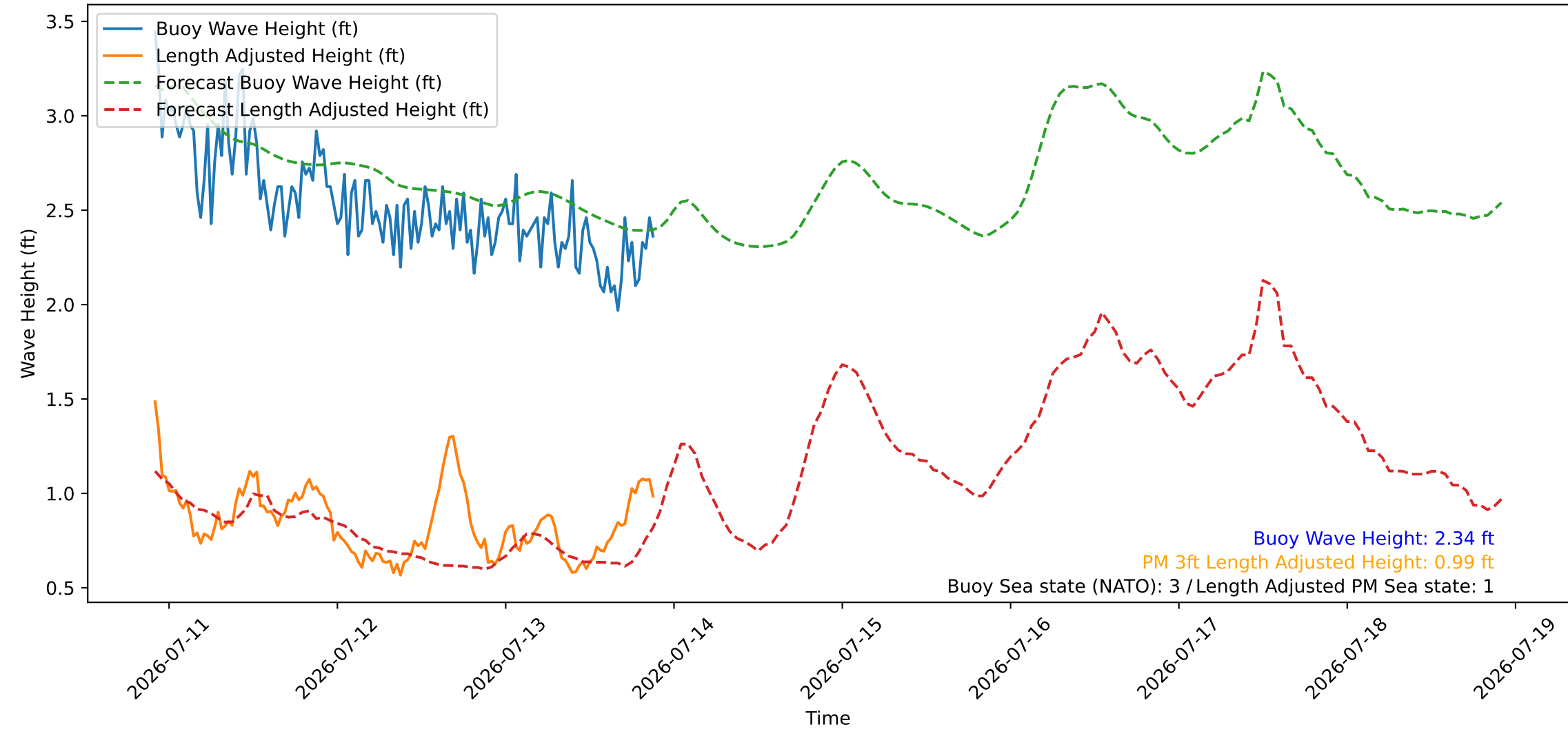
Wave Heights over Time for Red Beach at 2026-07-13 21:50:47
