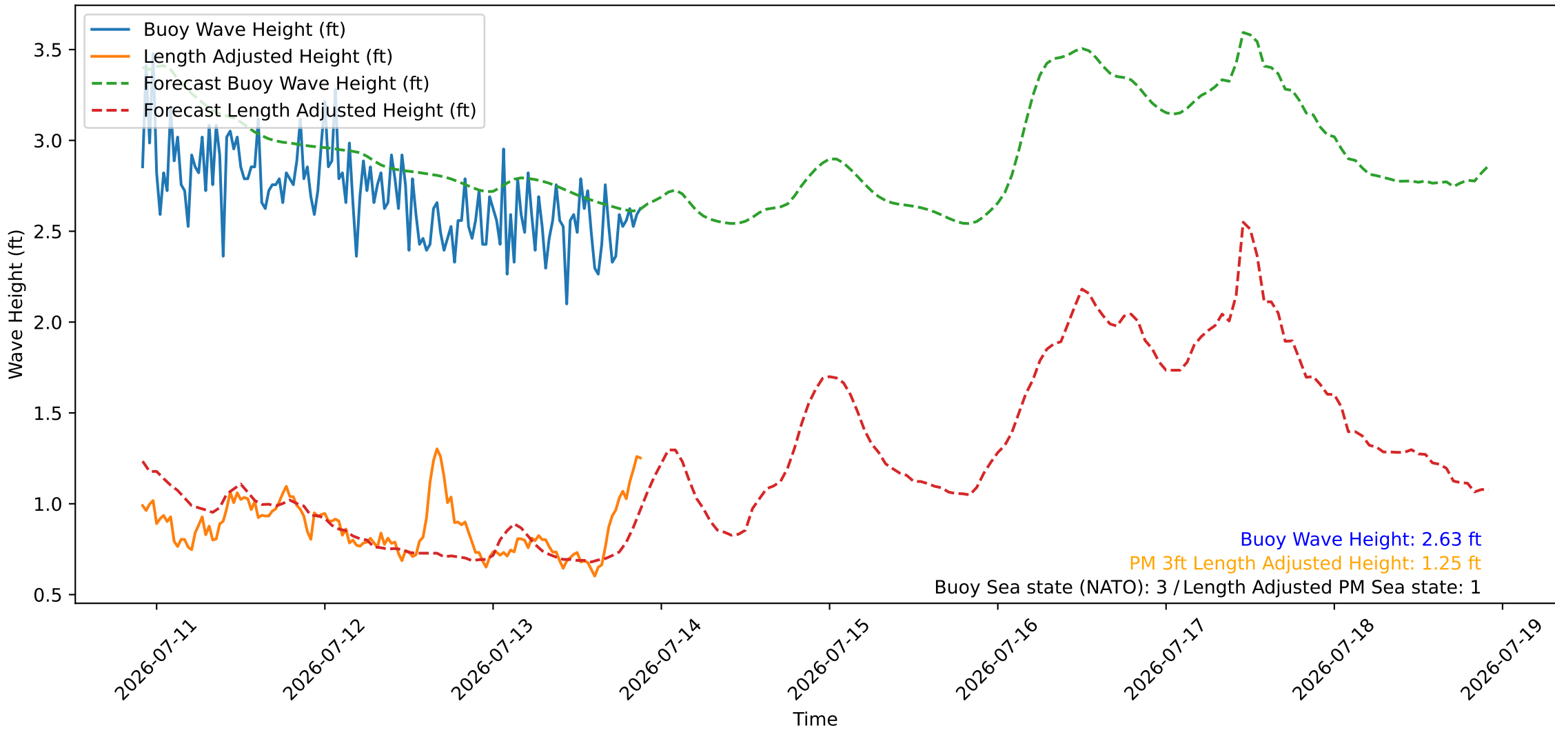
Wave Heights over Time for Oceanside Harbor at 2026-07-13 21:50:26
