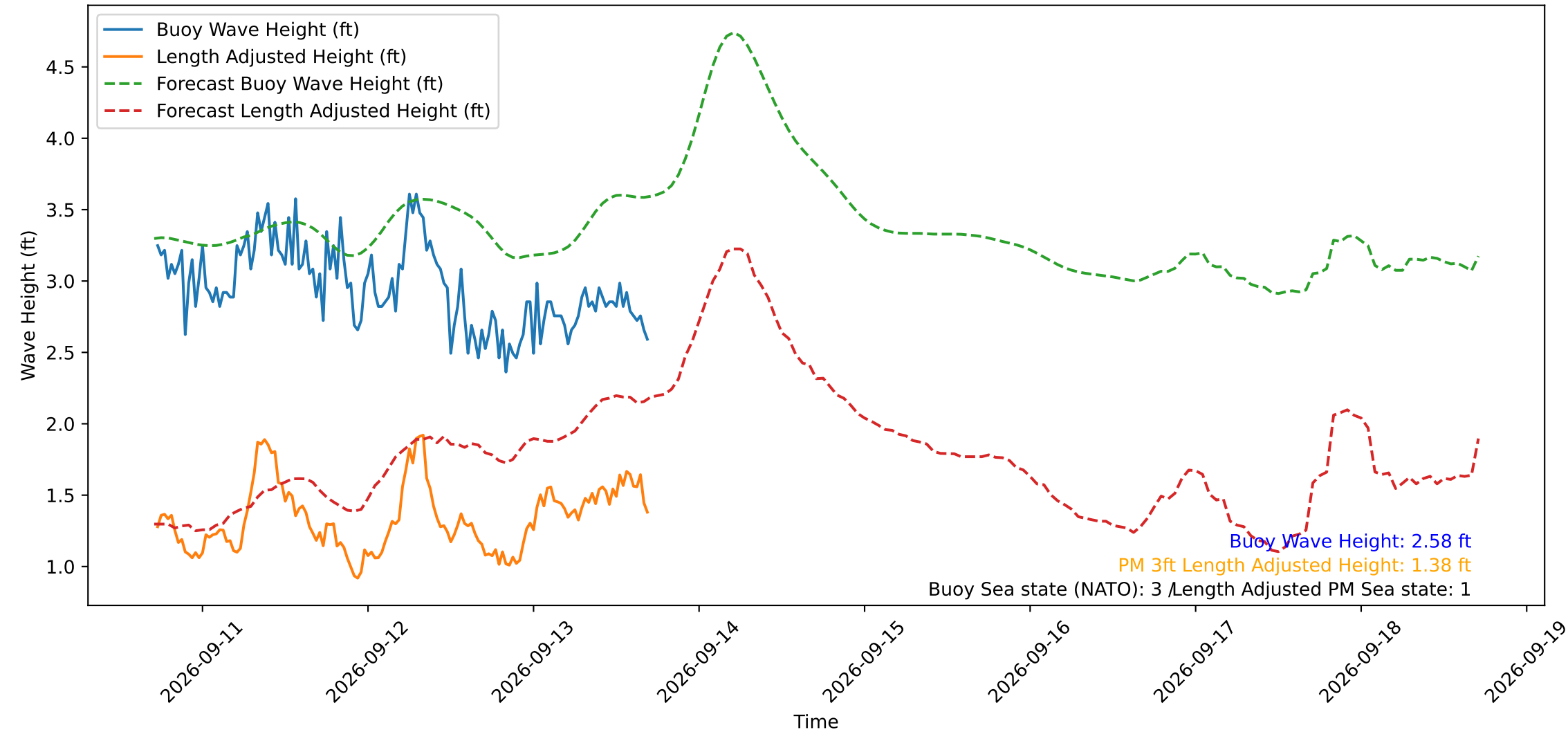
Wave Heights over Time for Green Beach at 2026-09-13 17:11:12
