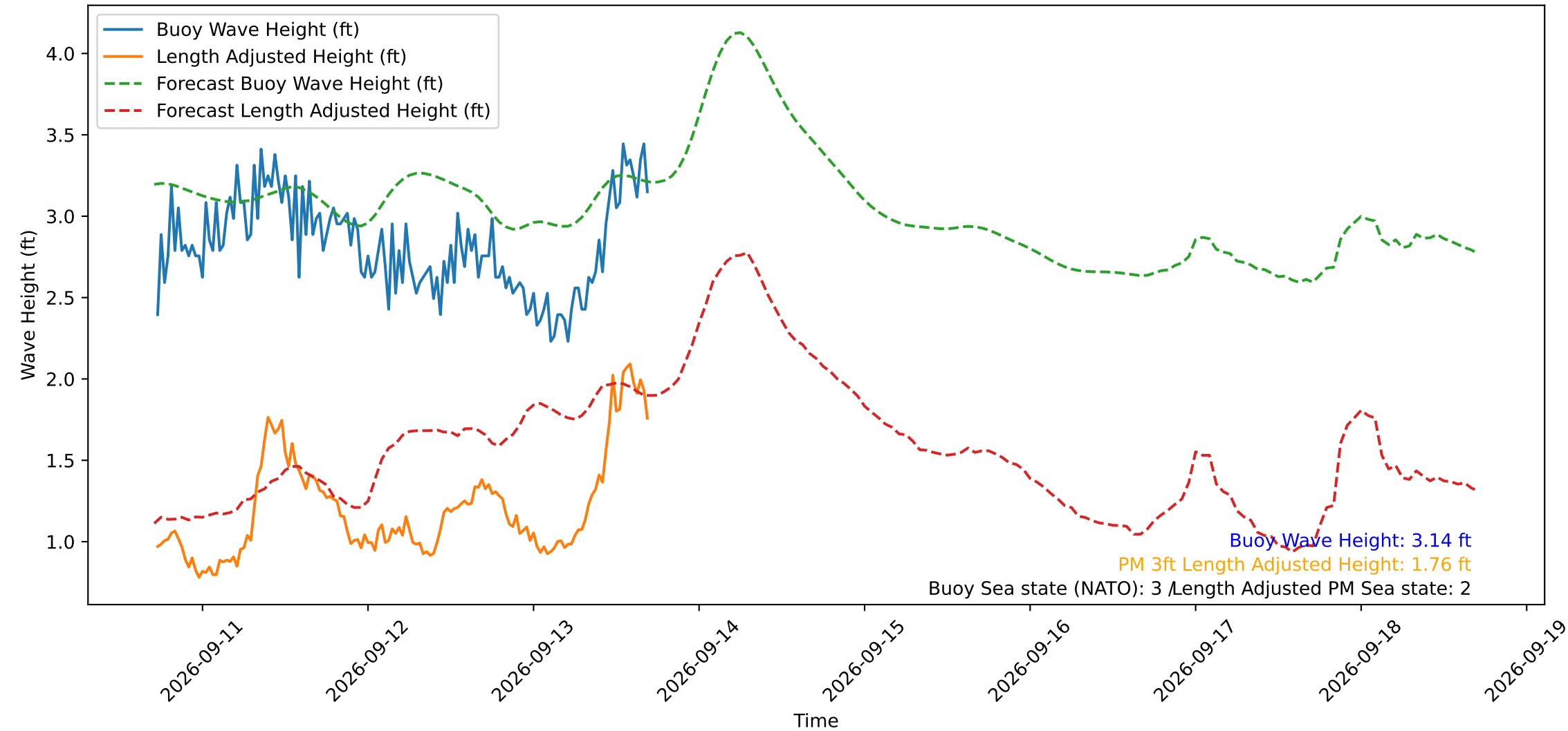
Wave Heights over Time for Red Beach at 2026-09-13 17:10:49
