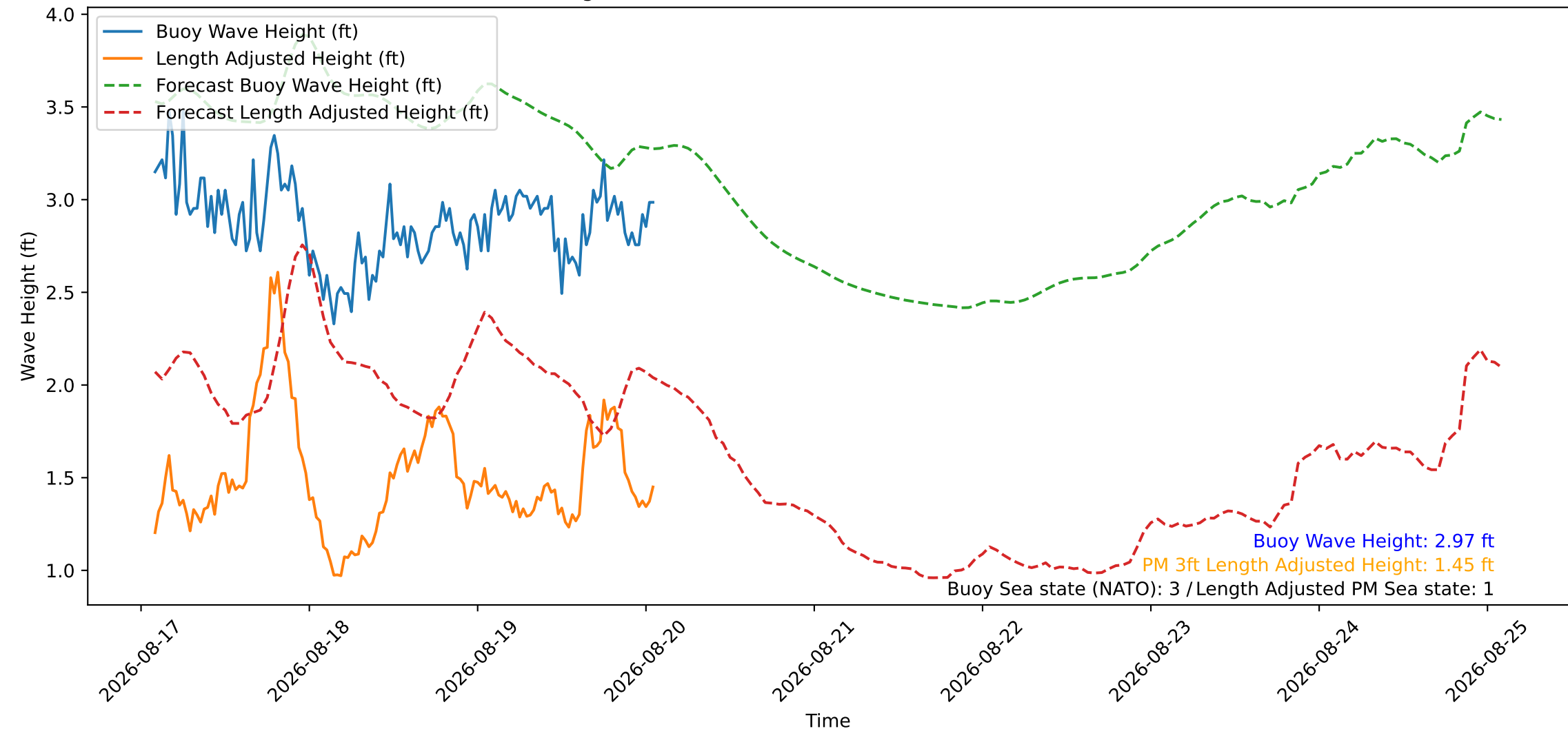
Wave Heights over Time for Red Beach at 2026-08-20 01:50:46
