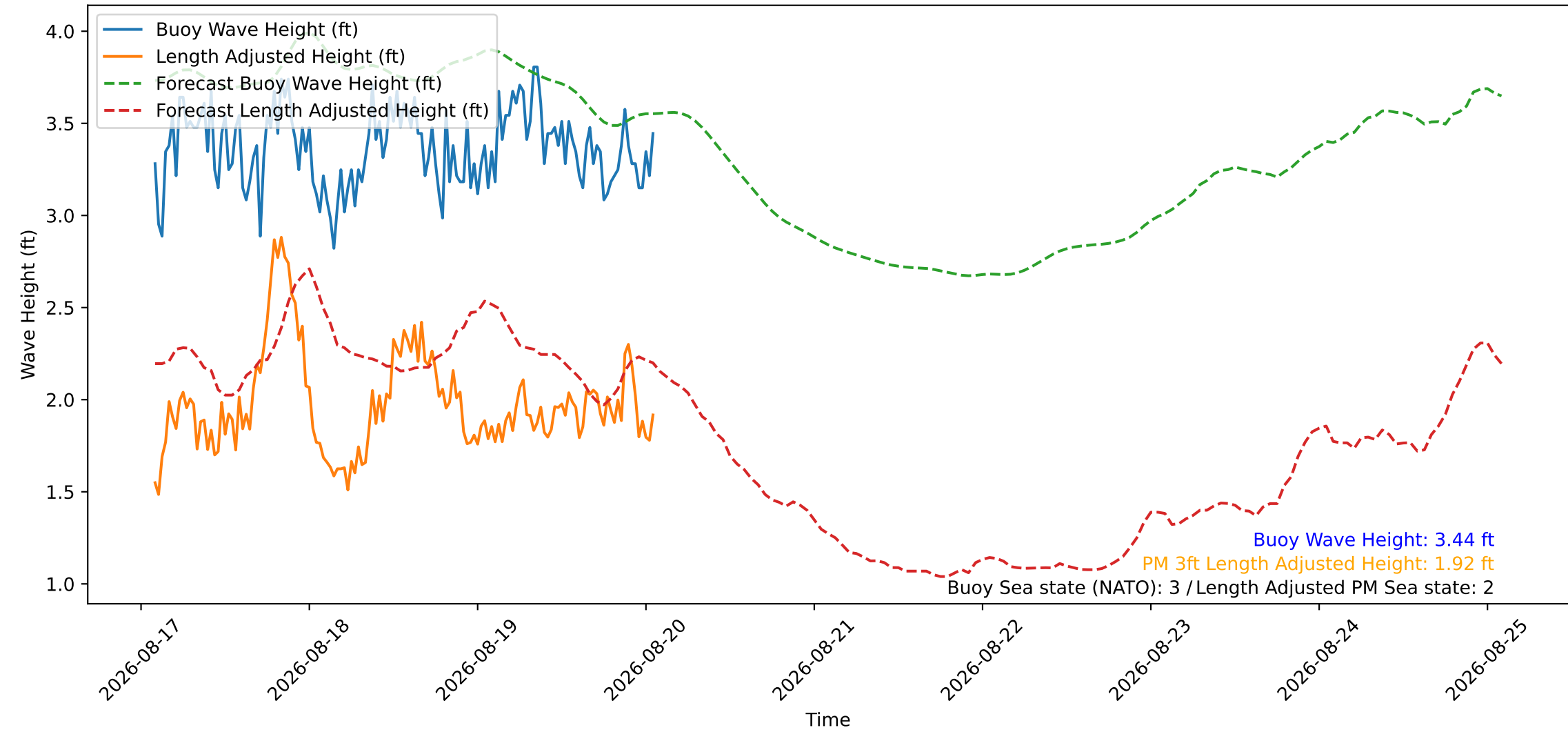
Wave Heights over Time for Oceanside Harbor at 2026-08-20 01:50:26
