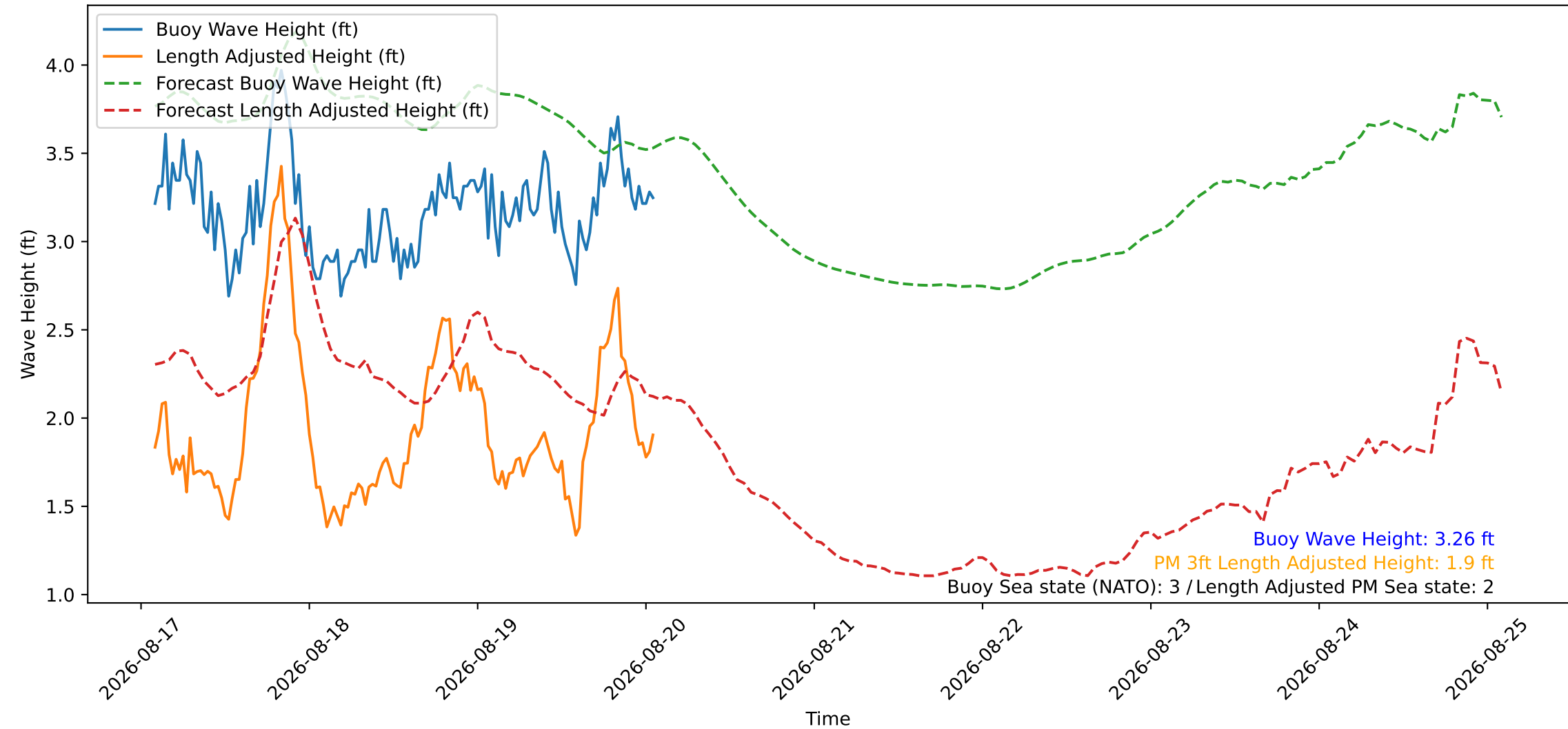
Wave Heights over Time for Green Beach at 2026-08-20 01:51:10
