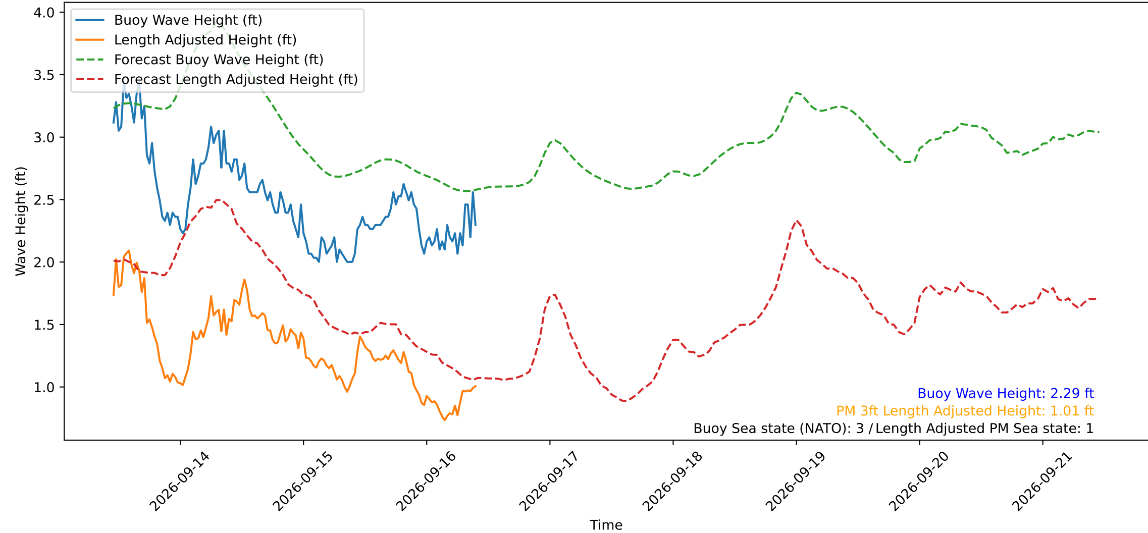
Wave Heights over Time for Red Beach at 2026-09-16 10:30:50
