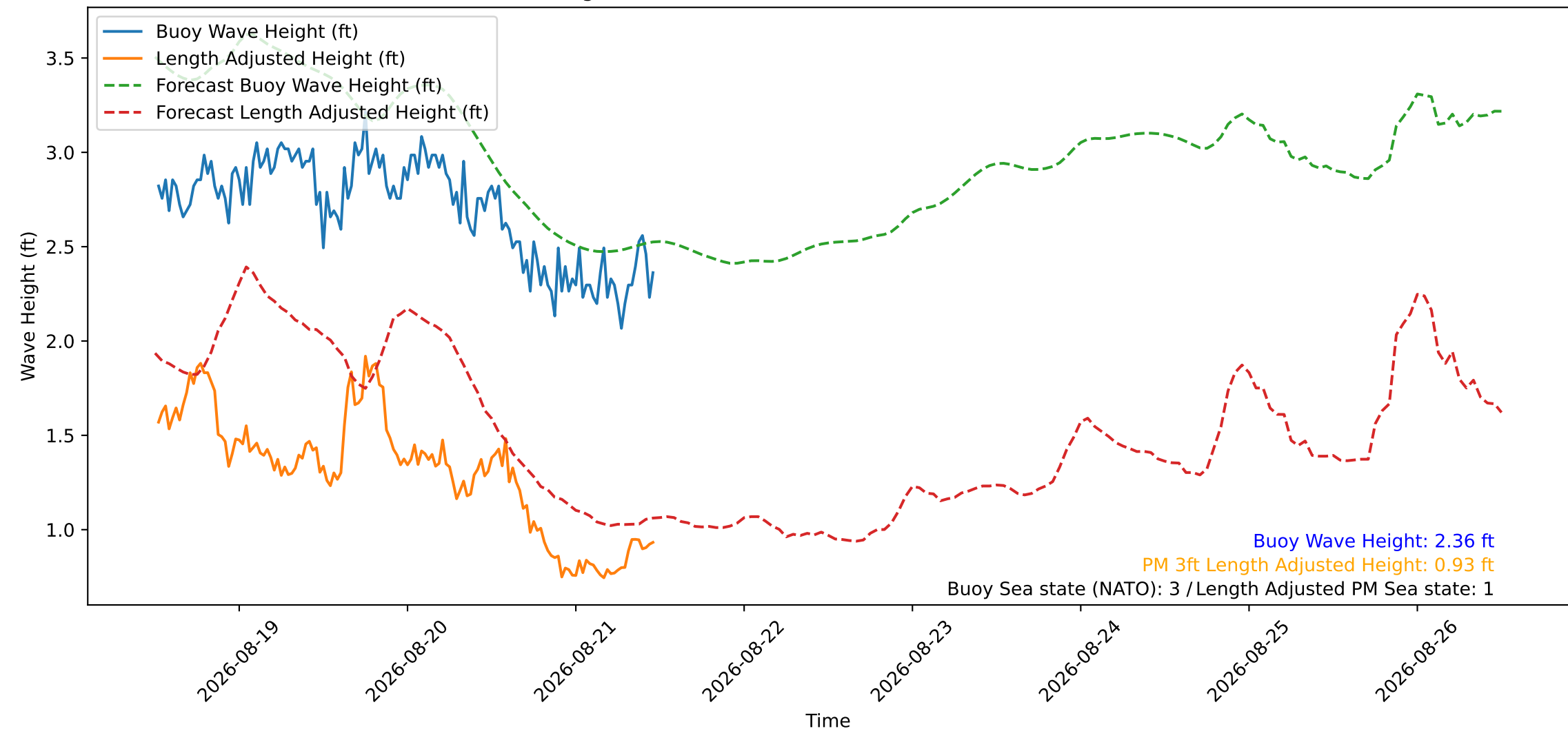
Wave Heights over Time for Red Beach at 2026-08-21 12:00:46
