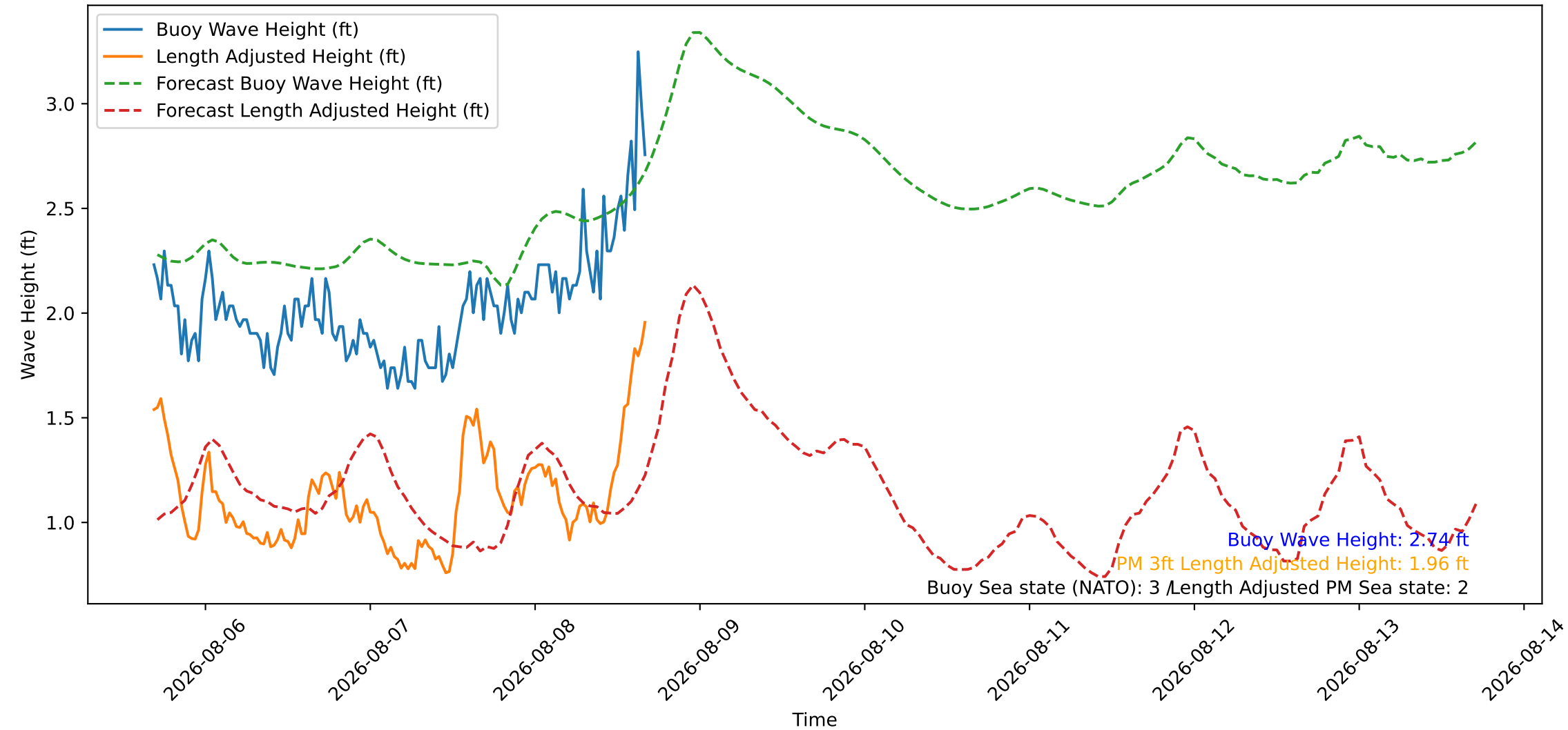
Wave Heights over Time for Oceanside Harbor at 2026-08-08 16:40:25
