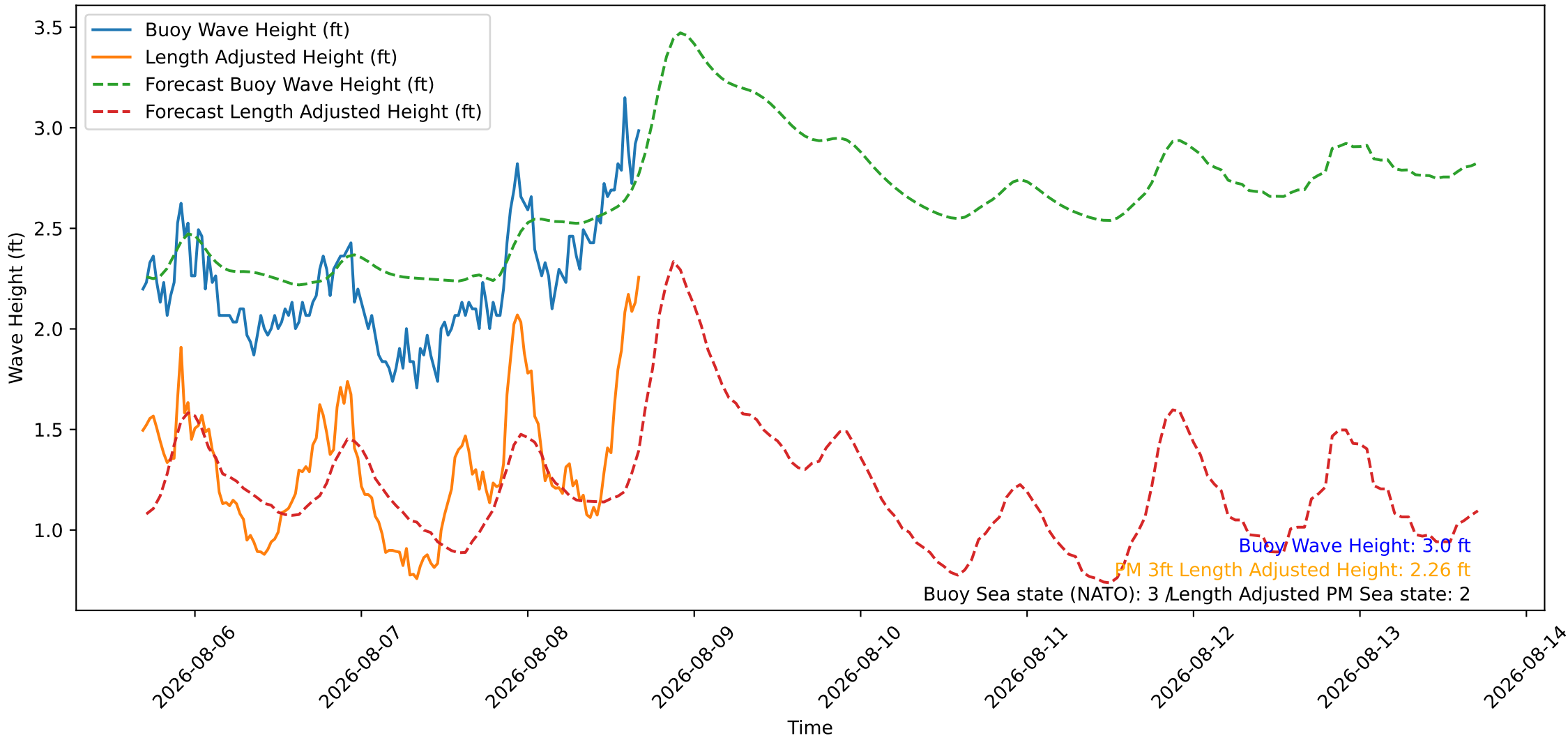
Wave Heights over Time for Green Beach at 2026-08-08 16:41:08
