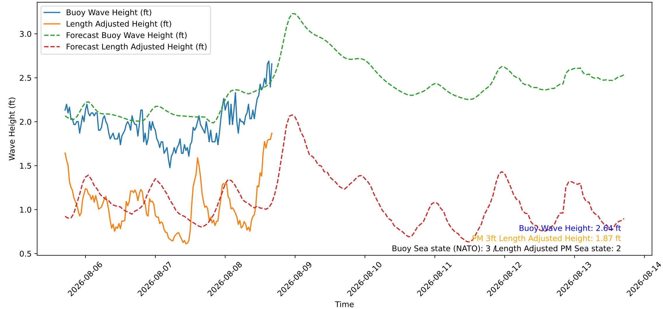
Wave Heights over Time for Red Beach at 2026-08-08 16:40:45
