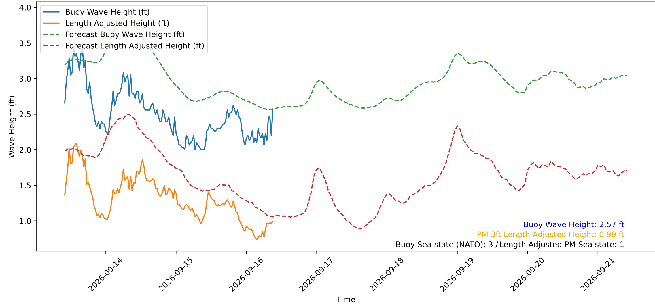
Wave Heights over Time for Red Beach at 2026-09-16 09:40:49
