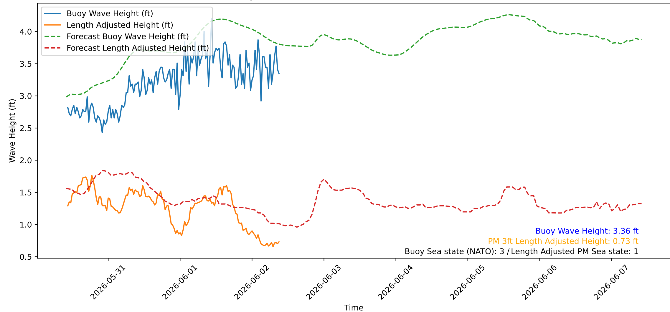
Wave Heights over Time for Red Beach at 2026-06-02 10:00:45
