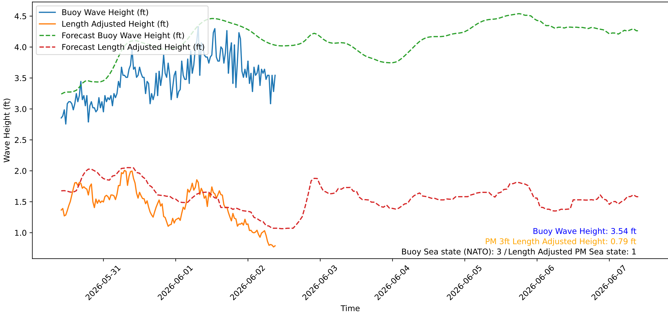
Wave Heights over Time for Green Beach at 2026-06-02 10:01:08
