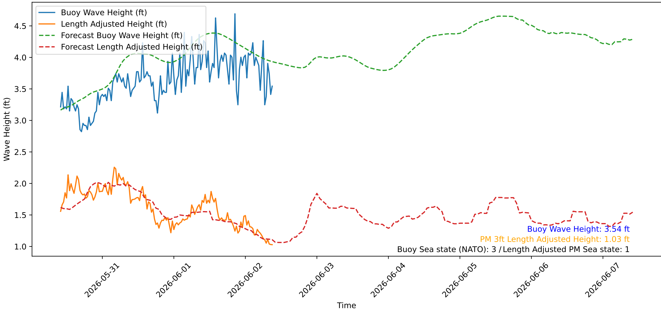
Wave Heights over Time for Oceanside Harbor at 2026-06-02 10:00:26
