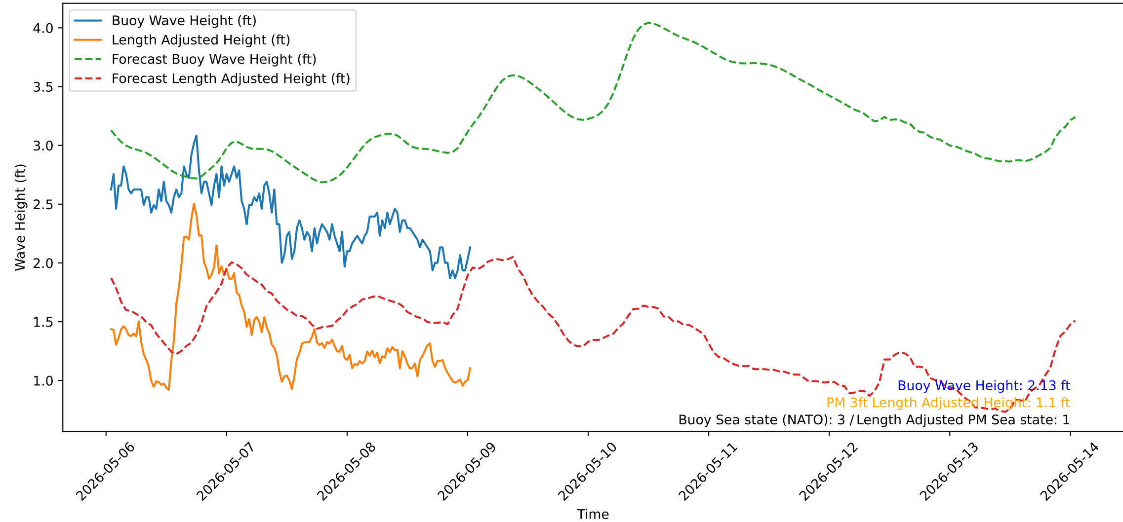
Wave Heights over Time for Oceanside Harbor at 2026-05-09 01:10:31
