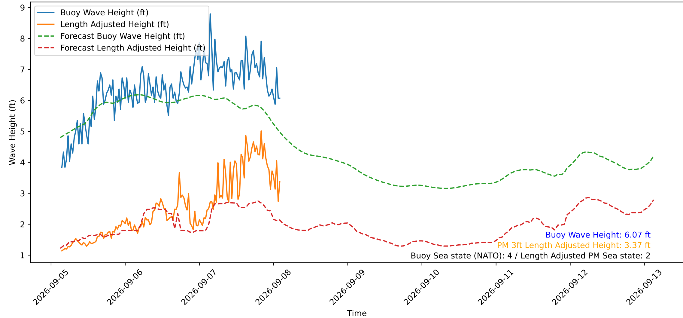
Wave Heights over Time for Green Beach at 2026-09-08 03:01:12
