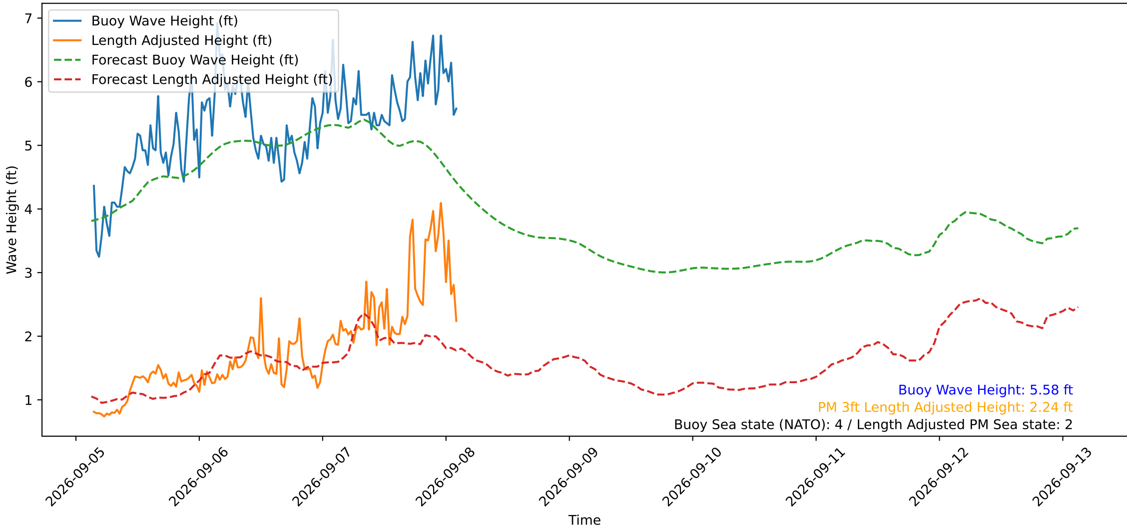
Wave Heights over Time for Red Beach at 2026-09-08 03:00:49
