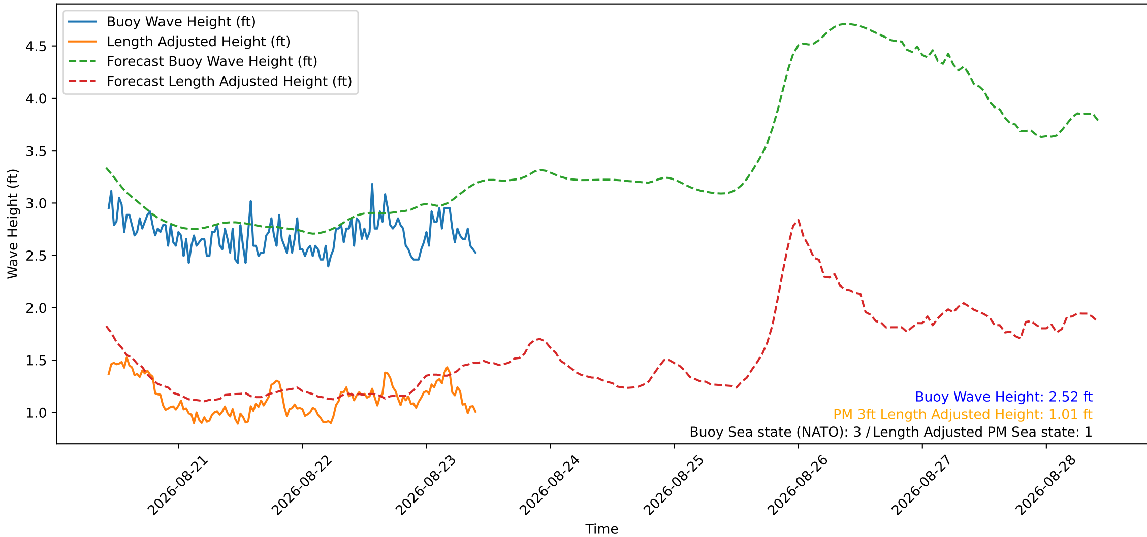
Wave Heights over Time for Green Beach at 2026-08-23 10:21:14
