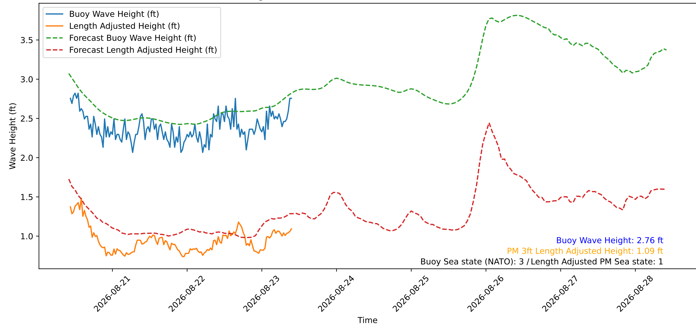
Wave Heights over Time for Red Beach at 2026-08-23 10:20:50
