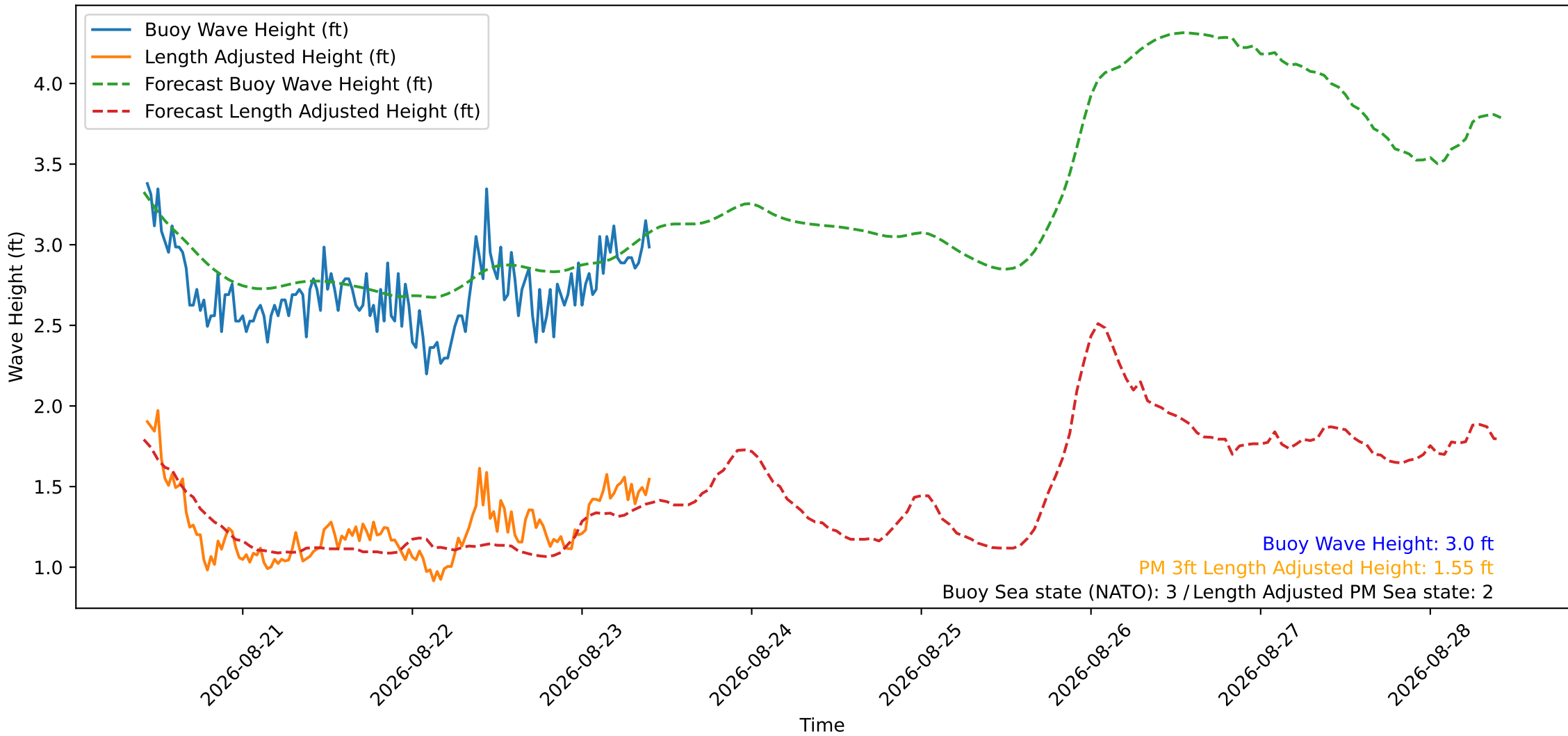
Wave Heights over Time for Oceanside Harbor at 2026-08-23 10:20:29
