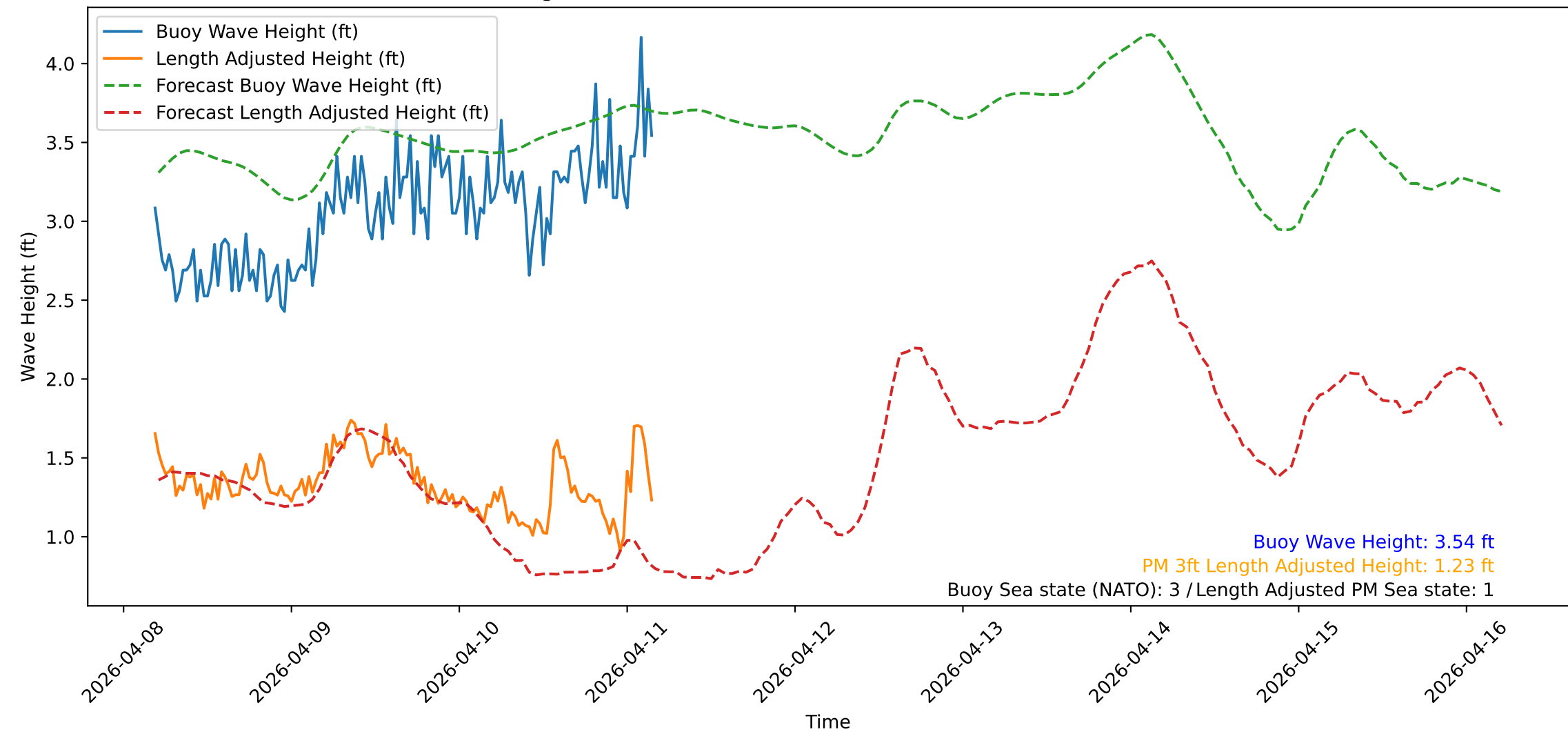
Wave Heights over Time for Oceanside Harbor at 2026-04-11 04:30:32
