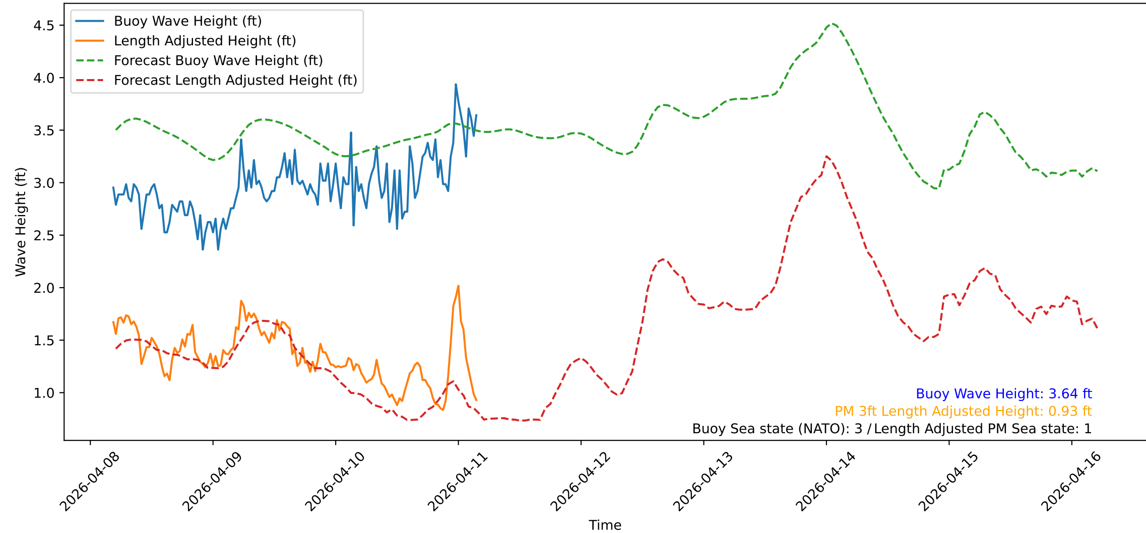
Wave Heights over Time for Green Beach at 2026-04-11 04:31:13
