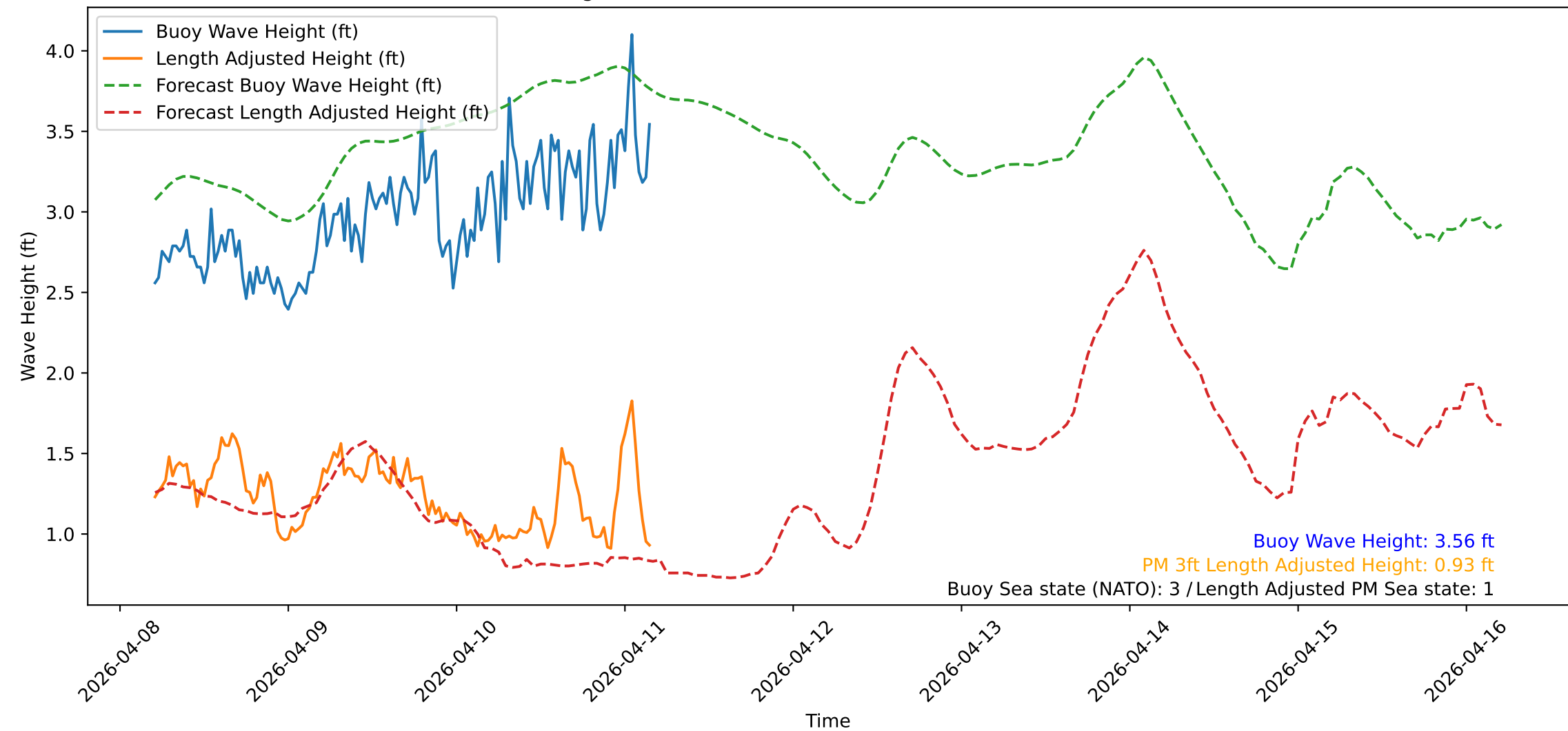
Wave Heights over Time for Red Beach at 2026-04-11 04:30:51
