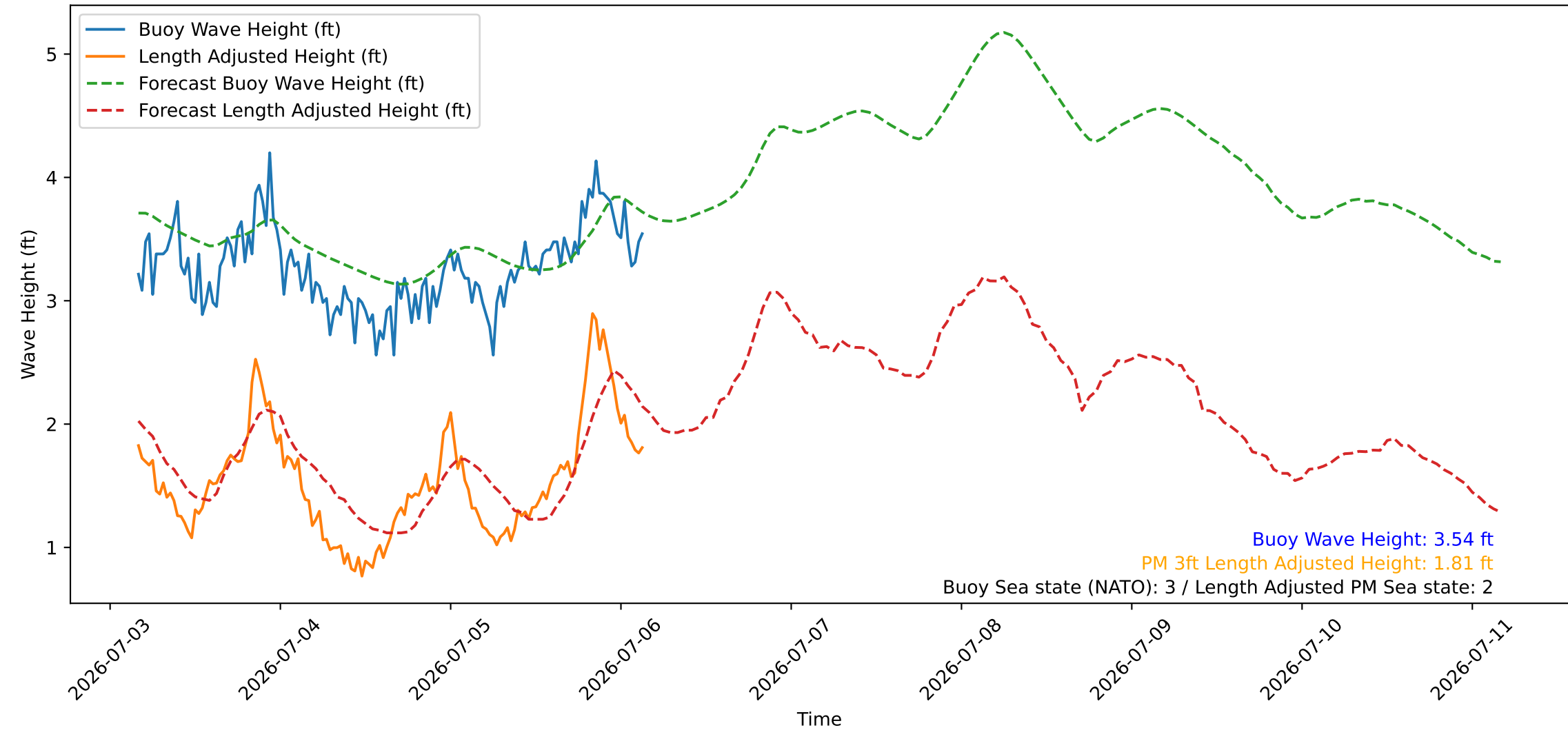
Wave Heights over Time for Green Beach at 2026-07-06 03:51:10
