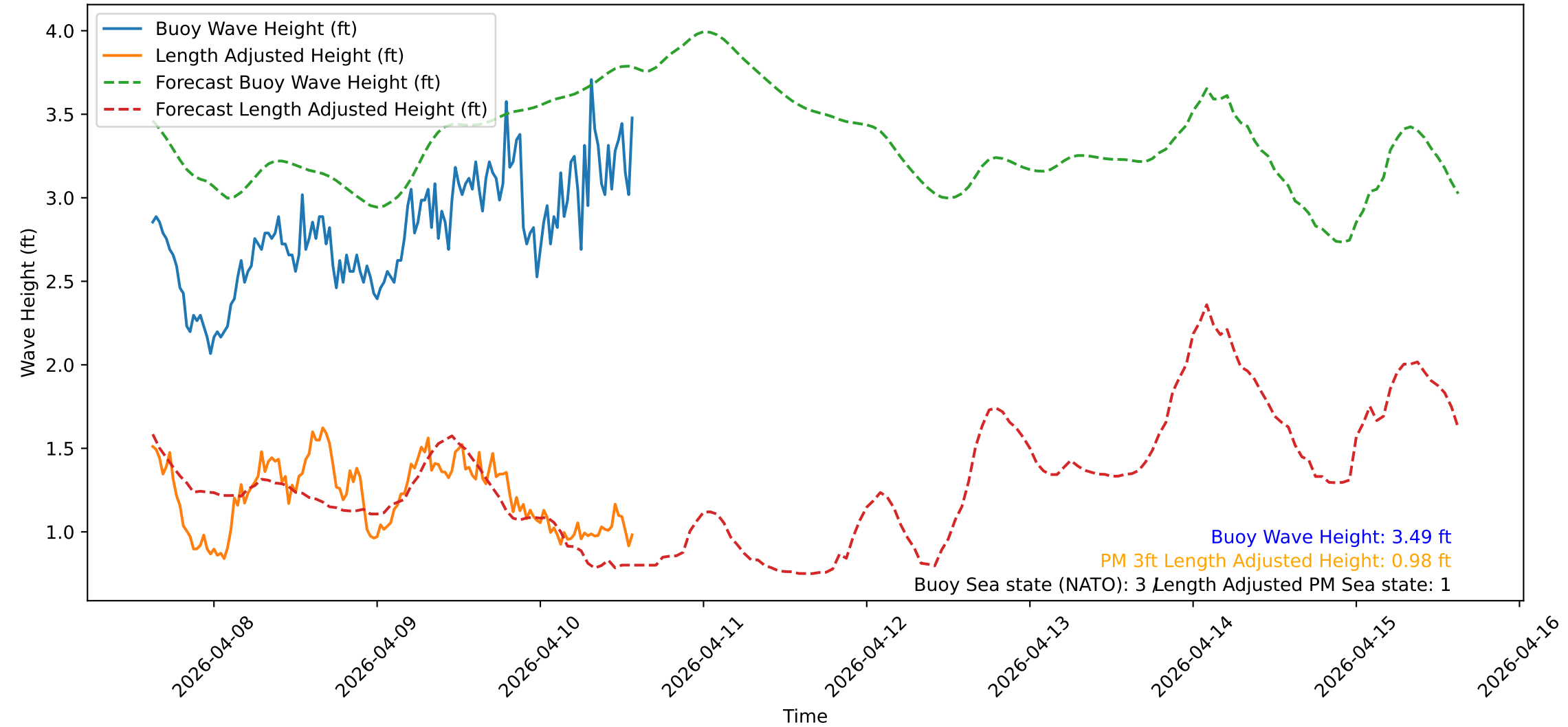
Wave Heights over Time for Red Beach at 2026-04-10 14:30:50
