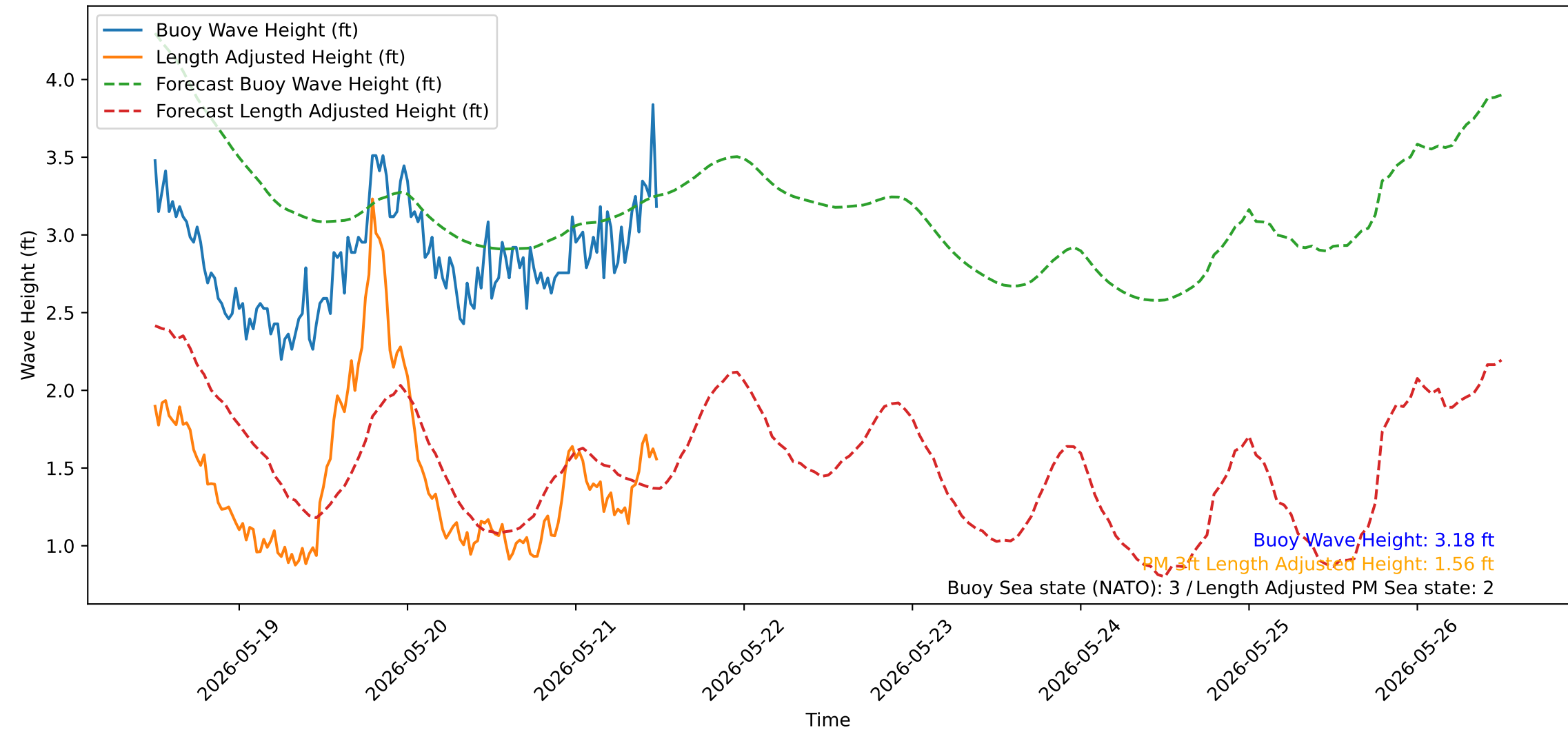
Wave Heights over Time for Oceanside Harbor at 2026-05-21 12:00:31
