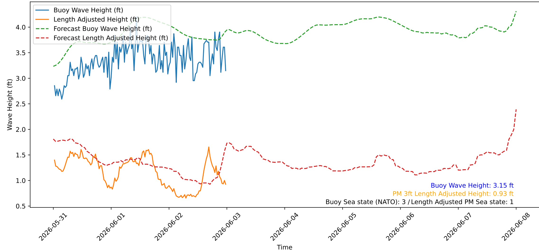
Wave Heights over Time for Red Beach at 2026-06-03 00:10:45
