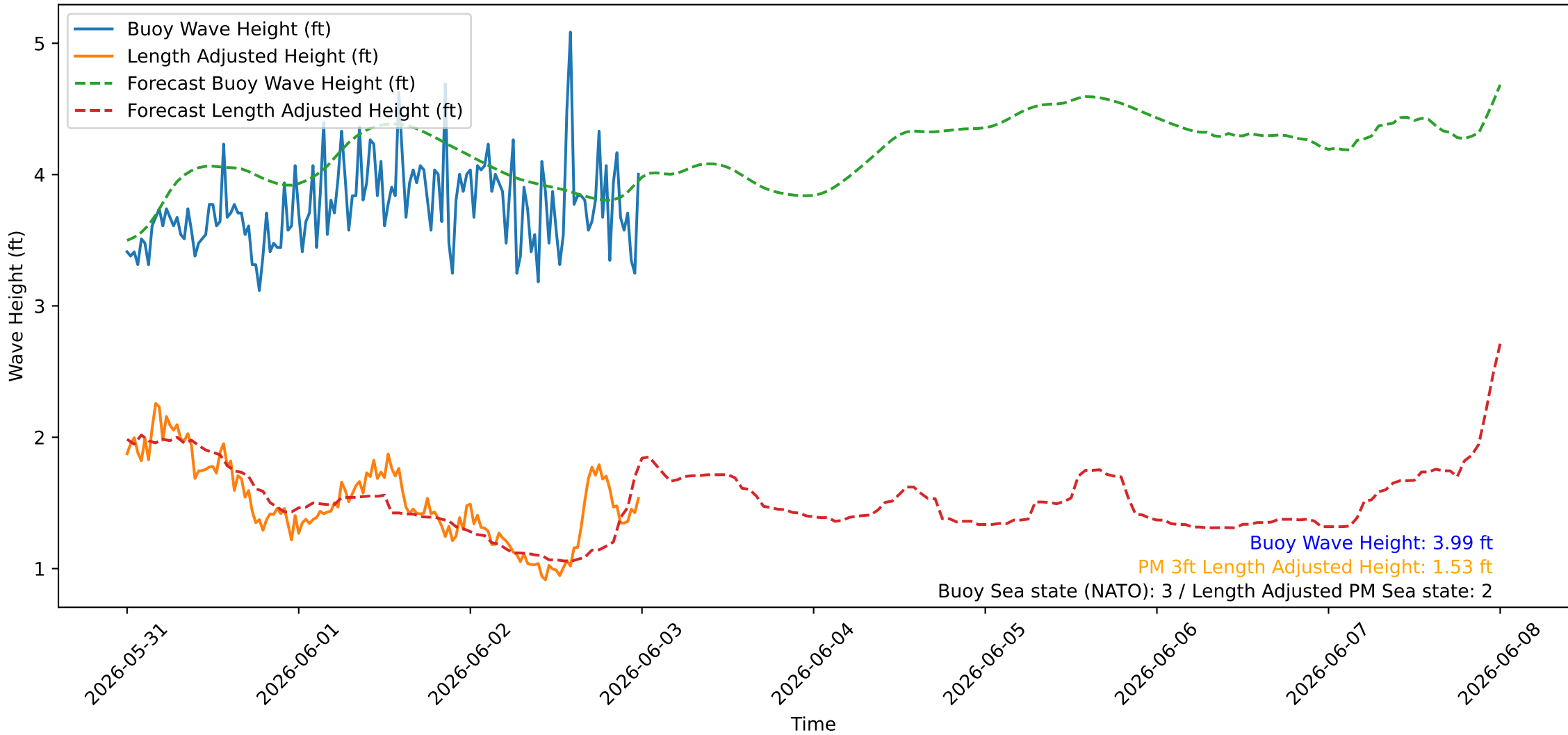
Wave Heights over Time for Oceanside Harbor at 2026-06-03 00:10:26
