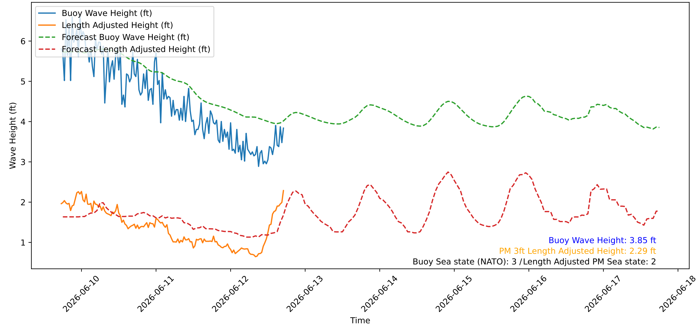
Wave Heights over Time for Green Beach at 2026-06-12 17:41:09
