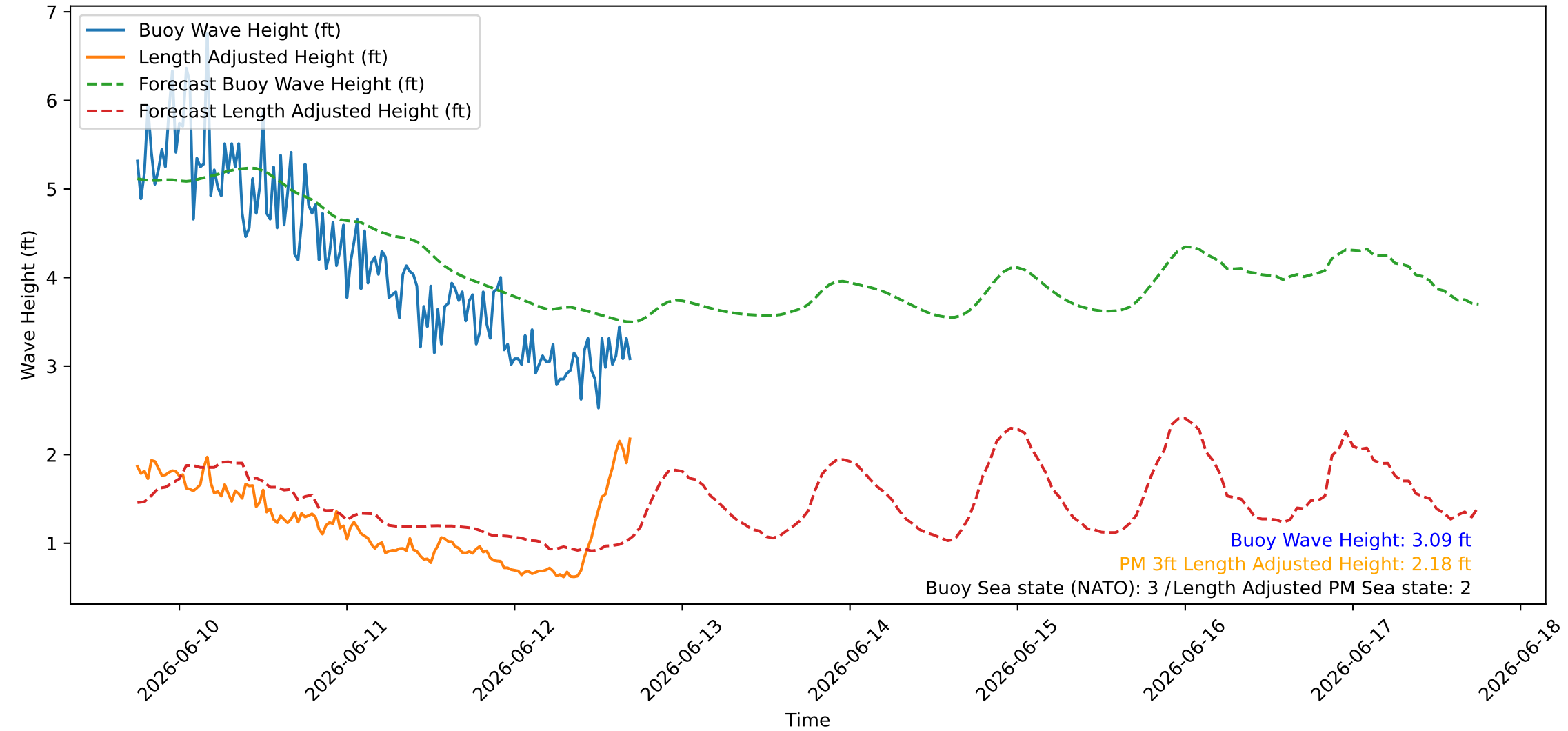
Wave Heights over Time for Red Beach at 2026-06-12 17:40:46
