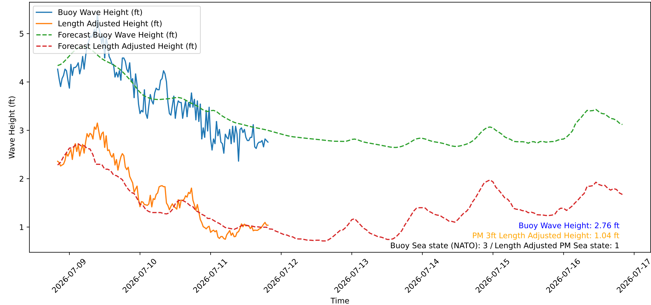
Wave Heights over Time for Oceanside Harbor at 2026-07-11 20:10:26
