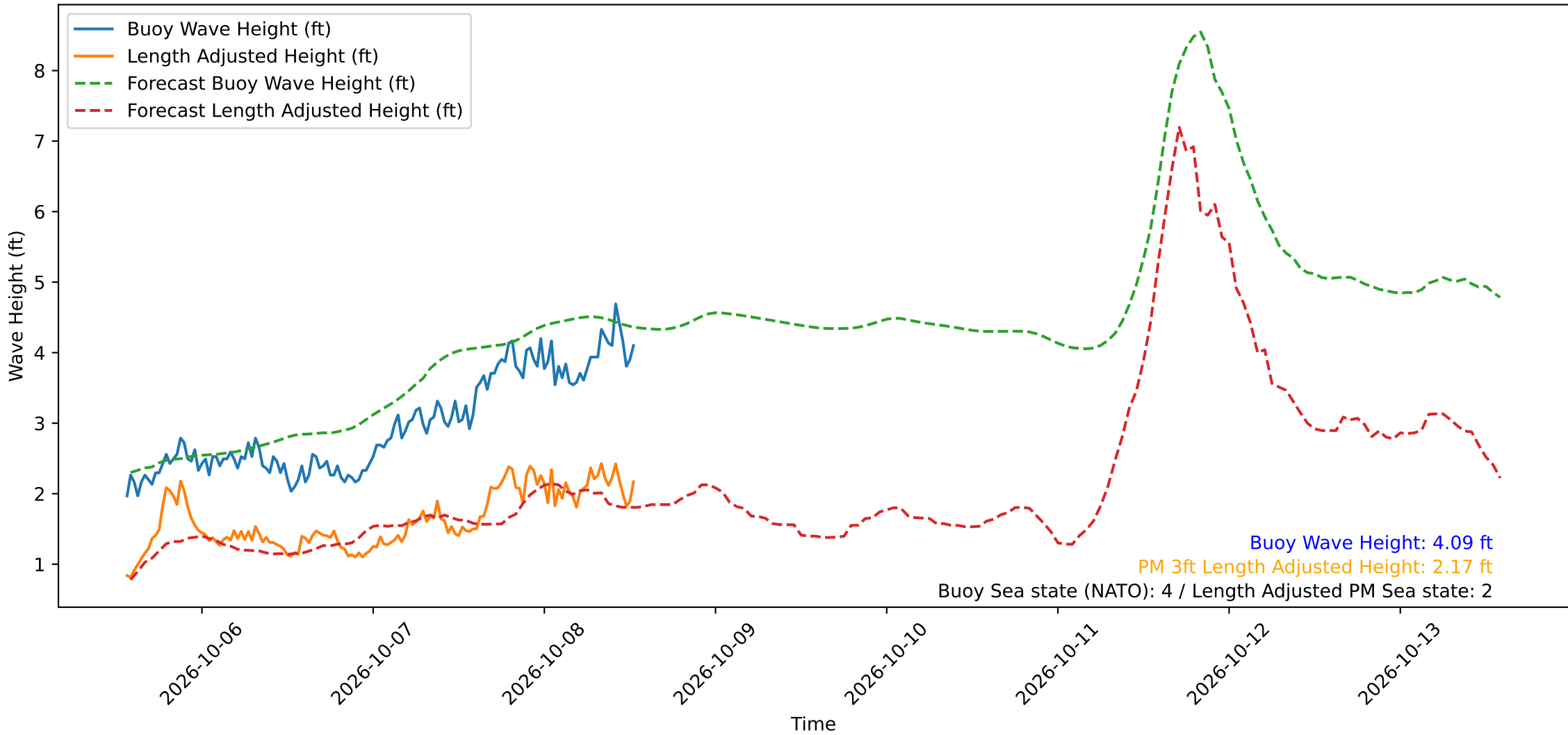
Wave Heights over Time for Oceanside Harbor at 2026-10-08 13:30:30
