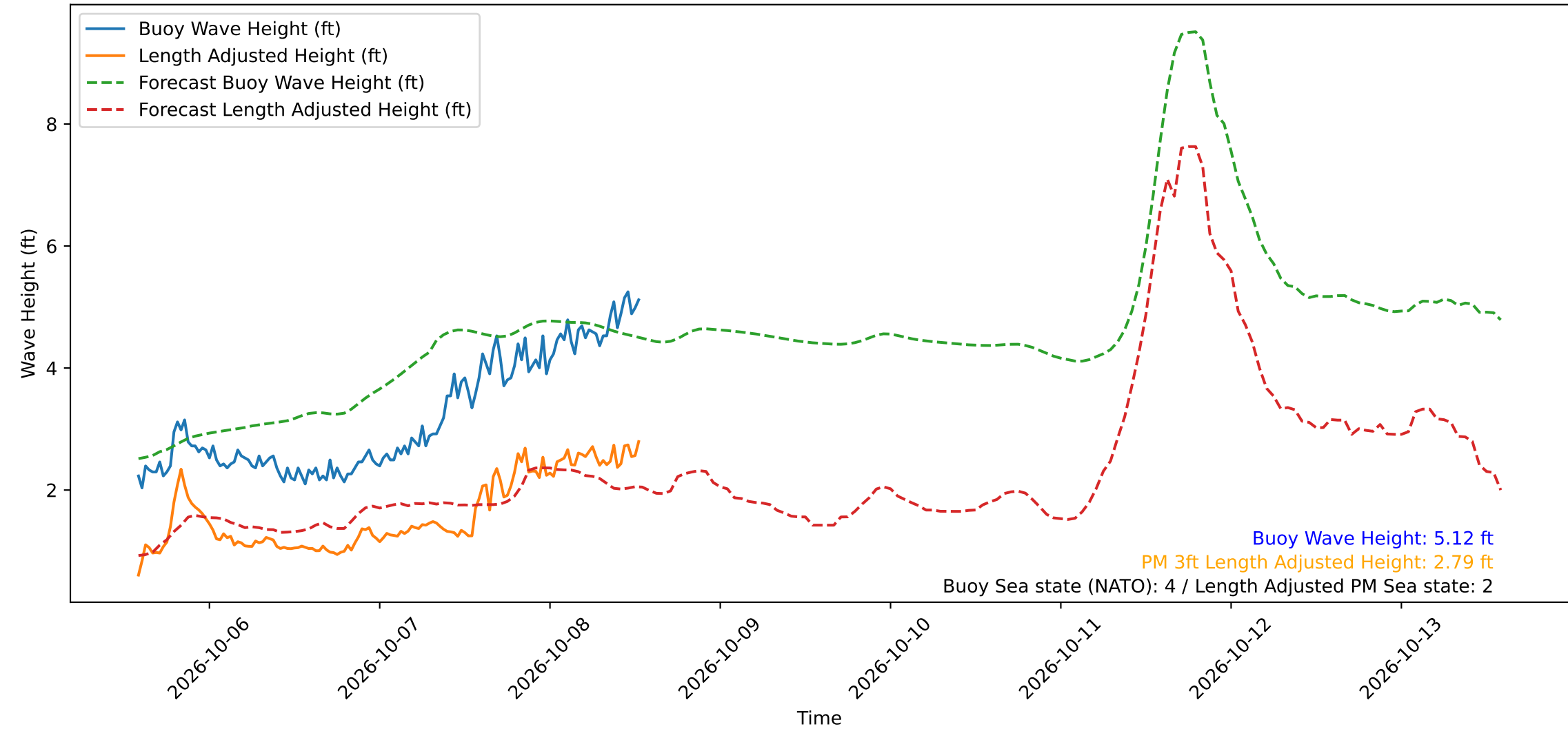
Wave Heights over Time for Green Beach at 2026-10-08 13:31:13
