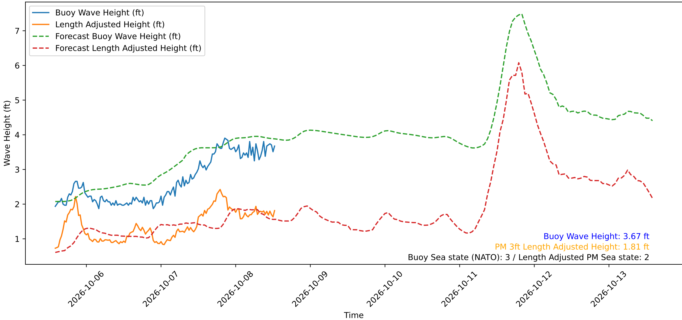
Wave Heights over Time for Red Beach at 2026-10-08 13:30:51
