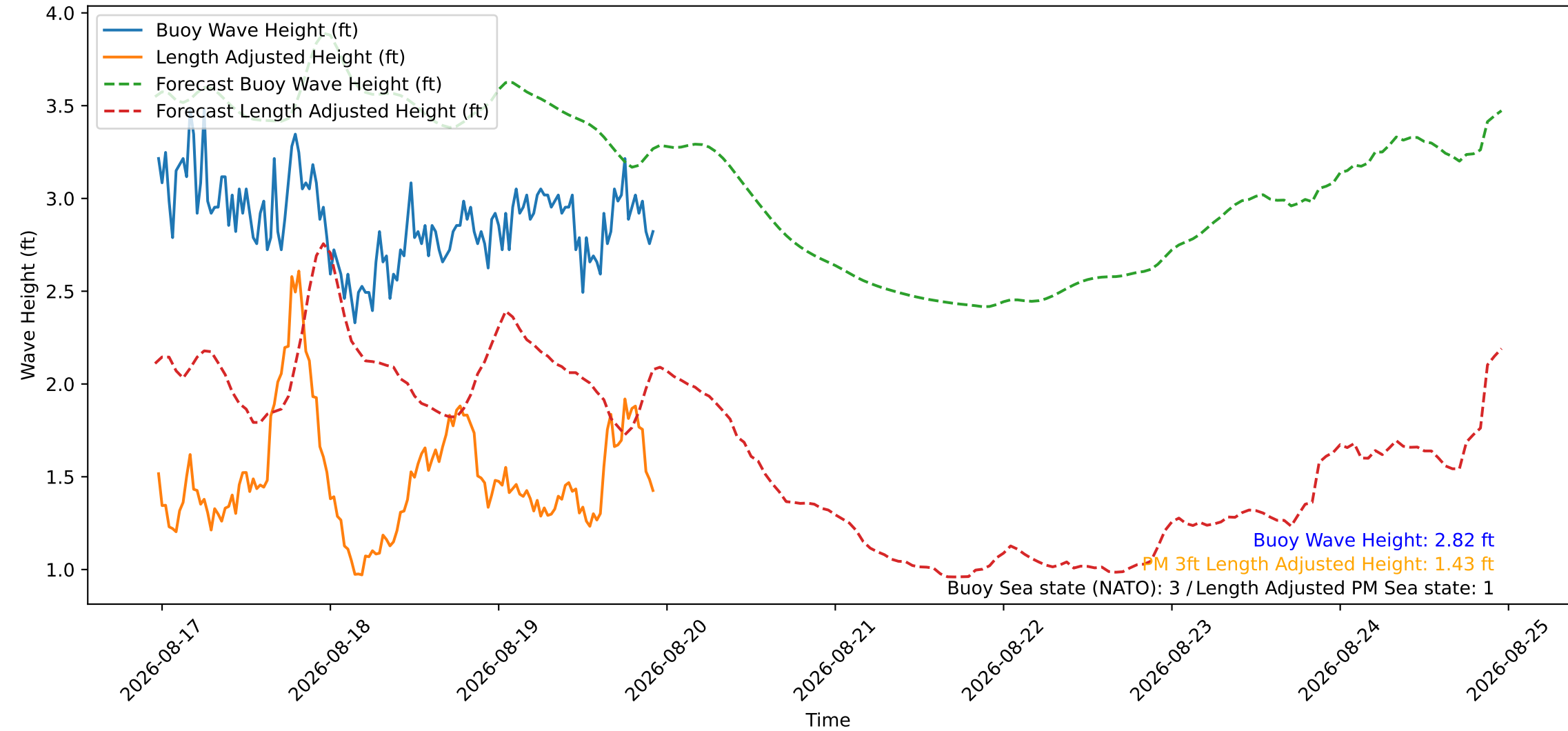
Wave Heights over Time for Red Beach at 2026-08-19 23:00:47
