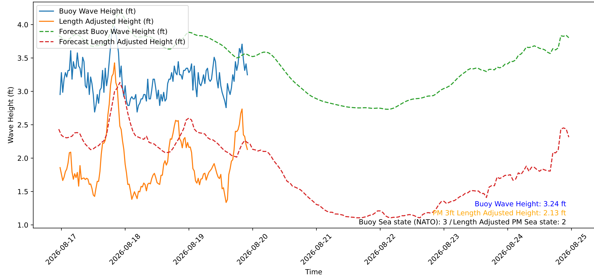
Wave Heights over Time for Green Beach at 2026-08-19 23:01:09
