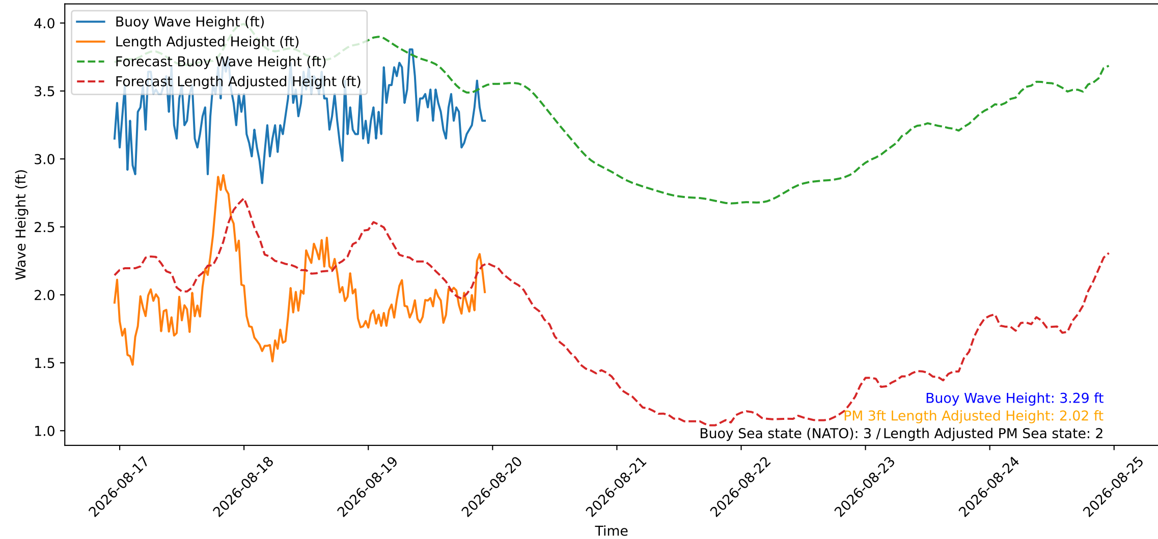
Wave Heights over Time for Oceanside Harbor at 2026-08-19 23:00:27
