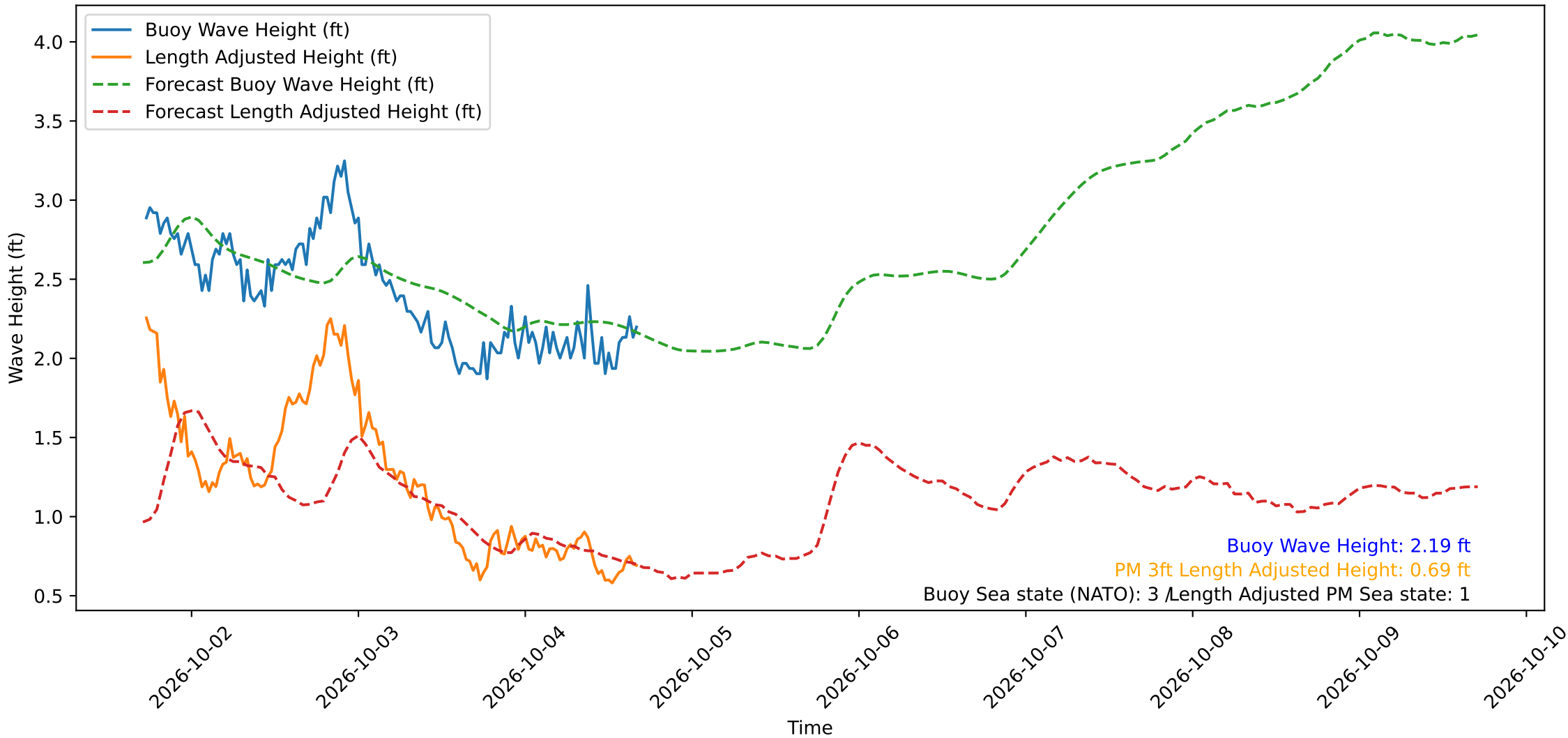
Wave Heights over Time for Red Beach at 2026-10-04 17:10:49
