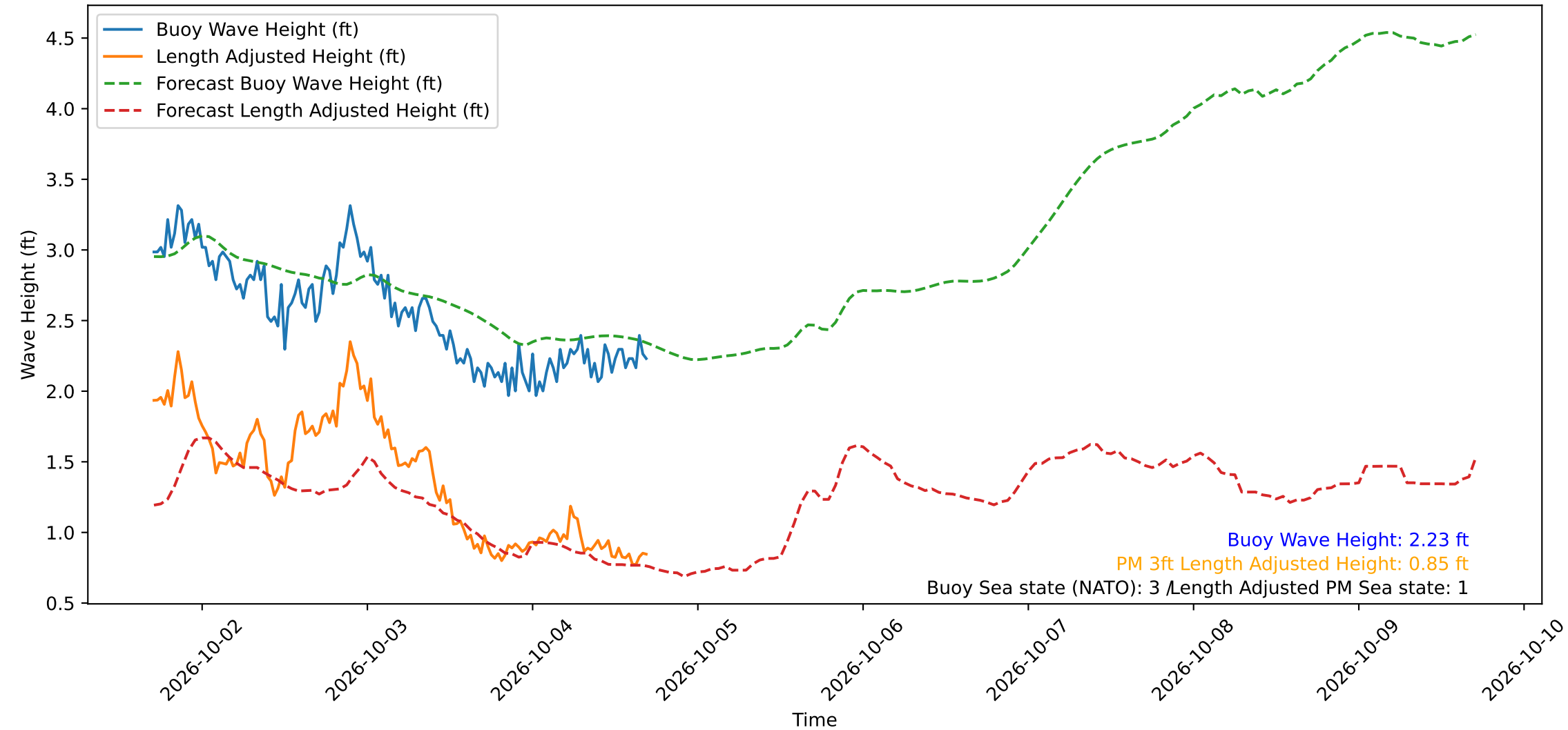
Wave Heights over Time for Oceanside Harbor at 2026-10-04 17:10:29
