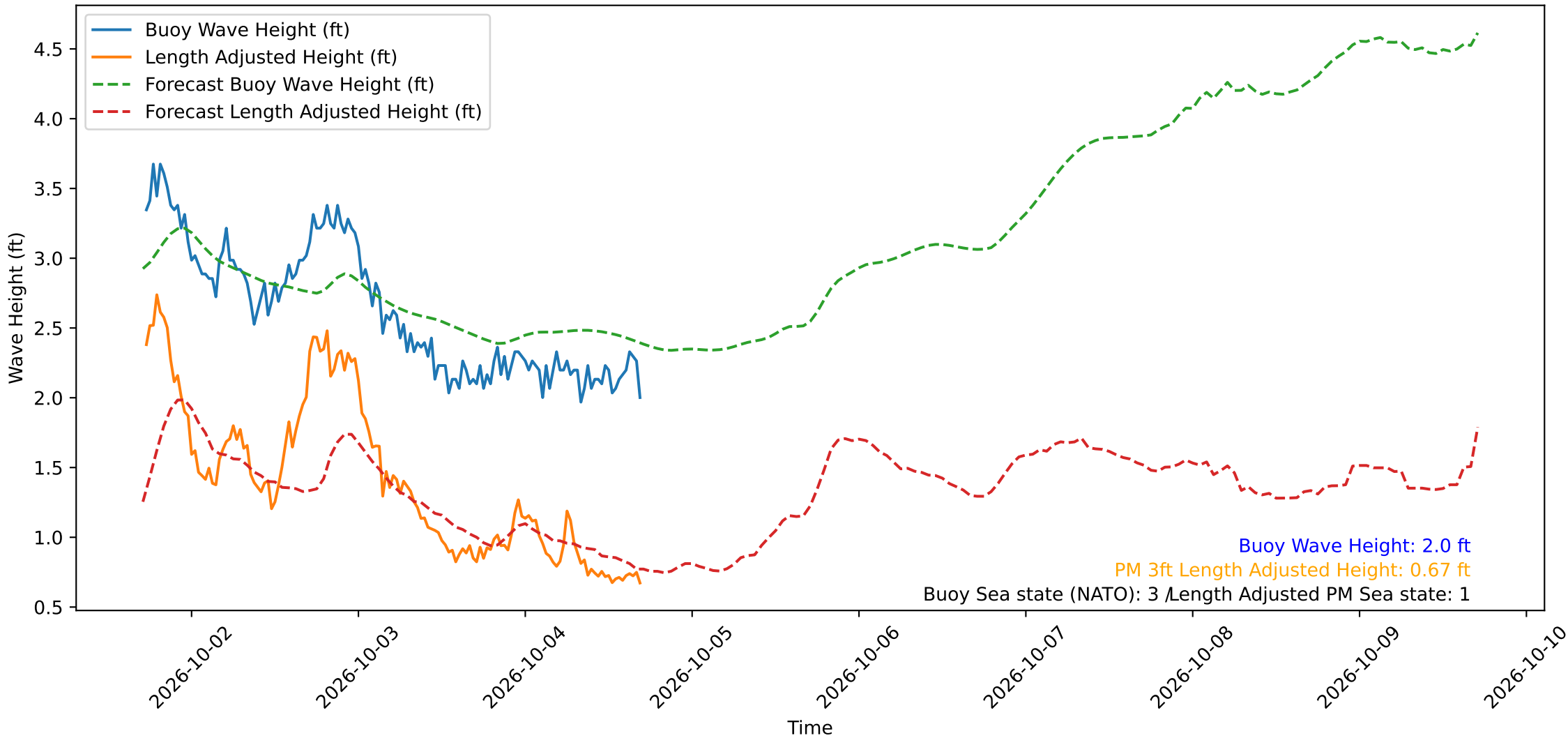
Wave Heights over Time for Green Beach at 2026-10-04 17:11:12
