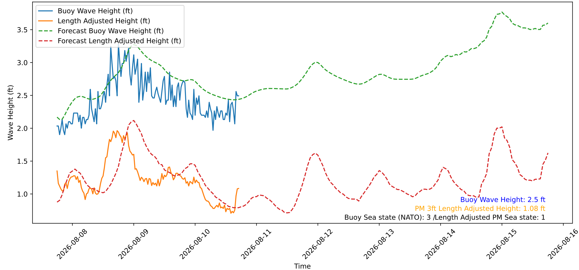
Wave Heights over Time for Oceanside Harbor at 2026-08-10 18:00:26
