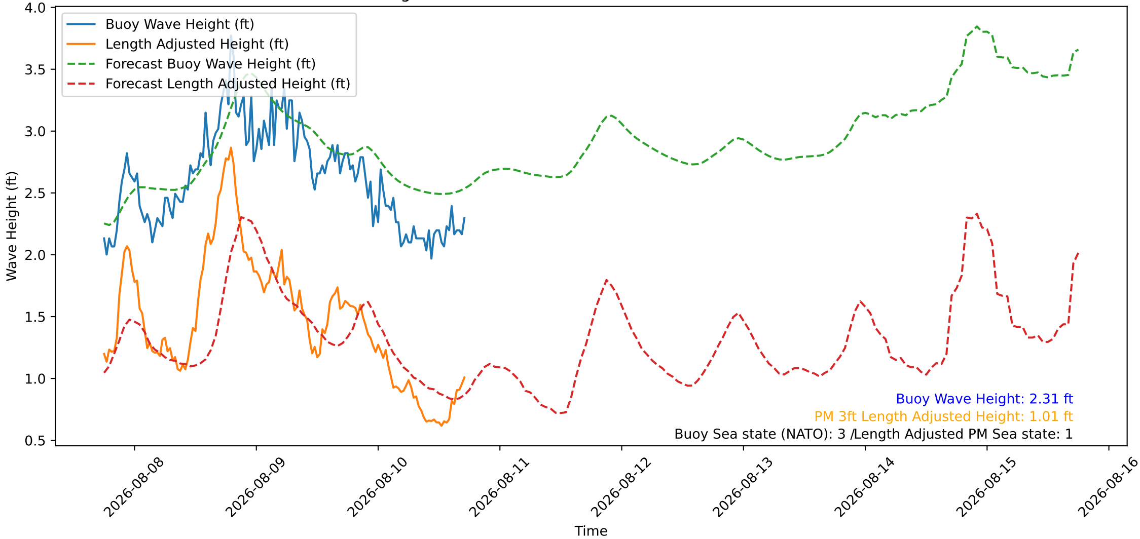
Wave Heights over Time for Green Beach at 2026-08-10 18:01:09
