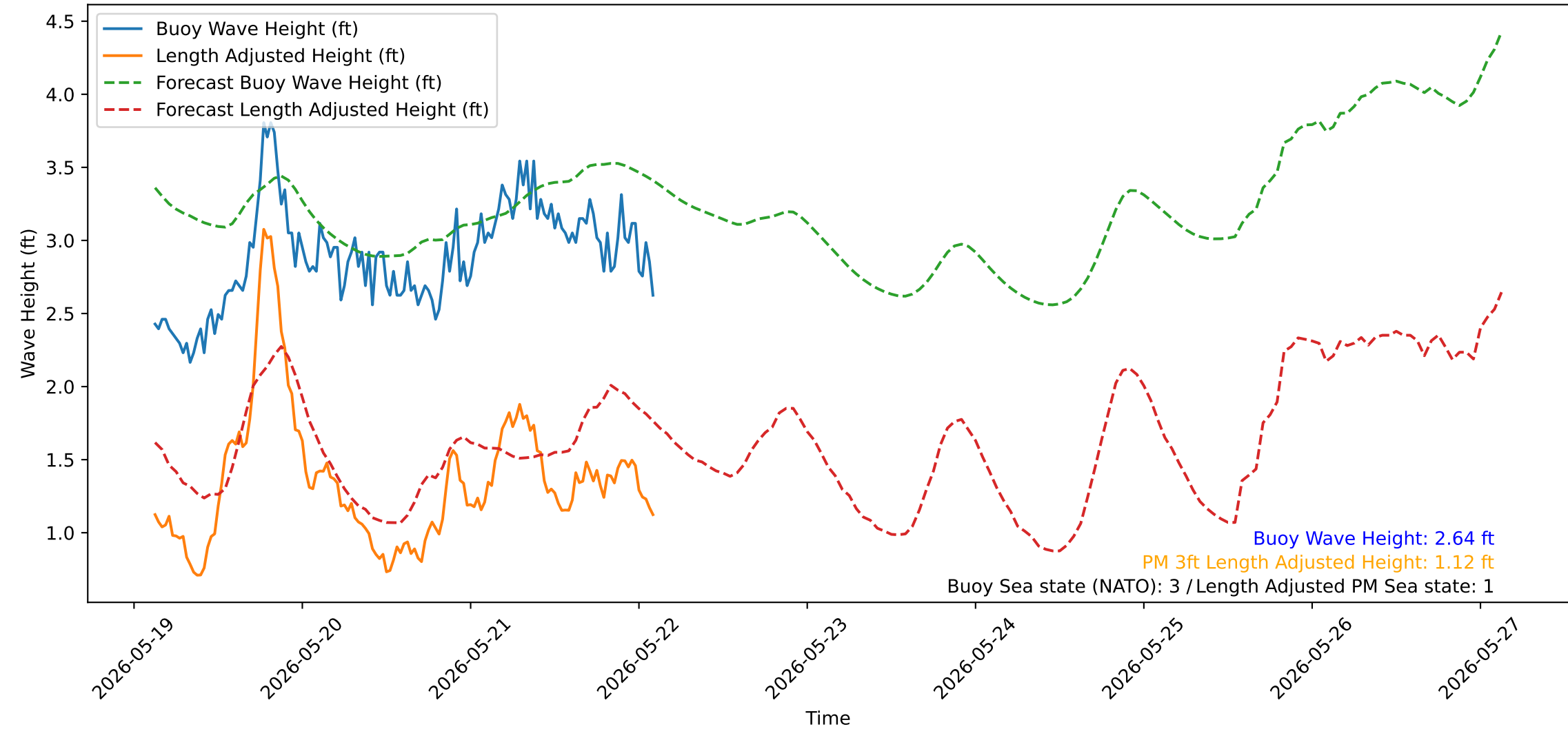
Wave Heights over Time for Green Beach at 2026-05-22 03:01:13
