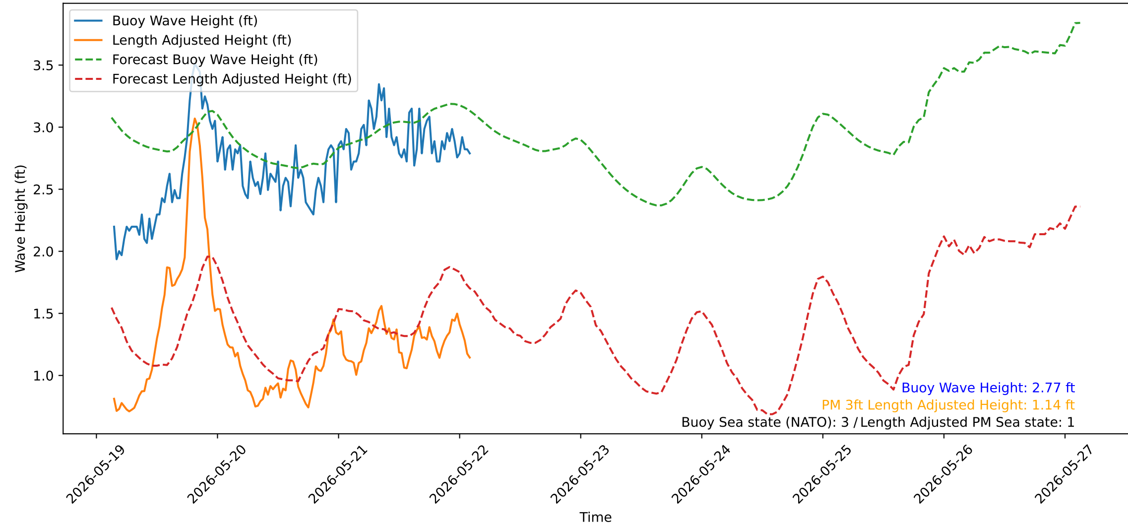
Wave Heights over Time for Red Beach at 2026-05-22 03:00:51
