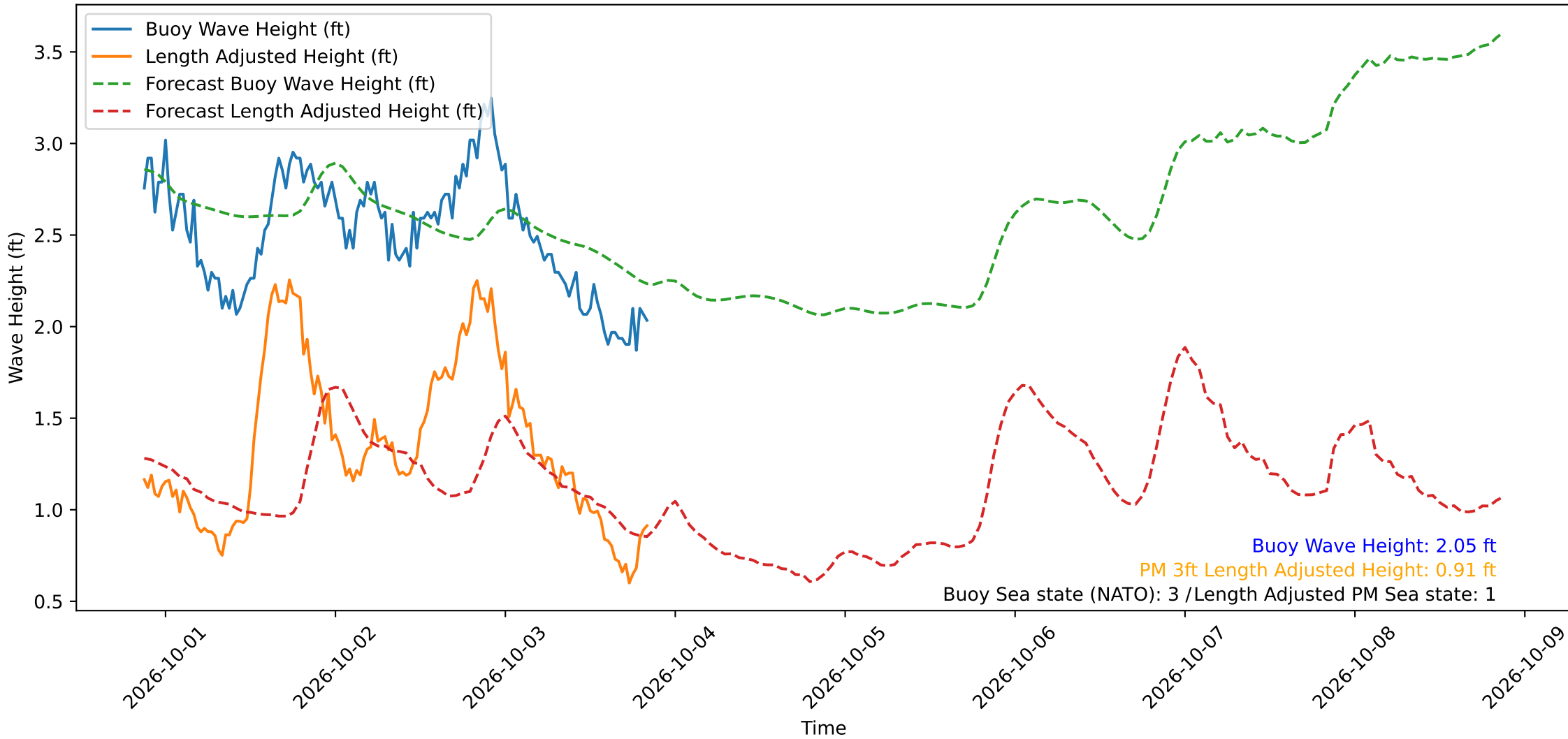
Wave Heights over Time for Red Beach at 2026-10-03 20:40:49
