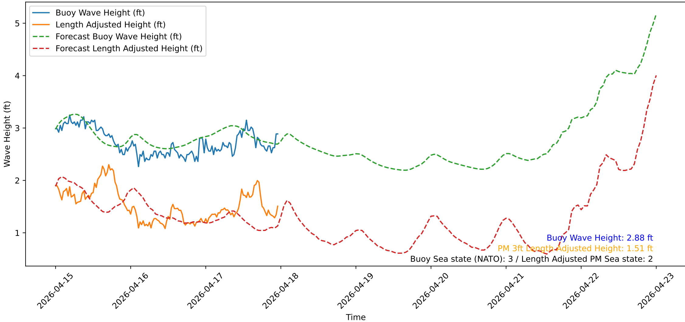
Wave Heights over Time for Red Beach at 2026-04-17 23:40:50
