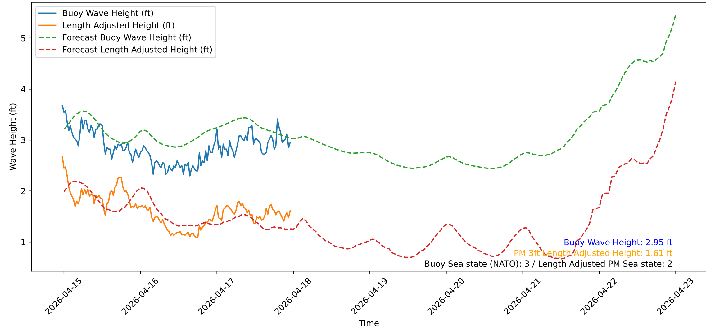
Wave Heights over Time for Oceanside Harbor at 2026-04-17 23:40:31
