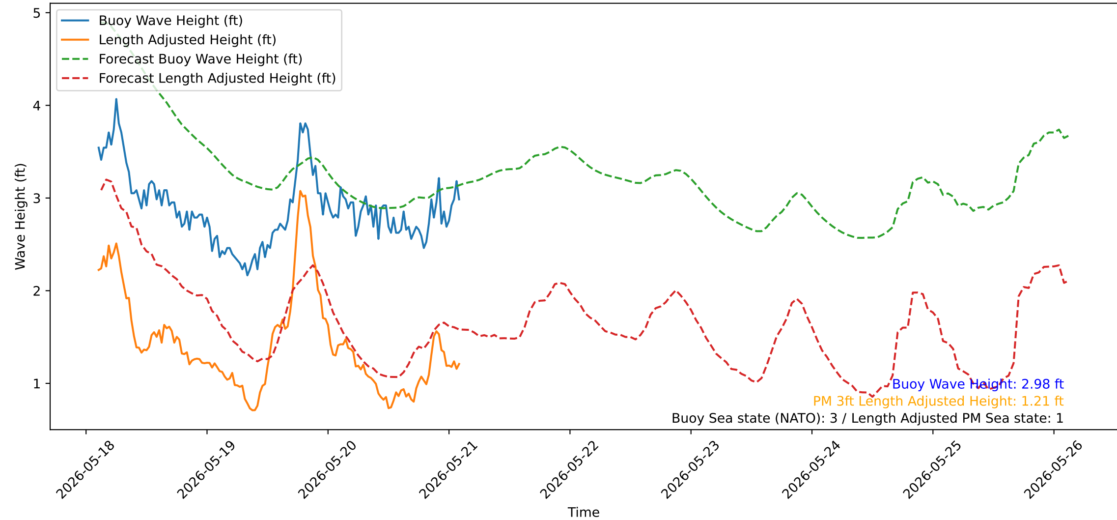
Wave Heights over Time for Green Beach at 2026-05-21 02:41:13
