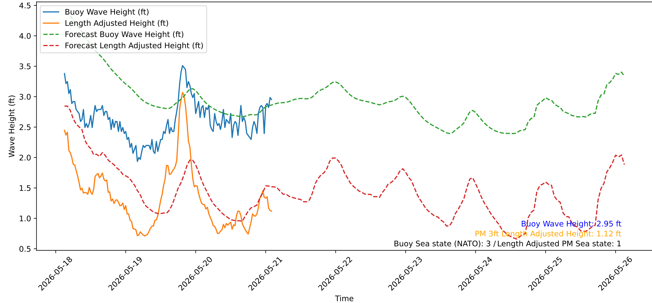
Wave Heights over Time for Red Beach at 2026-05-21 02:40:50
