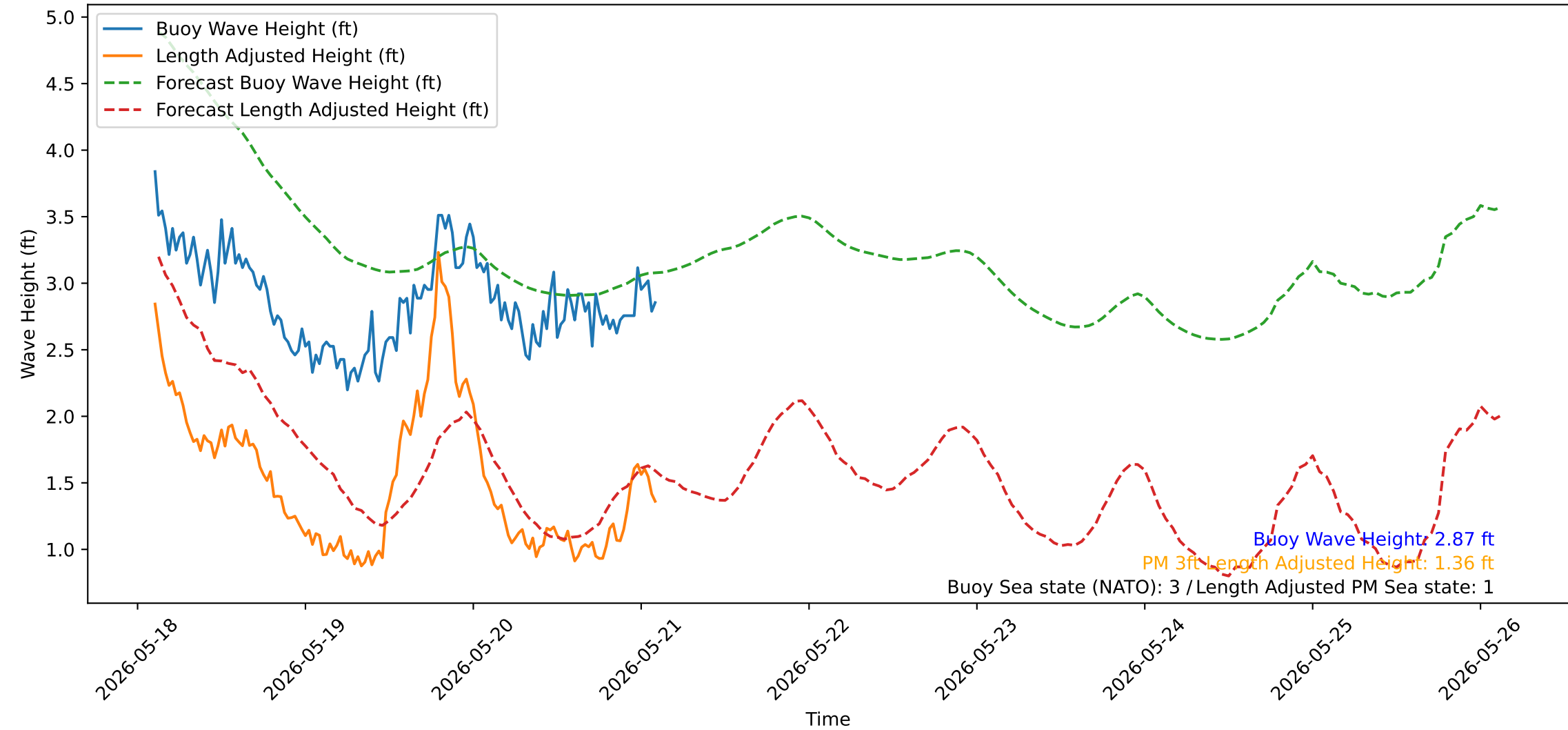
Wave Heights over Time for Oceanside Harbor at 2026-05-21 02:40:31
