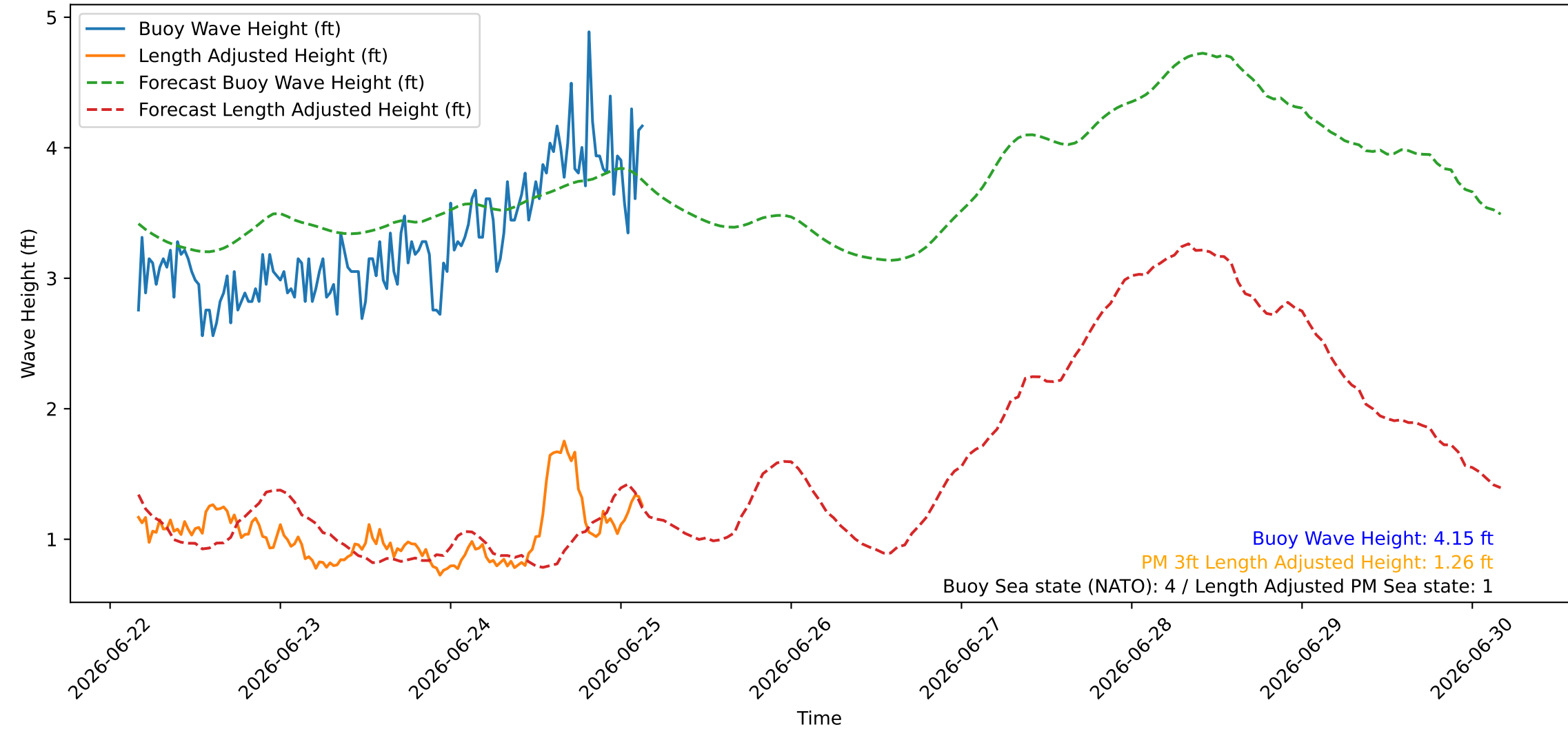
Wave Heights over Time for Oceanside Harbor at 2026-06-25 03:50:26
