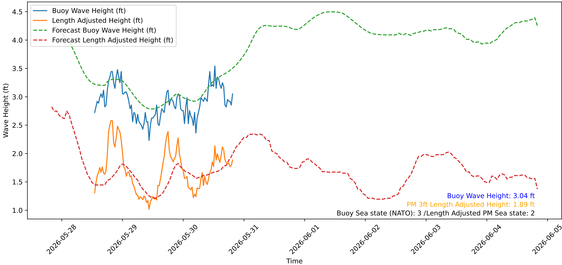
Wave Heights over Time for Oceanside Harbor at 2026-05-30 20:00:25
