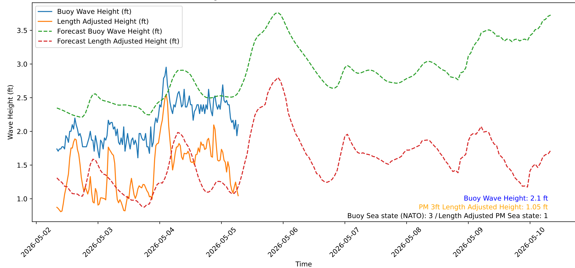
Wave Heights over Time for Red Beach at 2026-05-05 07:30:50
