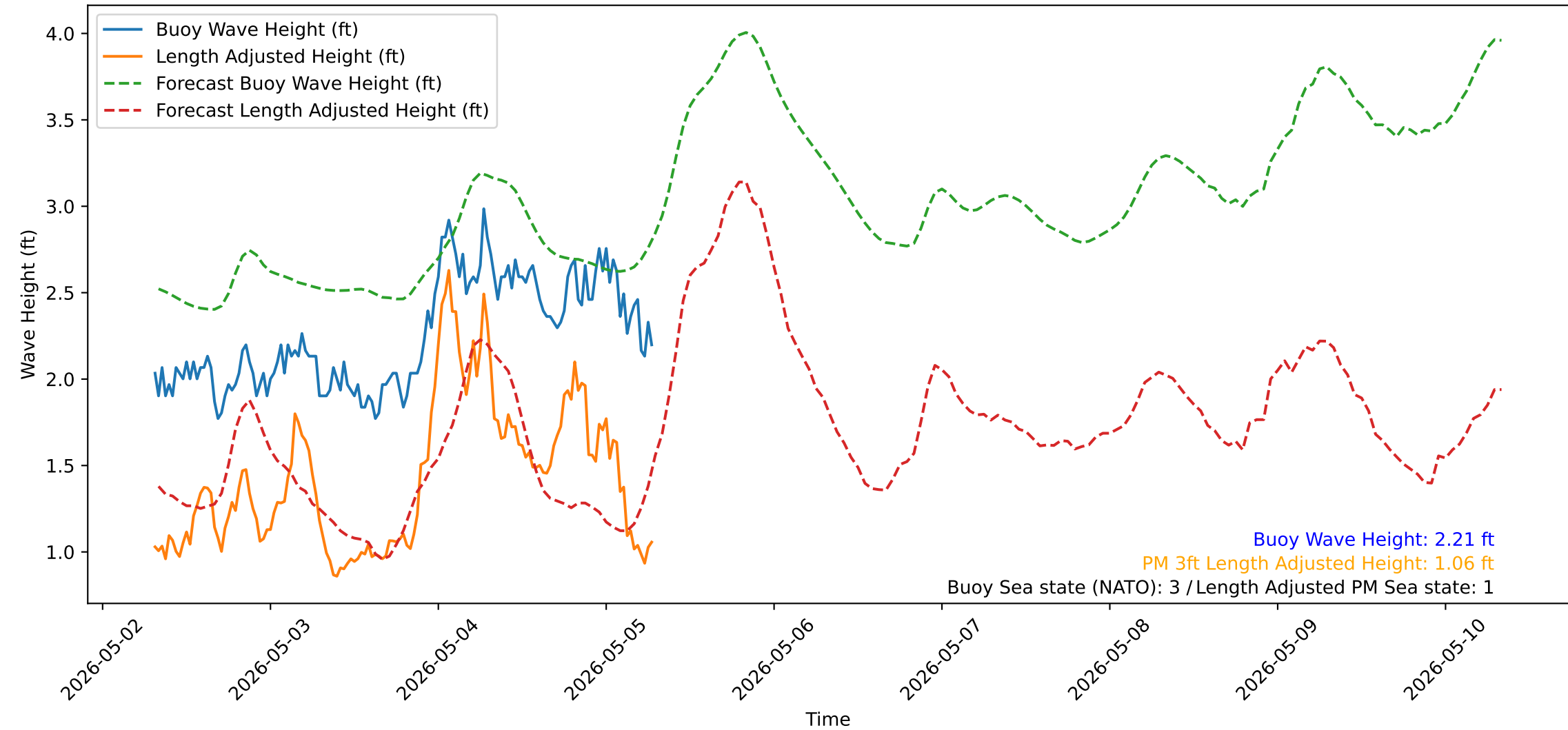
Wave Heights over Time for Green Beach at 2026-05-05 07:31:13
