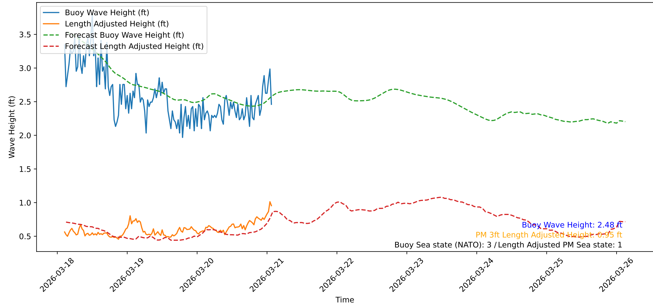
Wave Heights over Time for Oceanside Harbor at 2026-03-21 02:40:33
