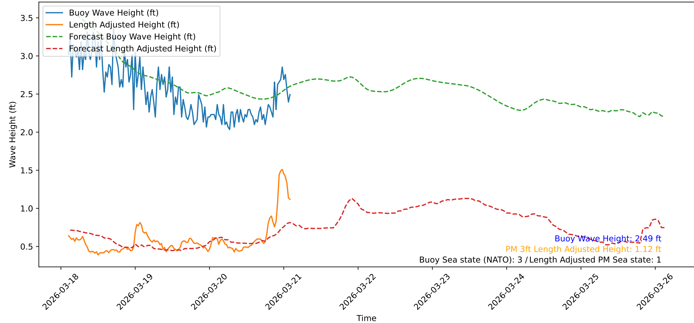
Wave Heights over Time for Green Beach at 2026-03-21 02:41:12
