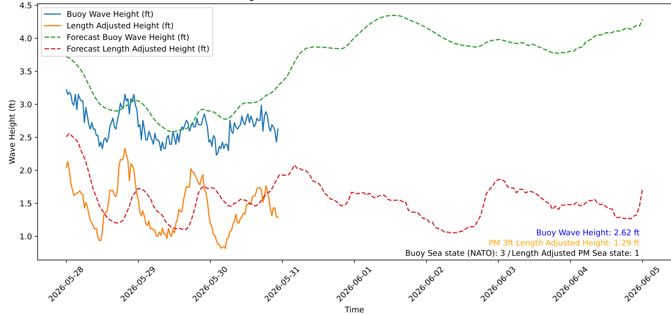
Wave Heights over Time for Red Beach at 2026-05-30 23:30:45
