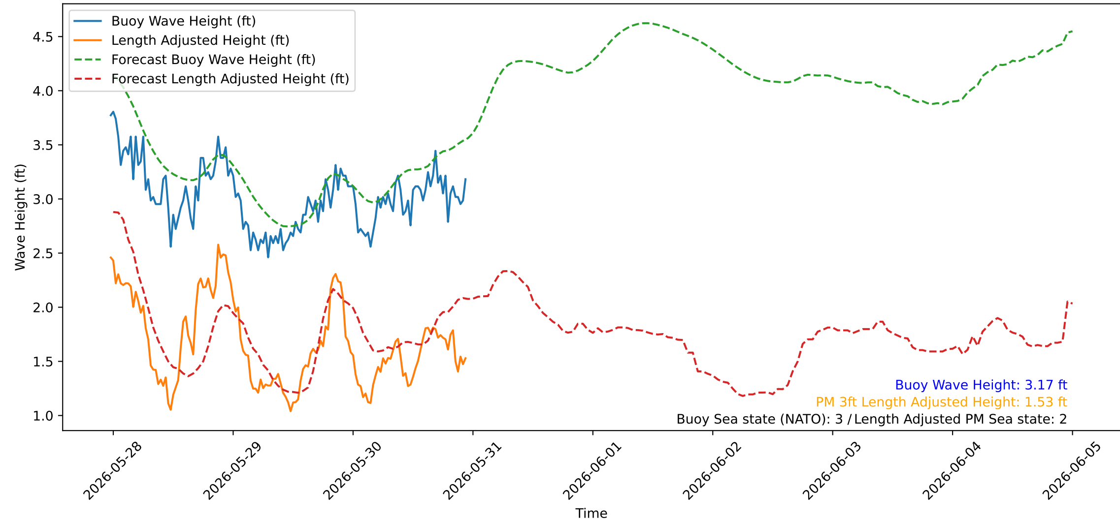
Wave Heights over Time for Green Beach at 2026-05-30 23:31:07
