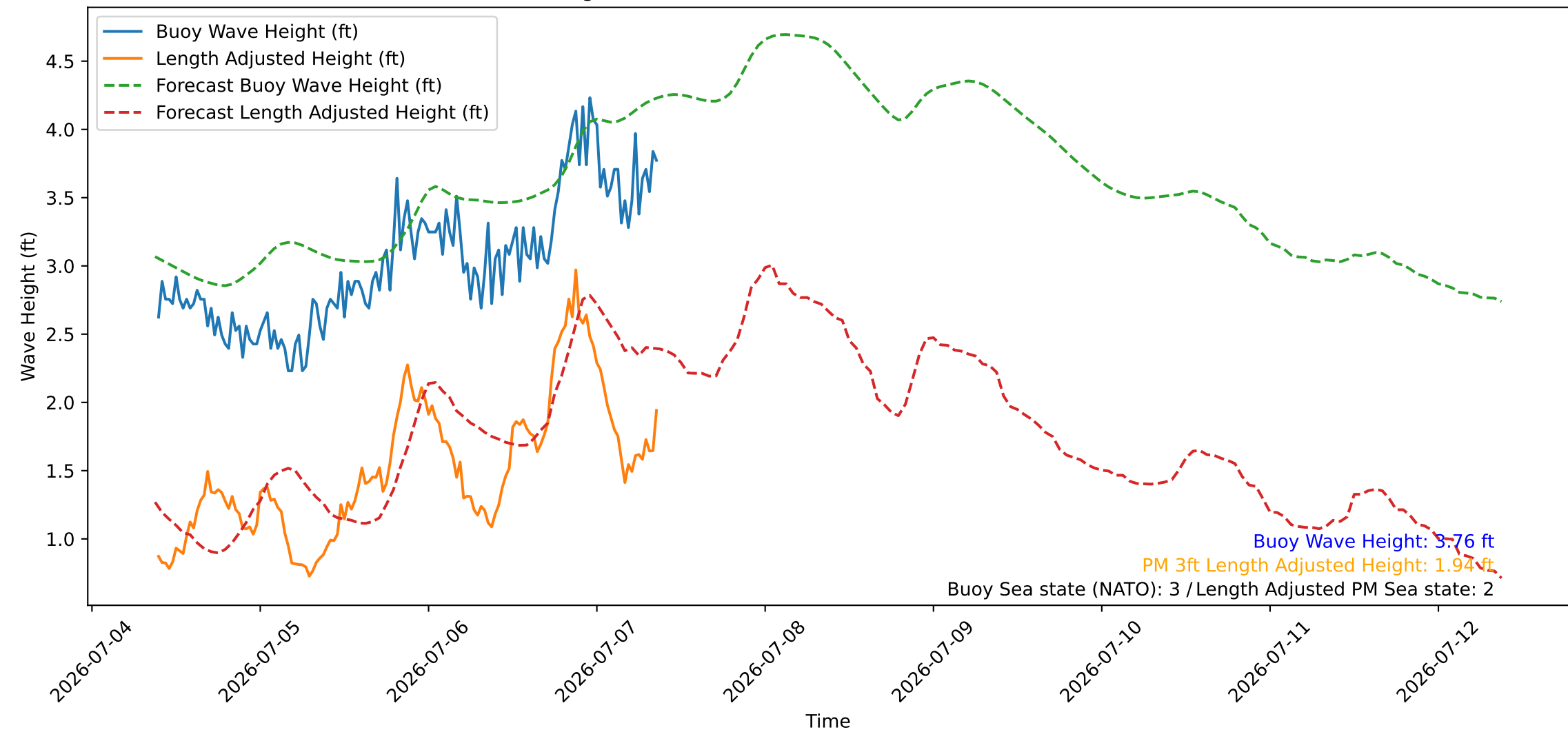
Wave Heights over Time for Red Beach at 2026-07-07 09:20:46
