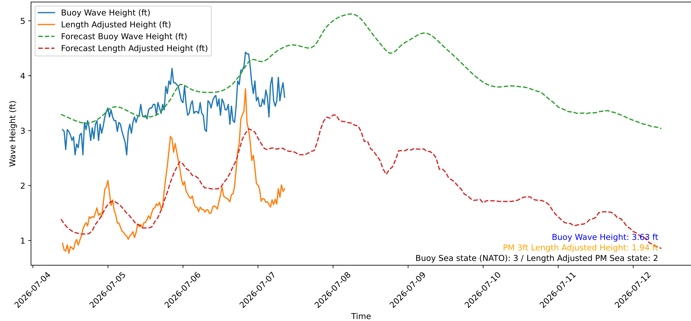
Wave Heights over Time for Green Beach at 2026-07-07 09:21:09
