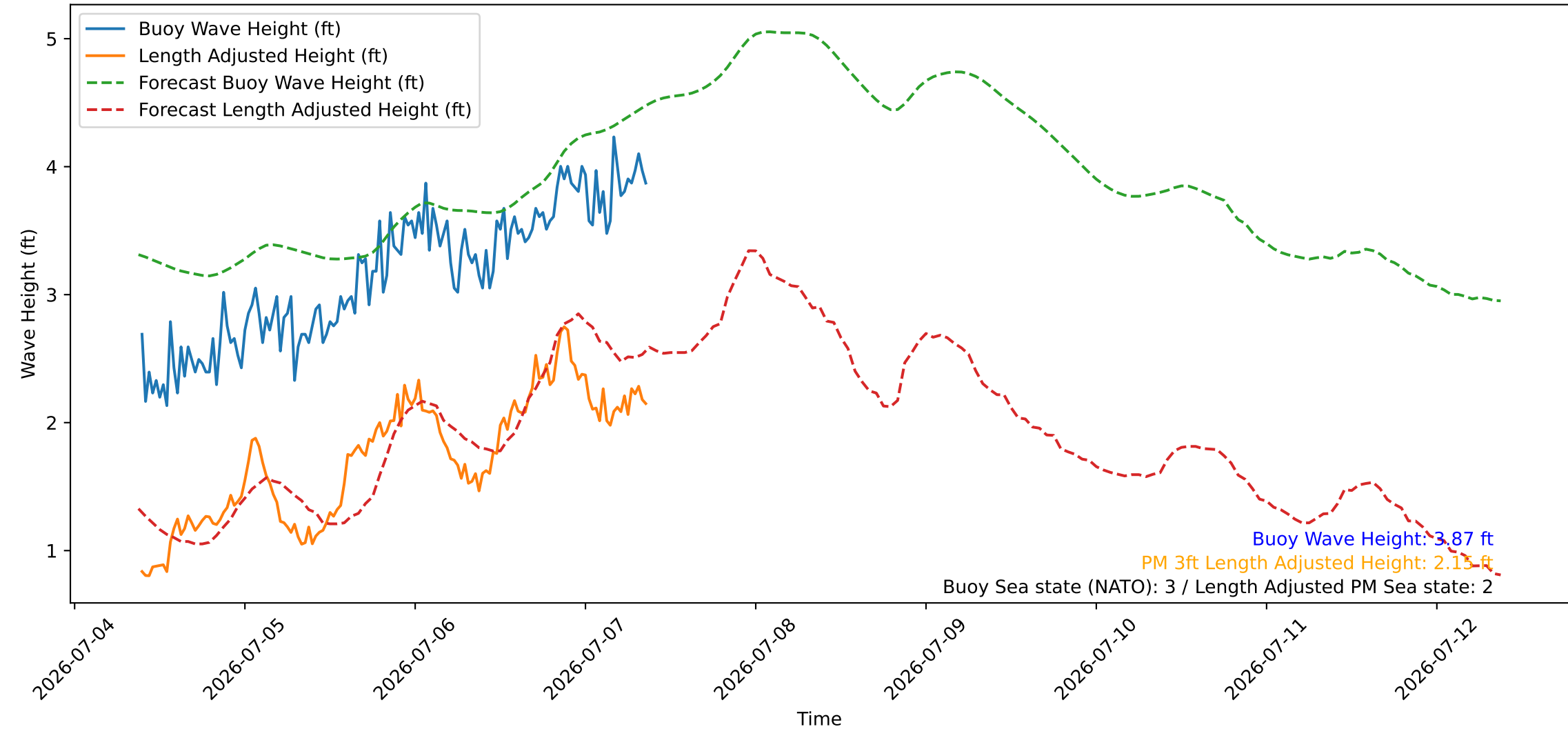
Wave Heights over Time for Oceanside Harbor at 2026-07-07 09:20:26
