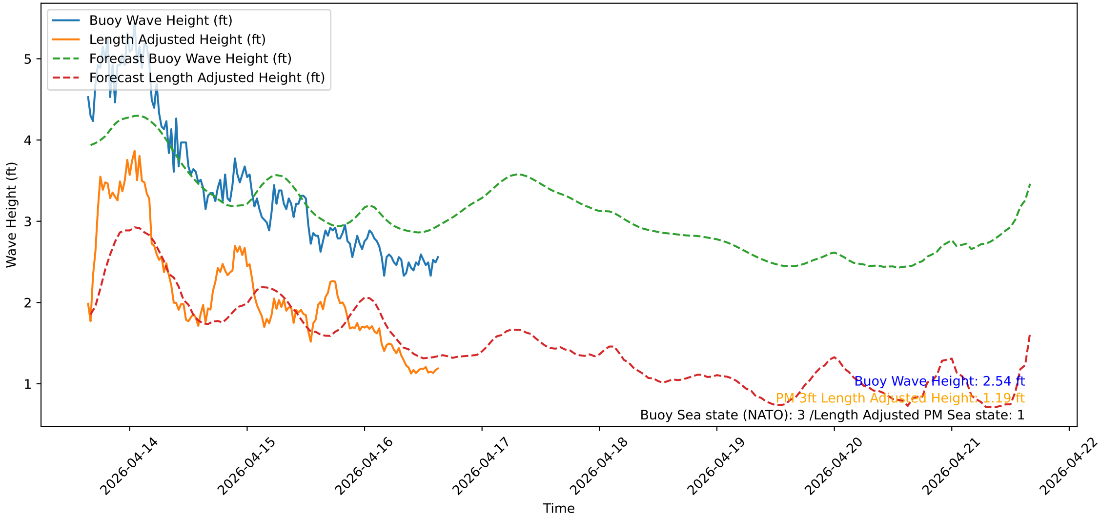
Wave Heights over Time for Oceanside Harbor at 2026-04-16 15:30:32
