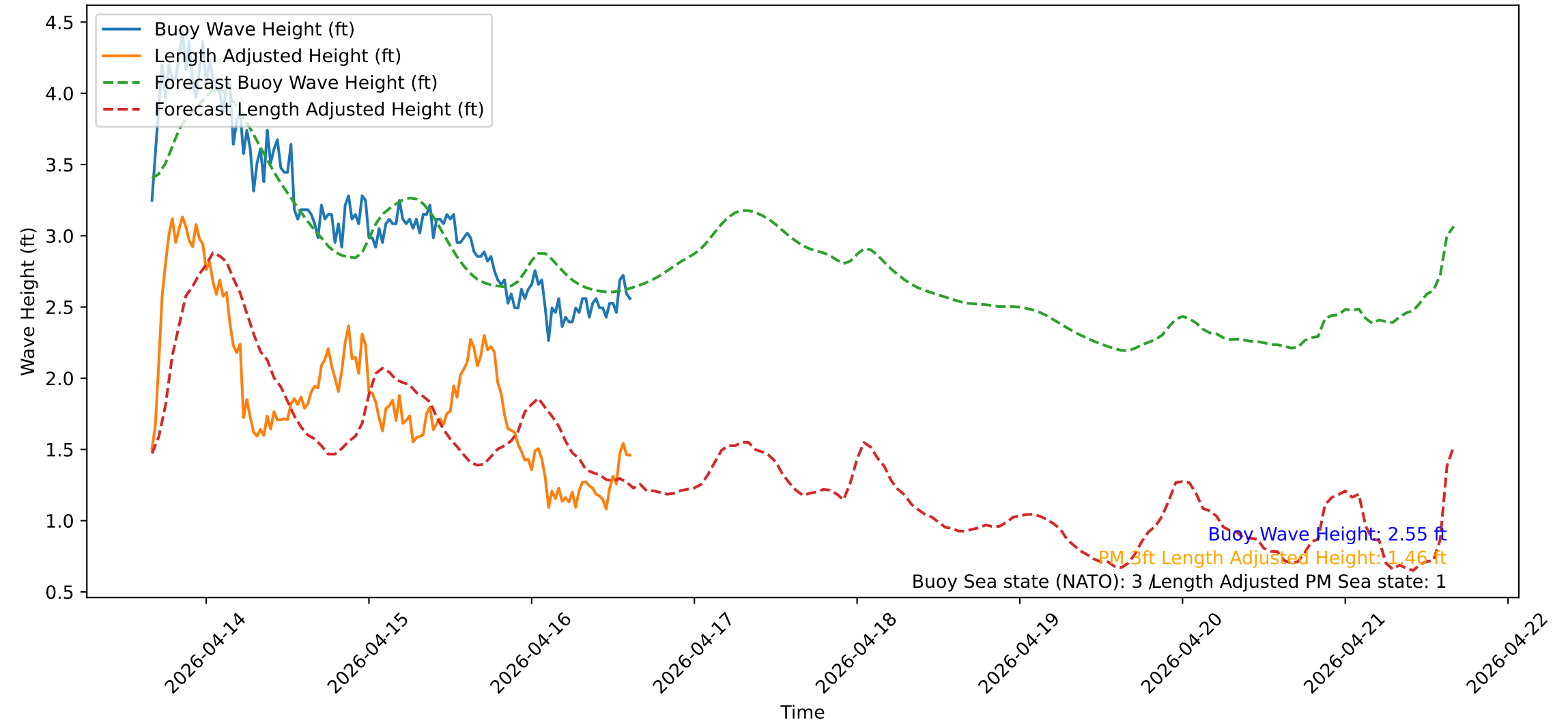
Wave Heights over Time for Red Beach at 2026-04-16 15:30:52
