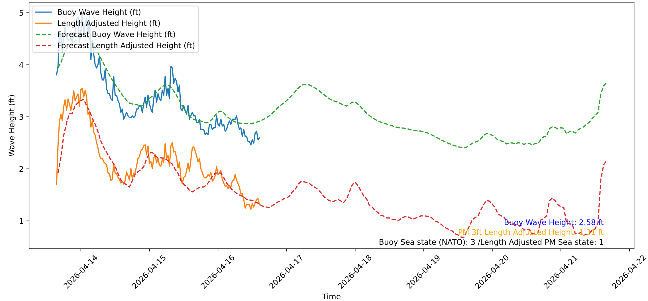
Wave Heights over Time for Green Beach at 2026-04-16 15:31:15
