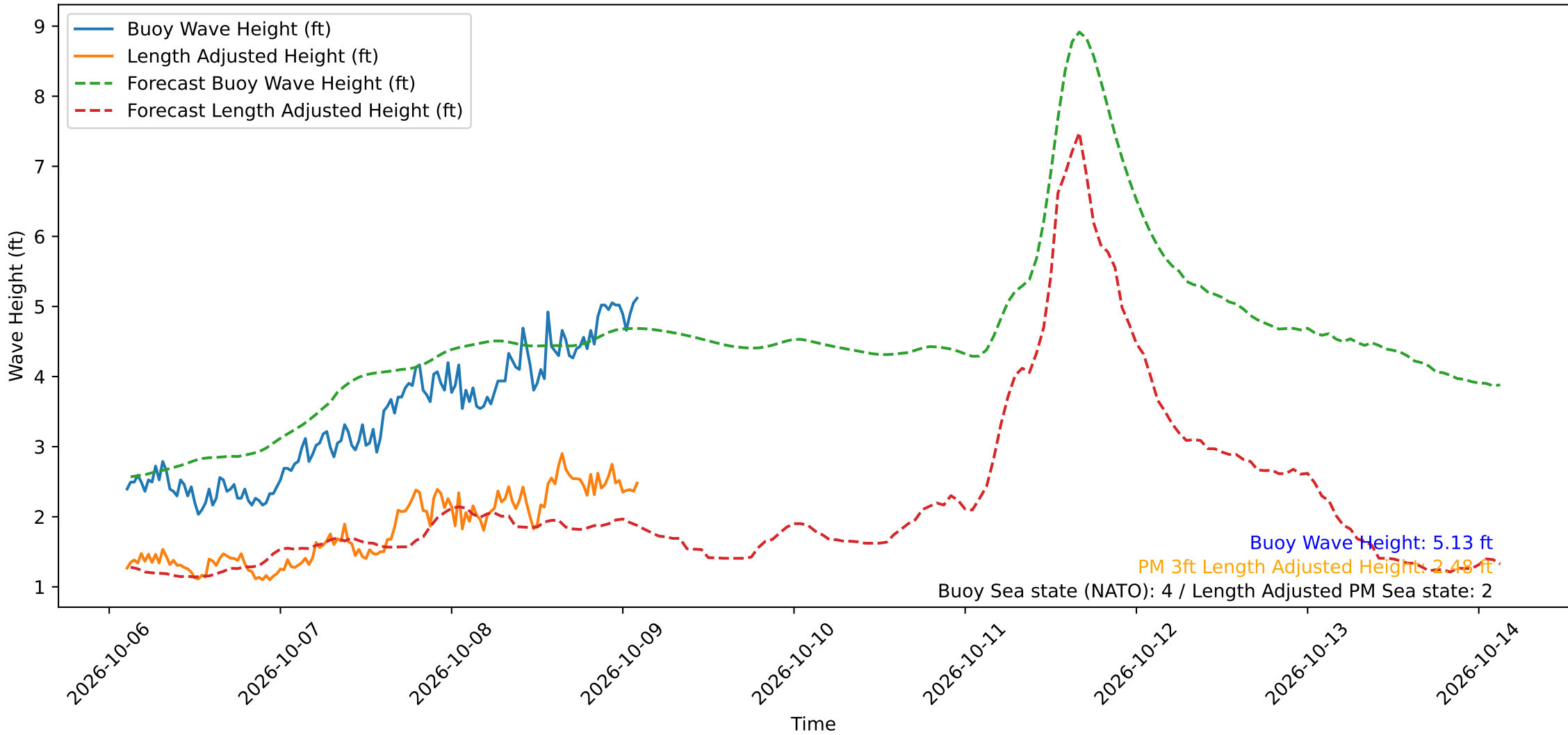
Wave Heights over Time for Oceanside Harbor at 2026-10-09 02:40:29
