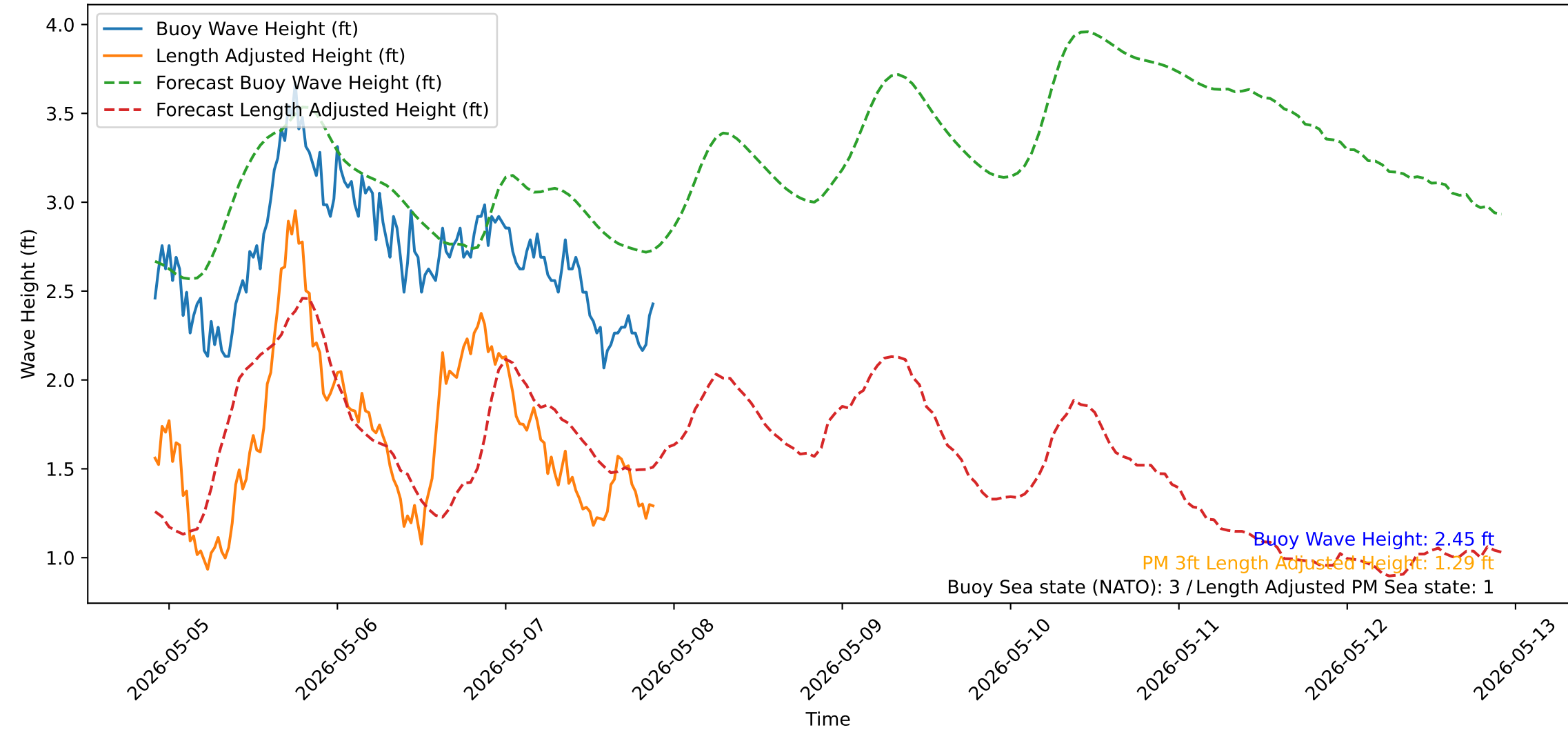
Wave Heights over Time for Green Beach at 2026-05-07 21:51:15
