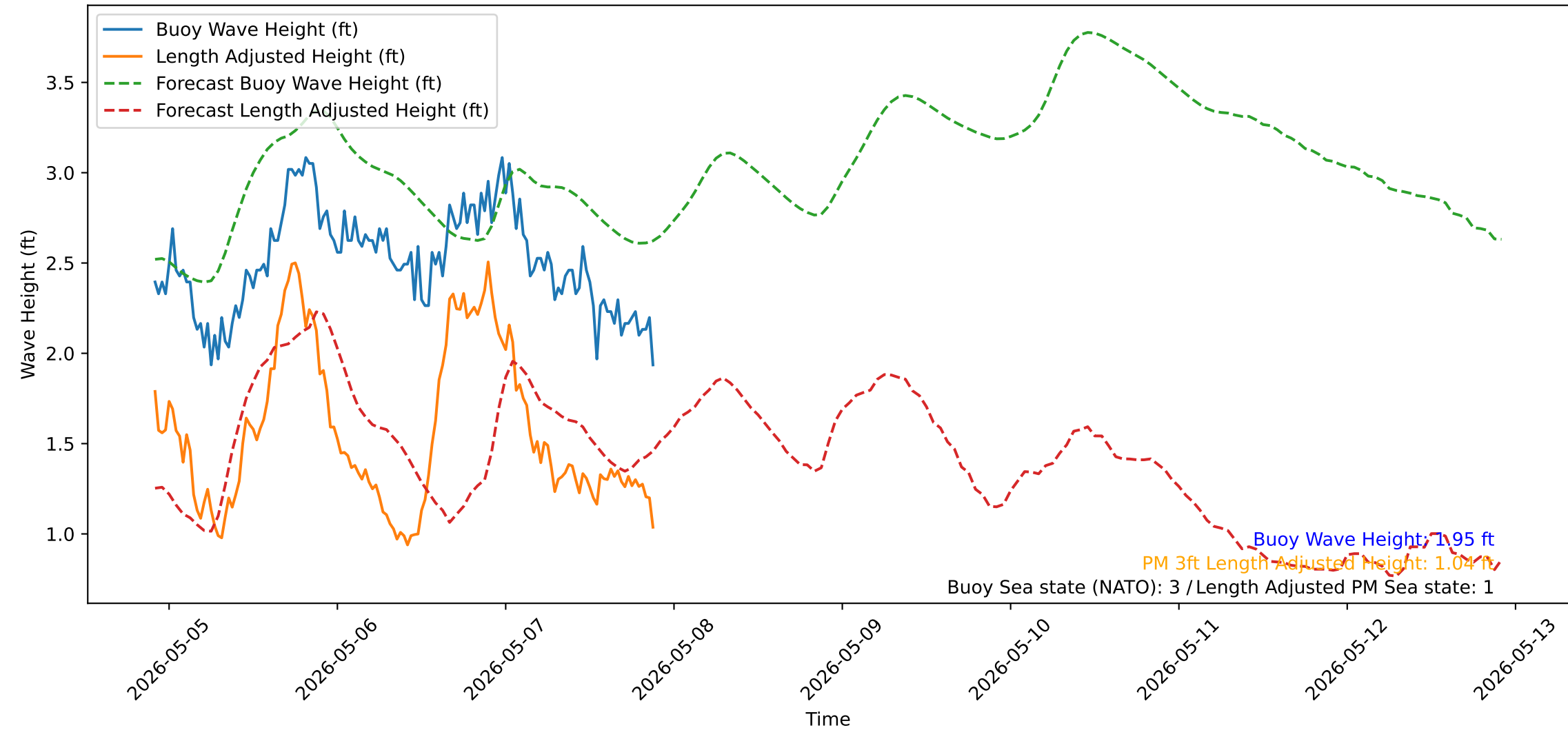
Wave Heights over Time for Red Beach at 2026-05-07 21:50:52
