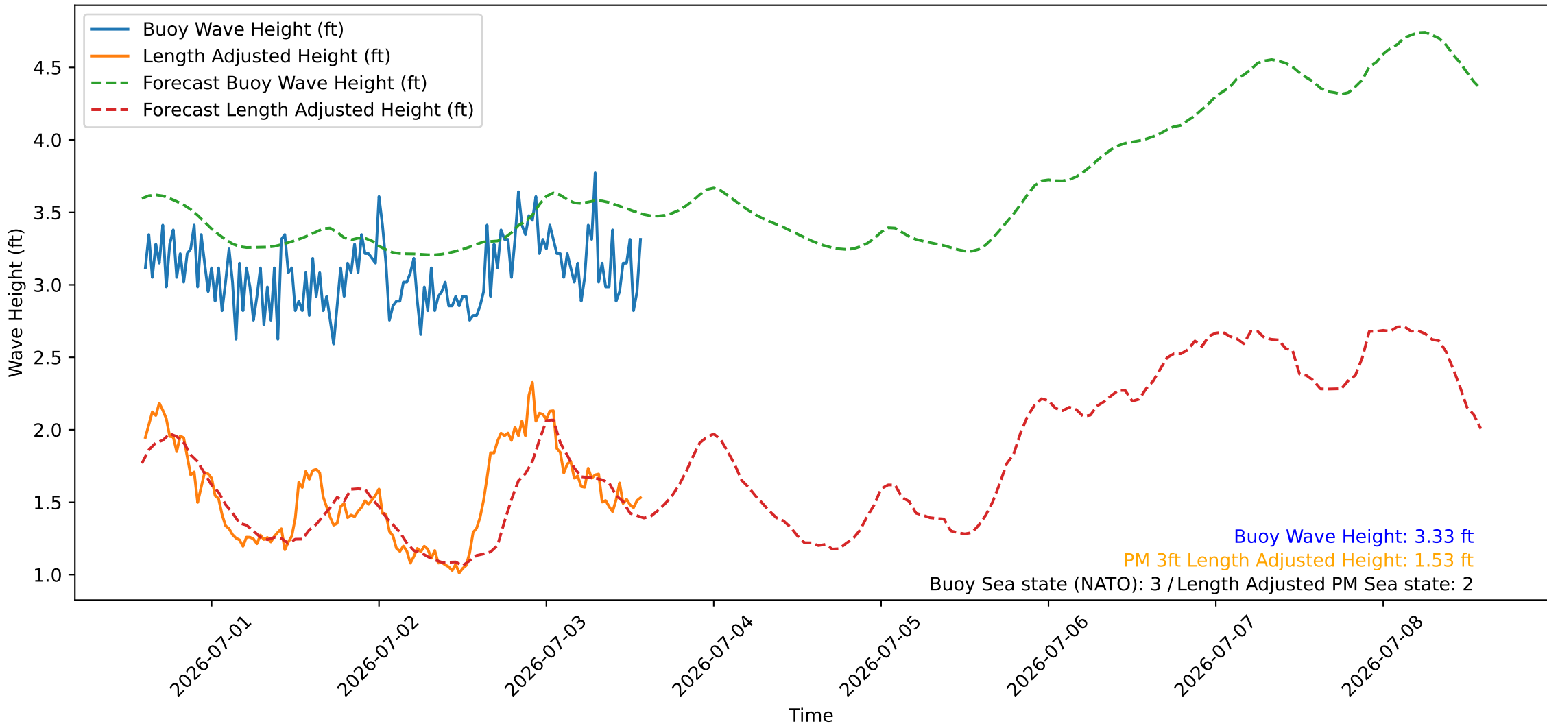
Wave Heights over Time for Oceanside Harbor at 2026-07-03 14:20:26
