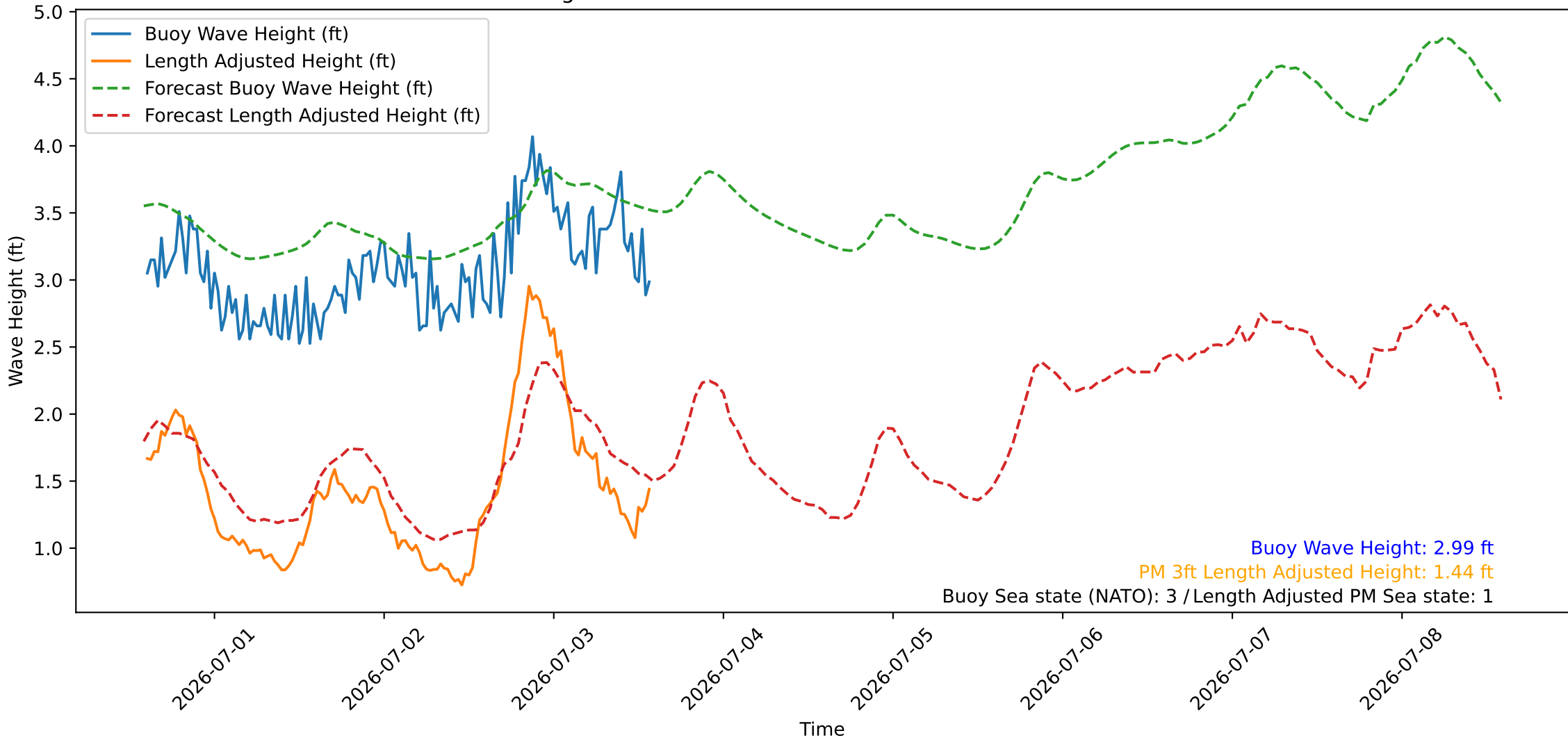
Wave Heights over Time for Green Beach at 2026-07-03 14:21:09
