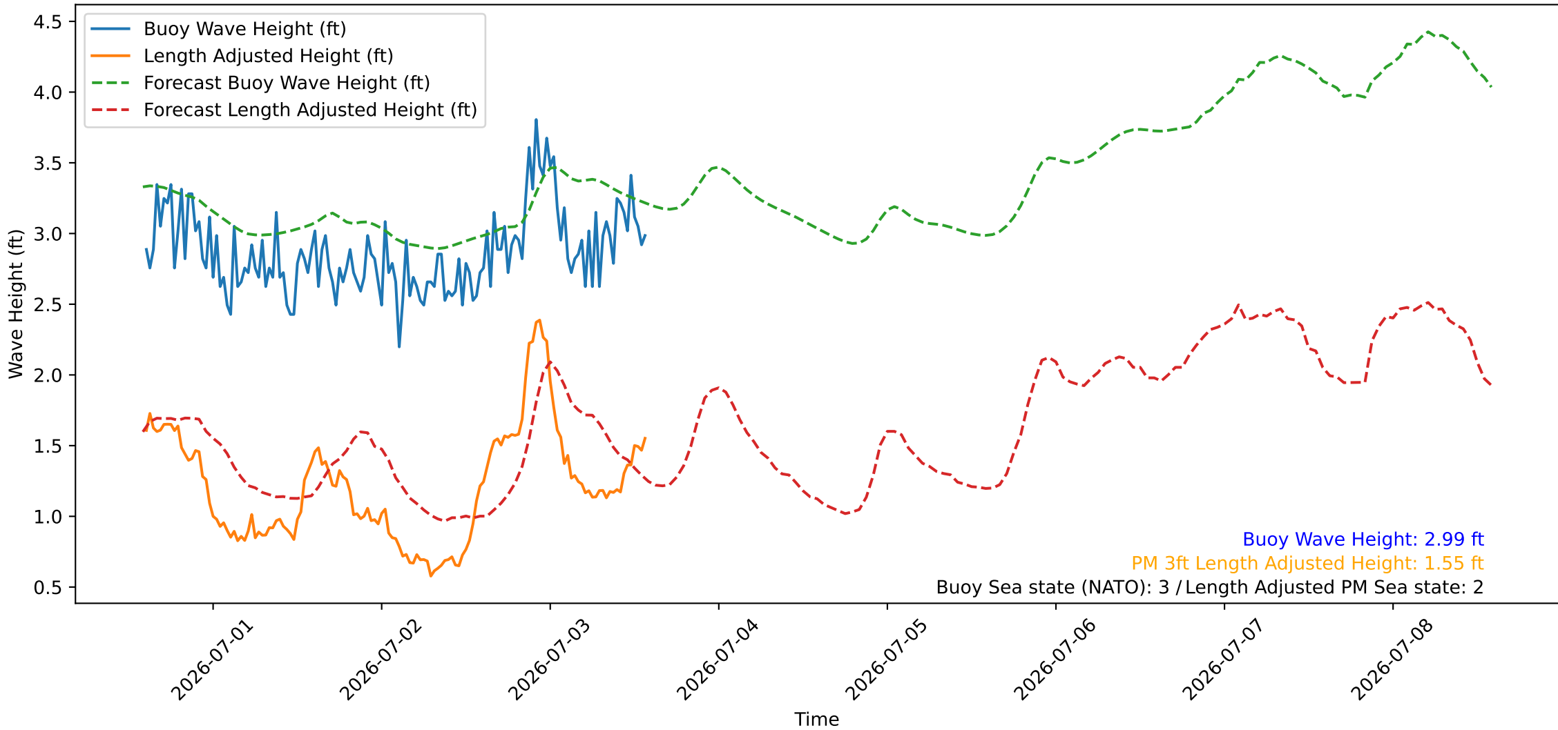
Wave Heights over Time for Red Beach at 2026-07-03 14:20:47
