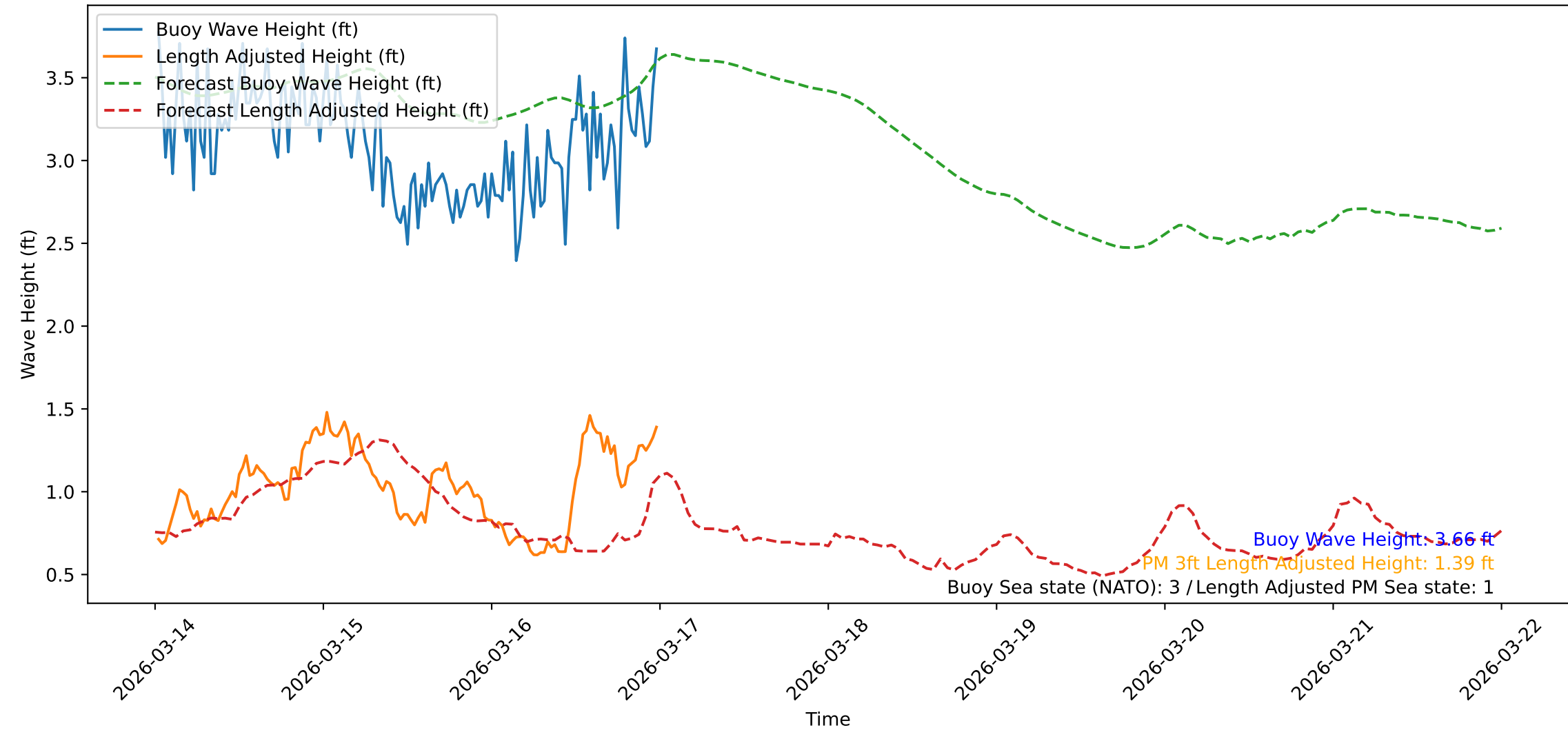
Wave Heights over Time for Oceanside Harbor at 2026-03-17 00:20:41
