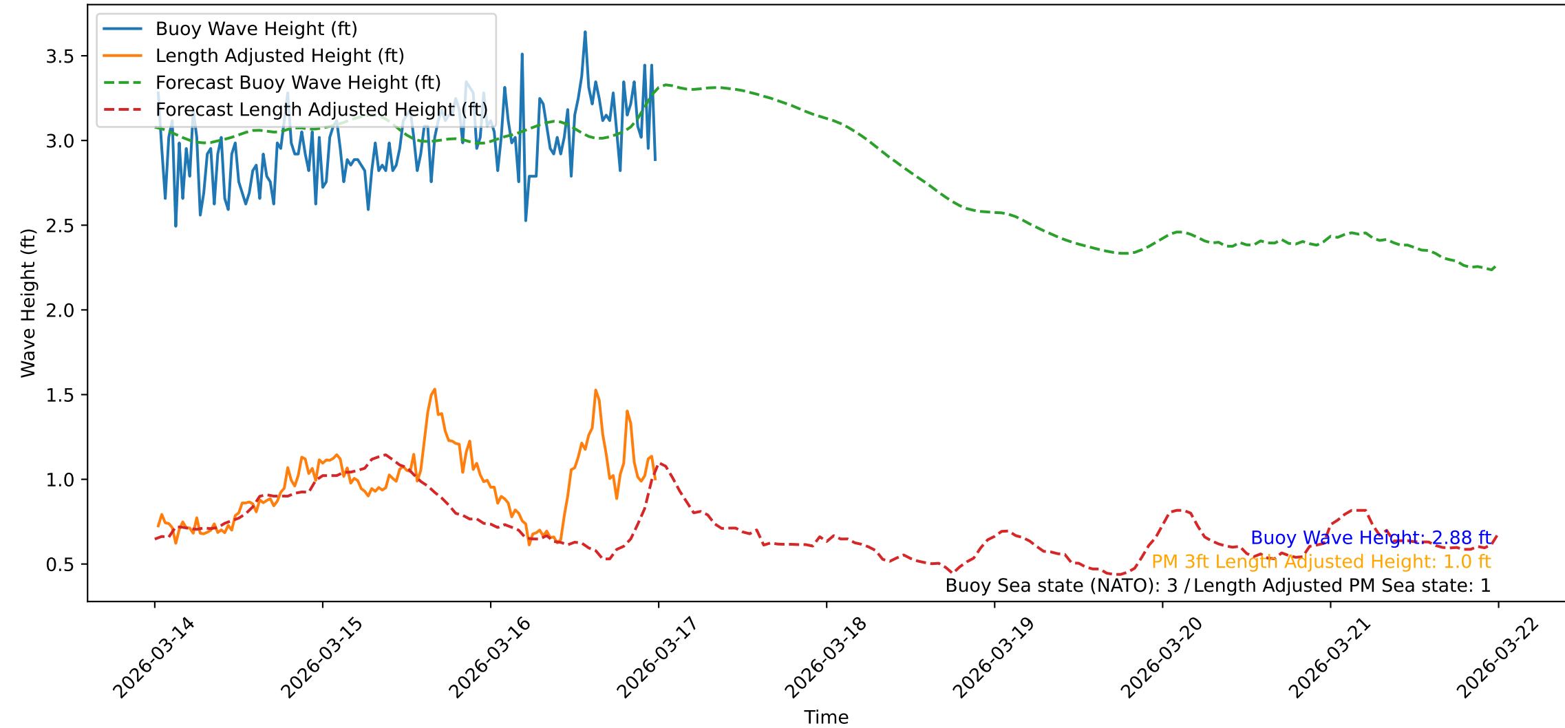
Wave Heights over Time for Red Beach at 2026-03-17 00:21:03
