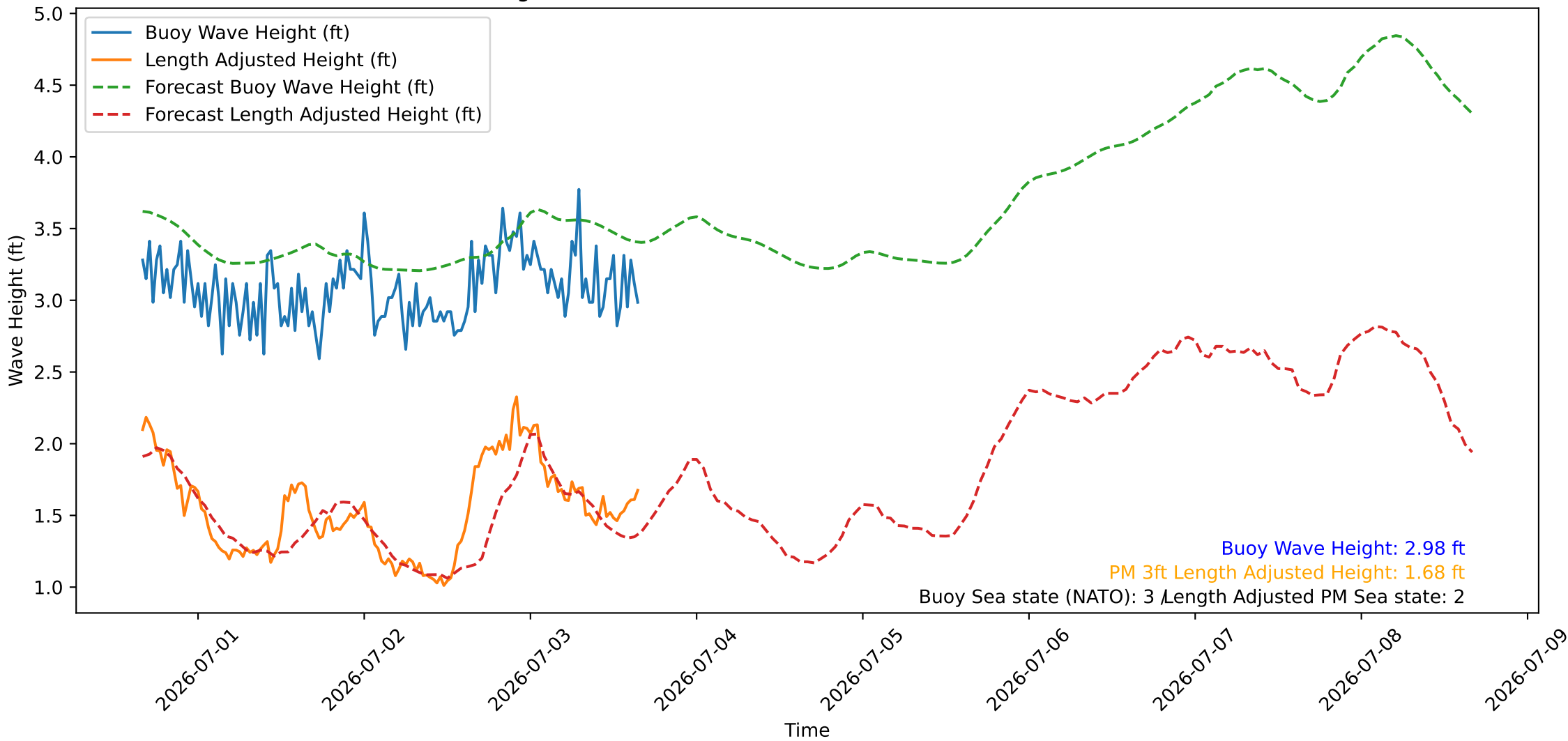
Wave Heights over Time for Oceanside Harbor at 2026-07-03 16:00:26
