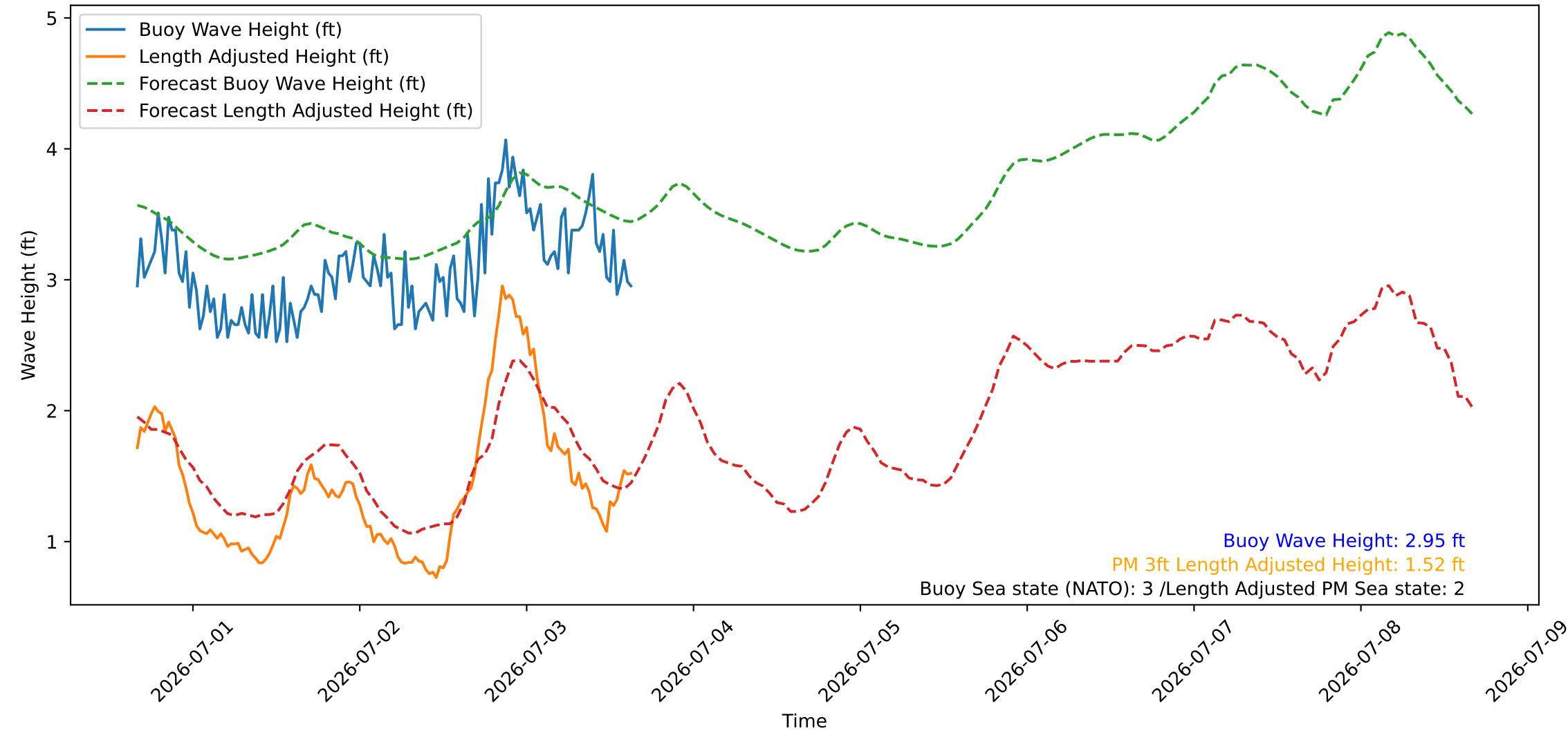
Wave Heights over Time for Green Beach at 2026-07-03 16:01:07
