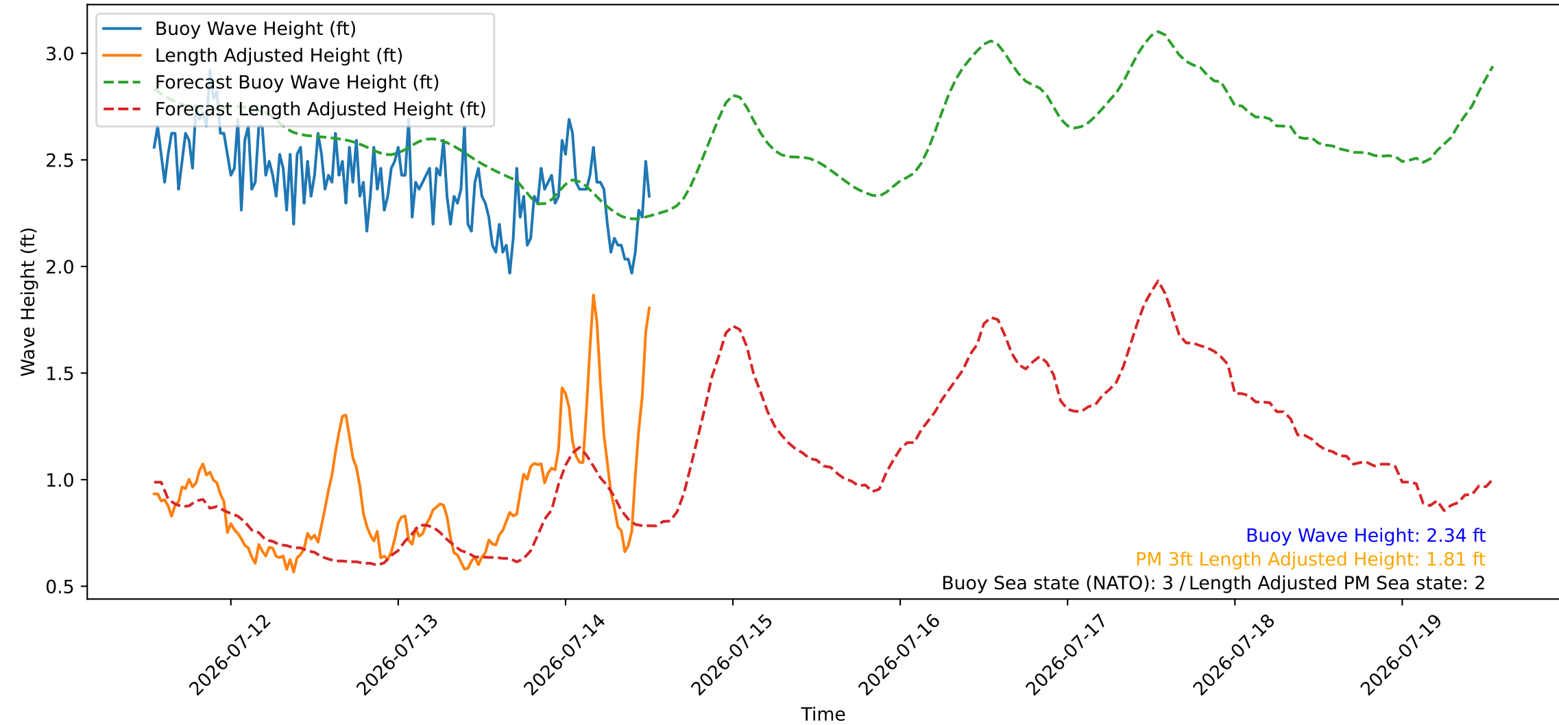
Wave Heights over Time for Red Beach at 2026-07-14 12:40:47
