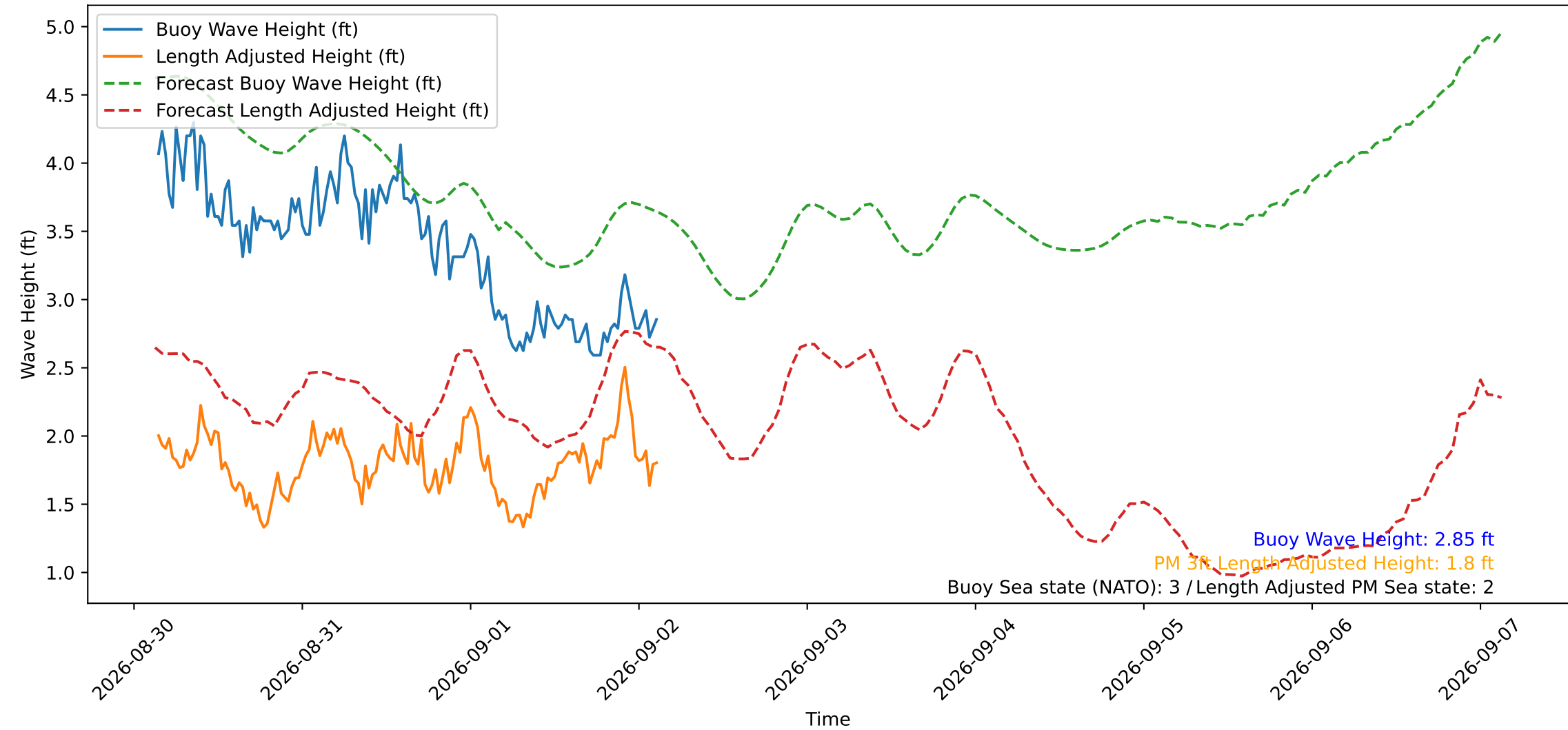
Wave Heights over Time for Red Beach at 2026-09-02 03:10:51
