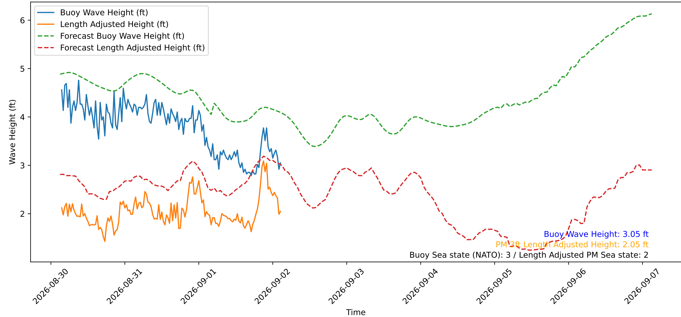
Wave Heights over Time for Green Beach at 2026-09-02 03:11:15
