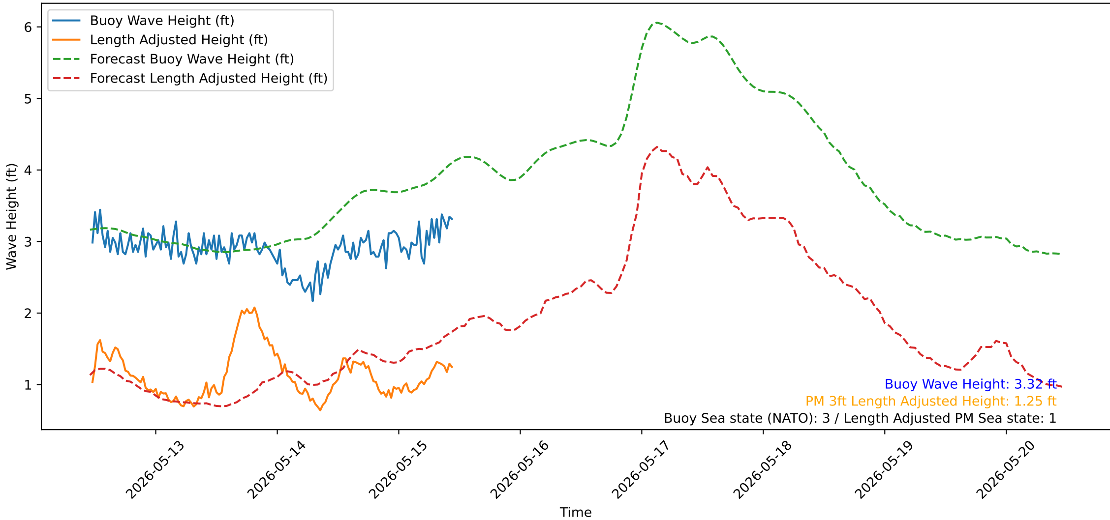
Wave Heights over Time for Oceanside Harbor at 2026-05-15 11:20:32
