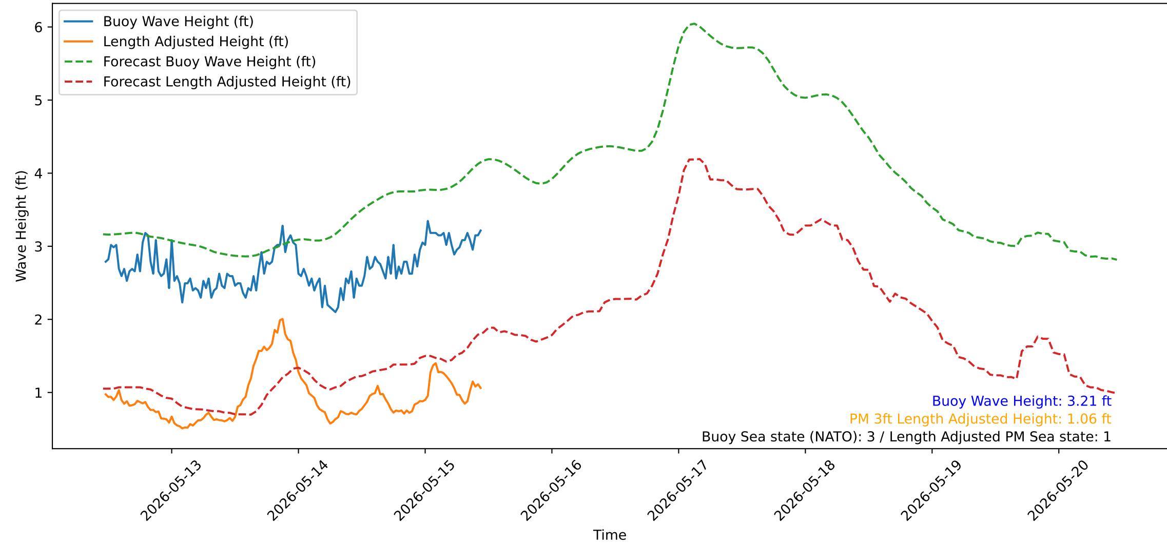
Wave Heights over Time for Green Beach at 2026-05-15 11:21:15
