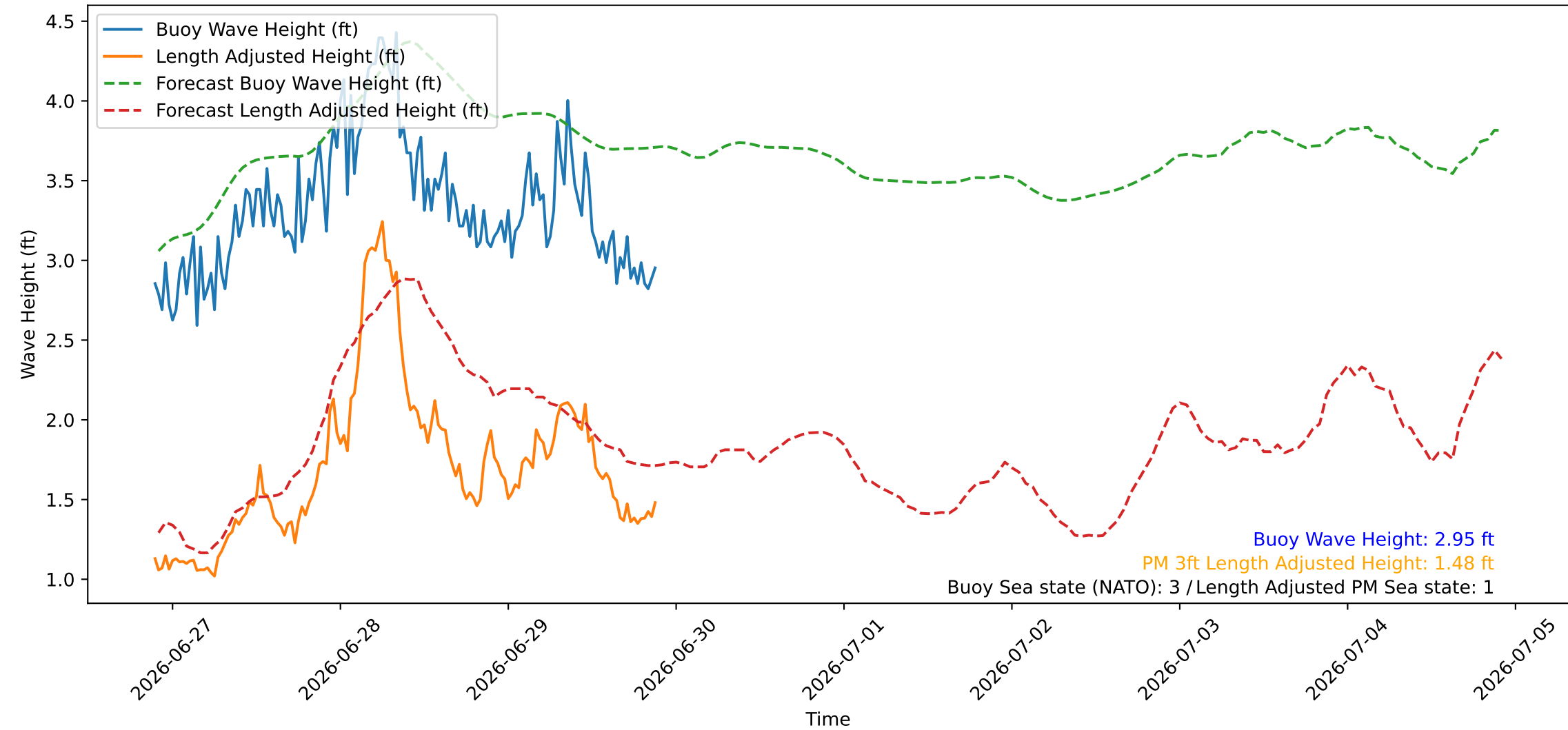
Wave Heights over Time for Oceanside Harbor at 2026-06-29 21:40:26
