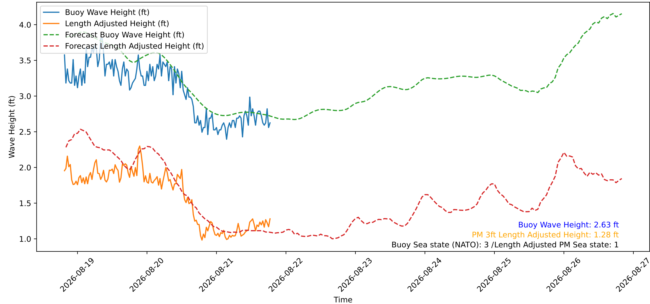
Wave Heights over Time for Oceanside Harbor at 2026-08-21 19:40:26
