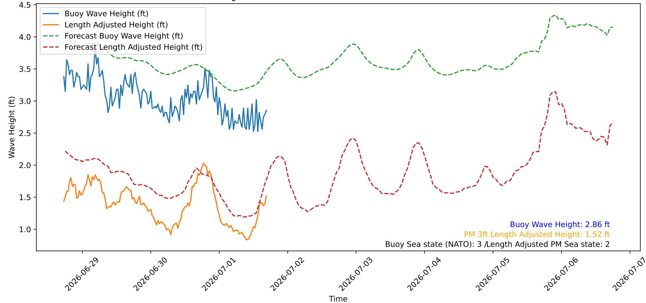
Wave Heights over Time for Green Beach at 2026-07-01 17:31:07
