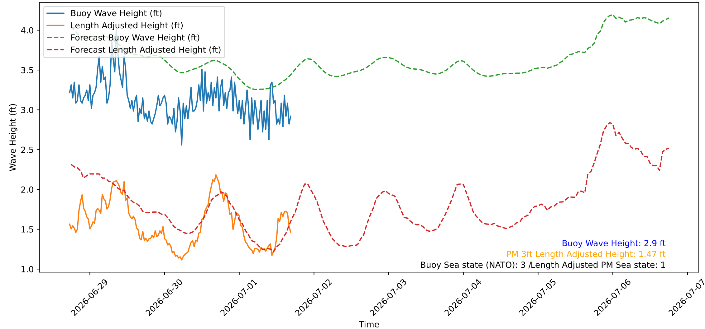
Wave Heights over Time for Oceanside Harbor at 2026-07-01 17:30:27
