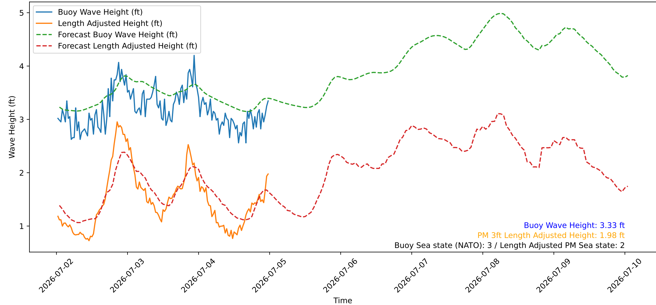
Wave Heights over Time for Green Beach at 2026-07-05 00:31:08
