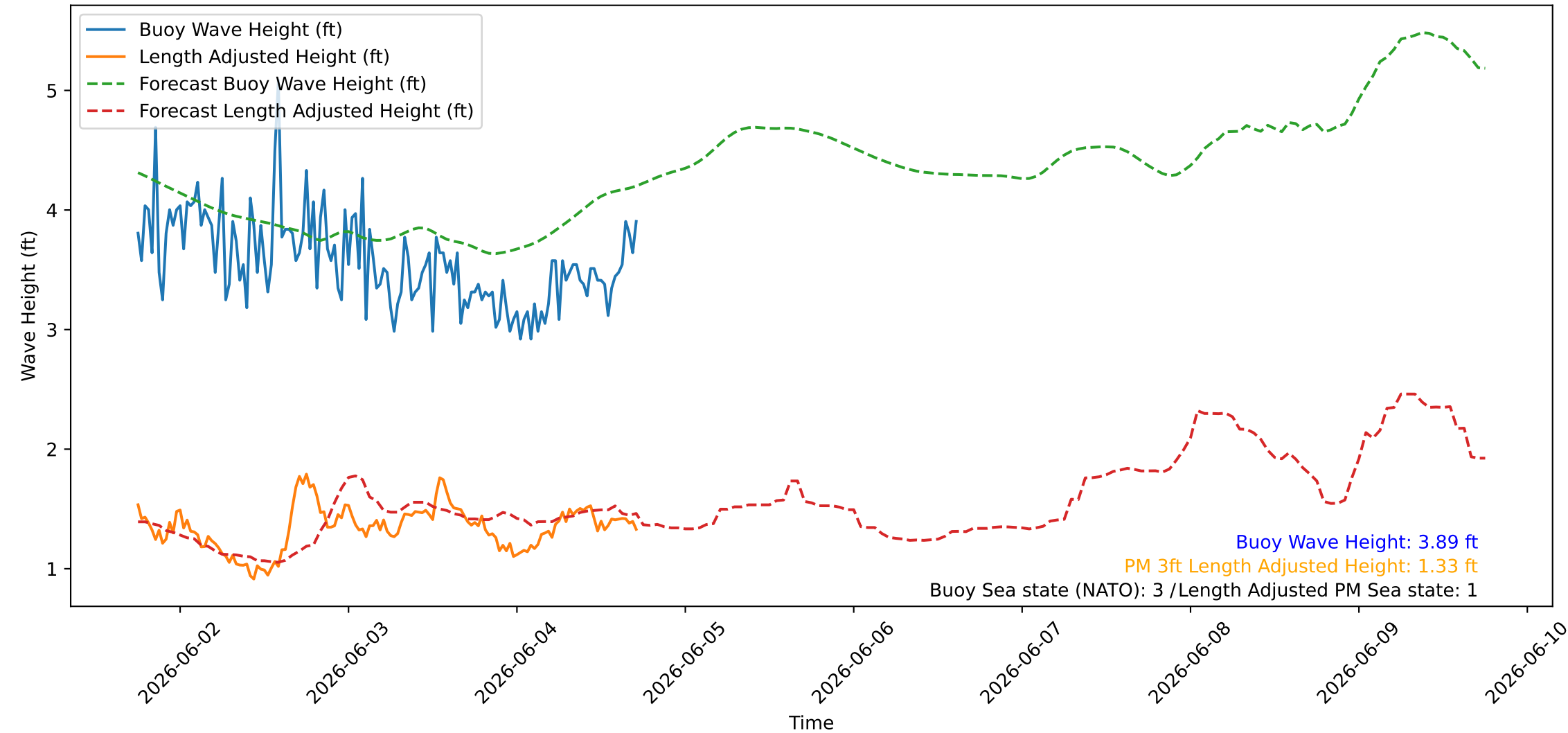
Wave Heights over Time for Oceanside Harbor at 2026-06-04 18:00:26
