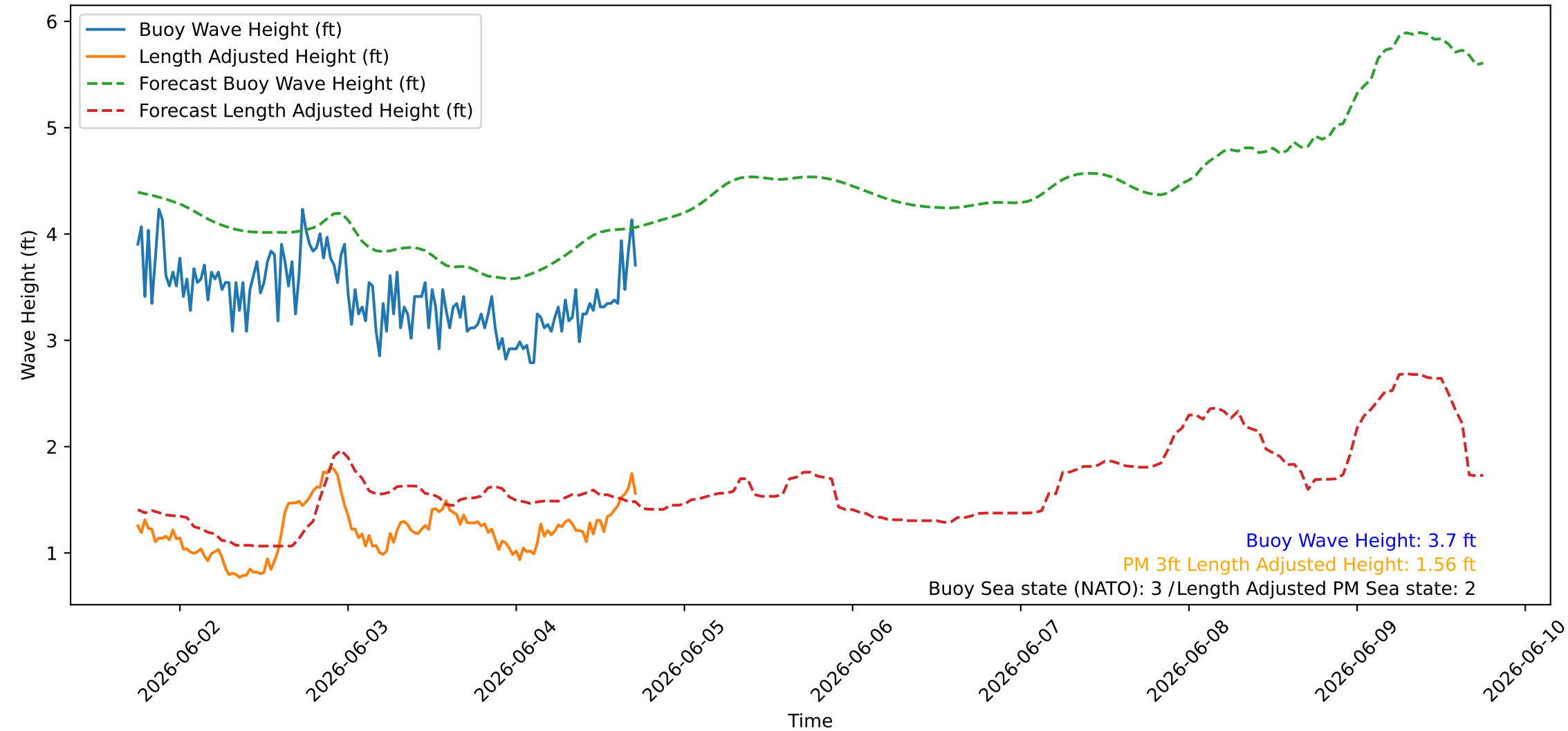
Wave Heights over Time for Green Beach at 2026-06-04 18:01:07
