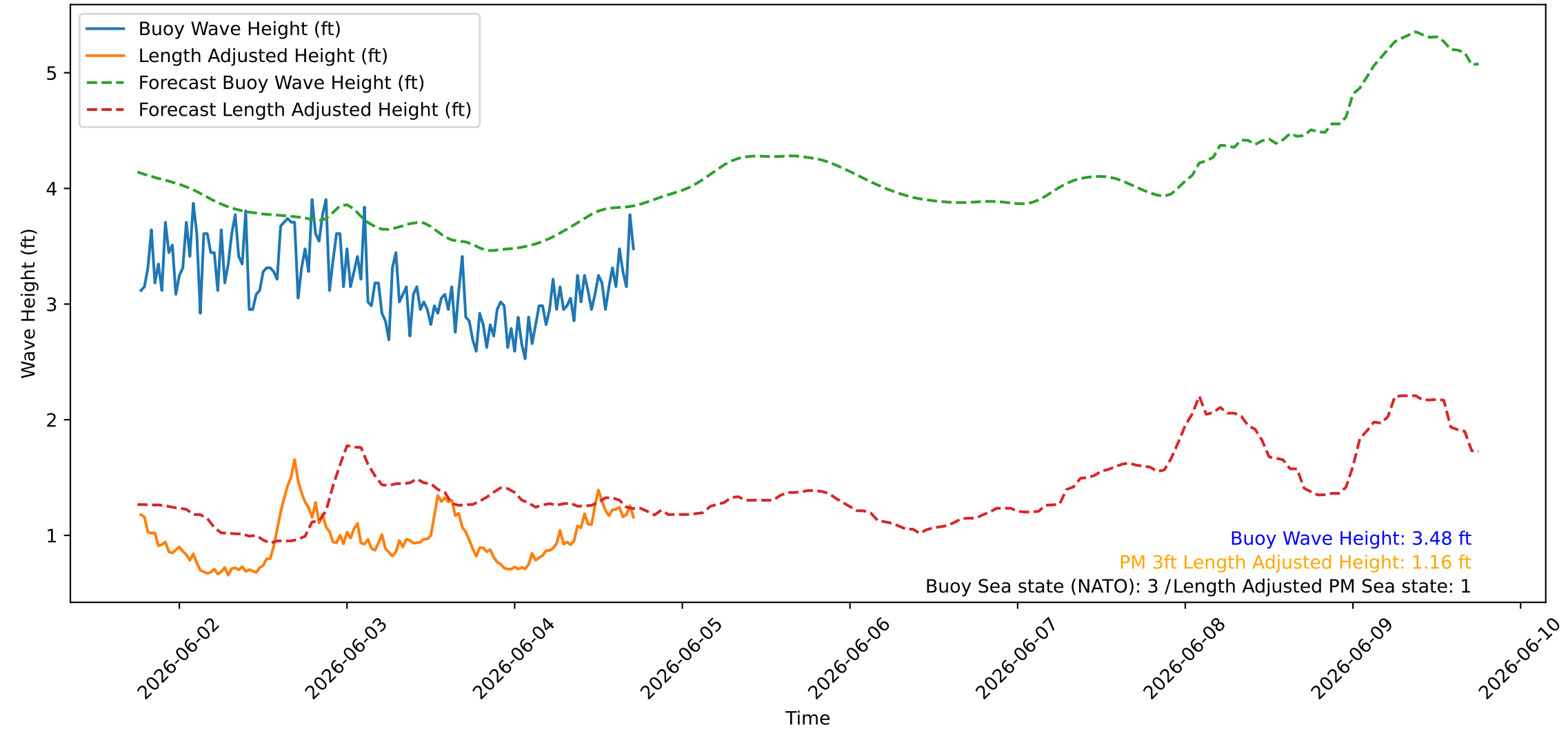
Wave Heights over Time for Red Beach at 2026-06-04 18:00:45
