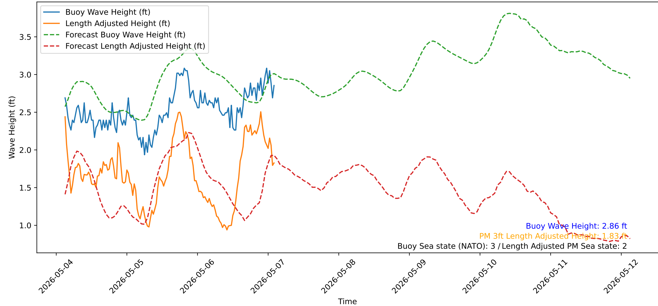
Wave Heights over Time for Red Beach at 2026-05-07 02:40:50
