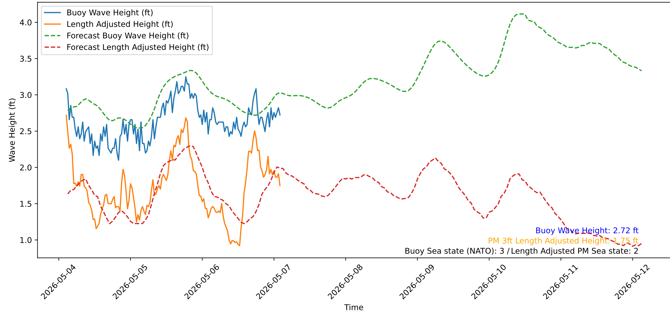
Wave Heights over Time for Oceanside Harbor at 2026-05-07 02:40:31
