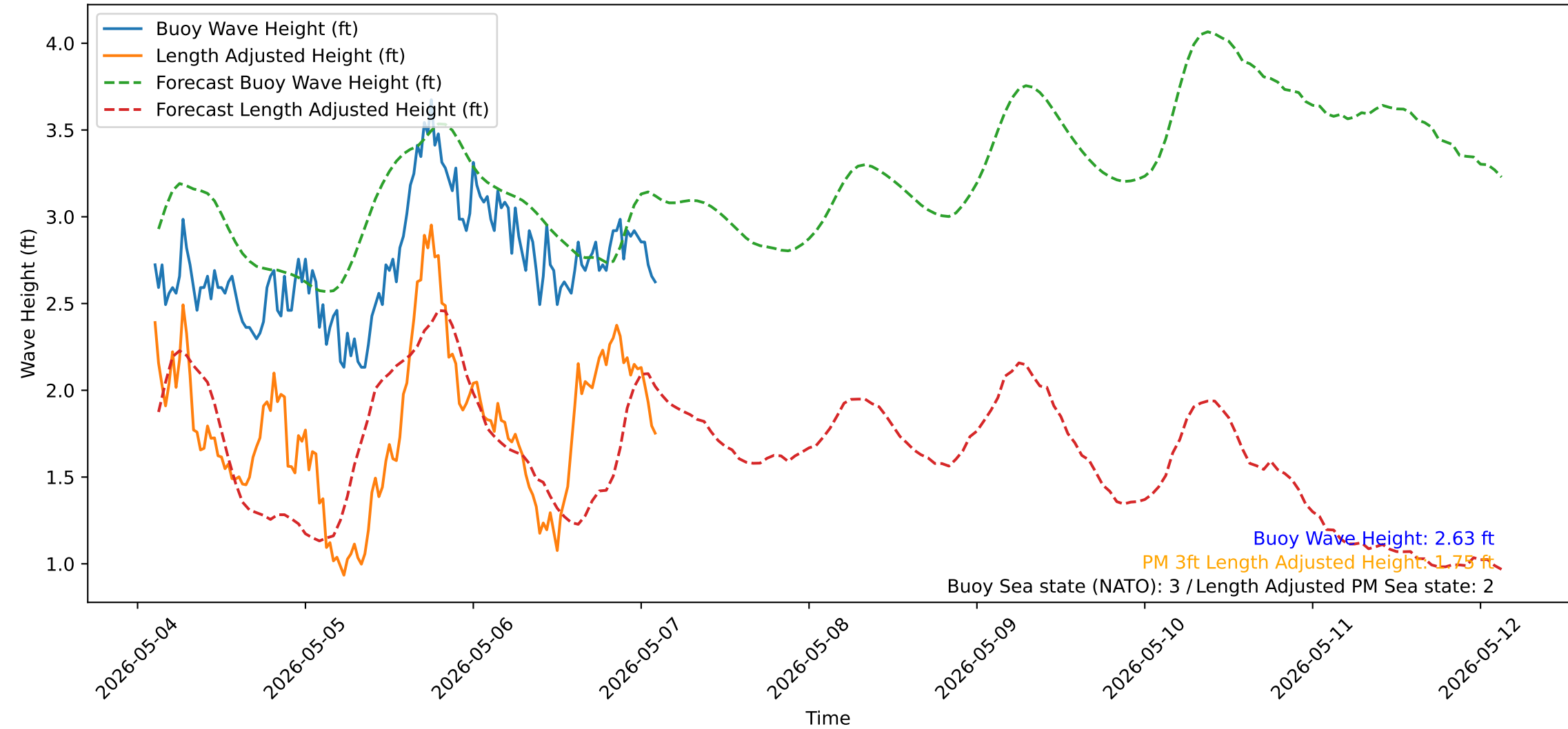
Wave Heights over Time for Green Beach at 2026-05-07 02:41:13
