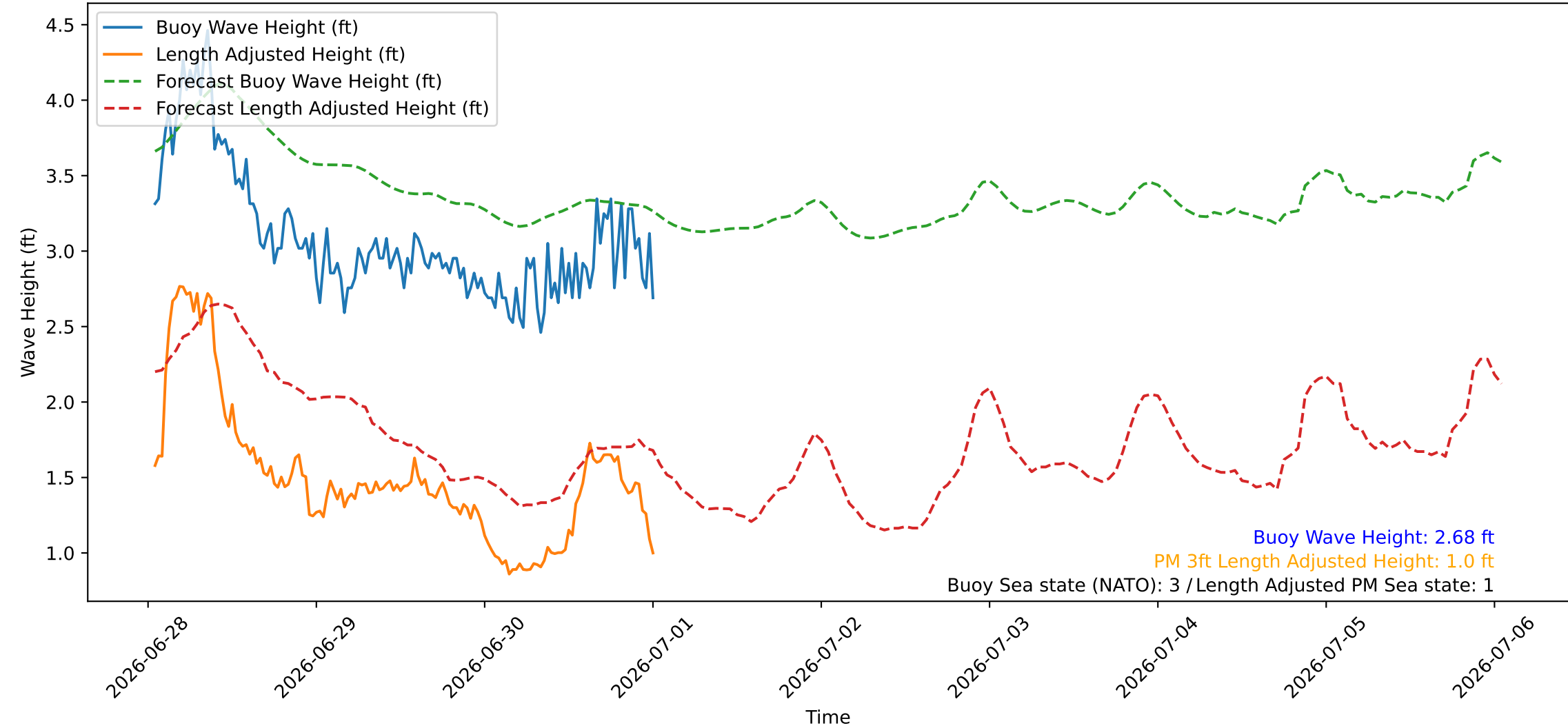
Wave Heights over Time for Red Beach at 2026-07-01 00:50:46
