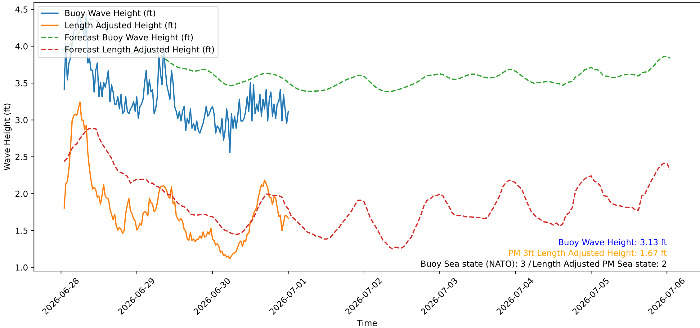
Wave Heights over Time for Oceanside Harbor at 2026-07-01 00:50:26
