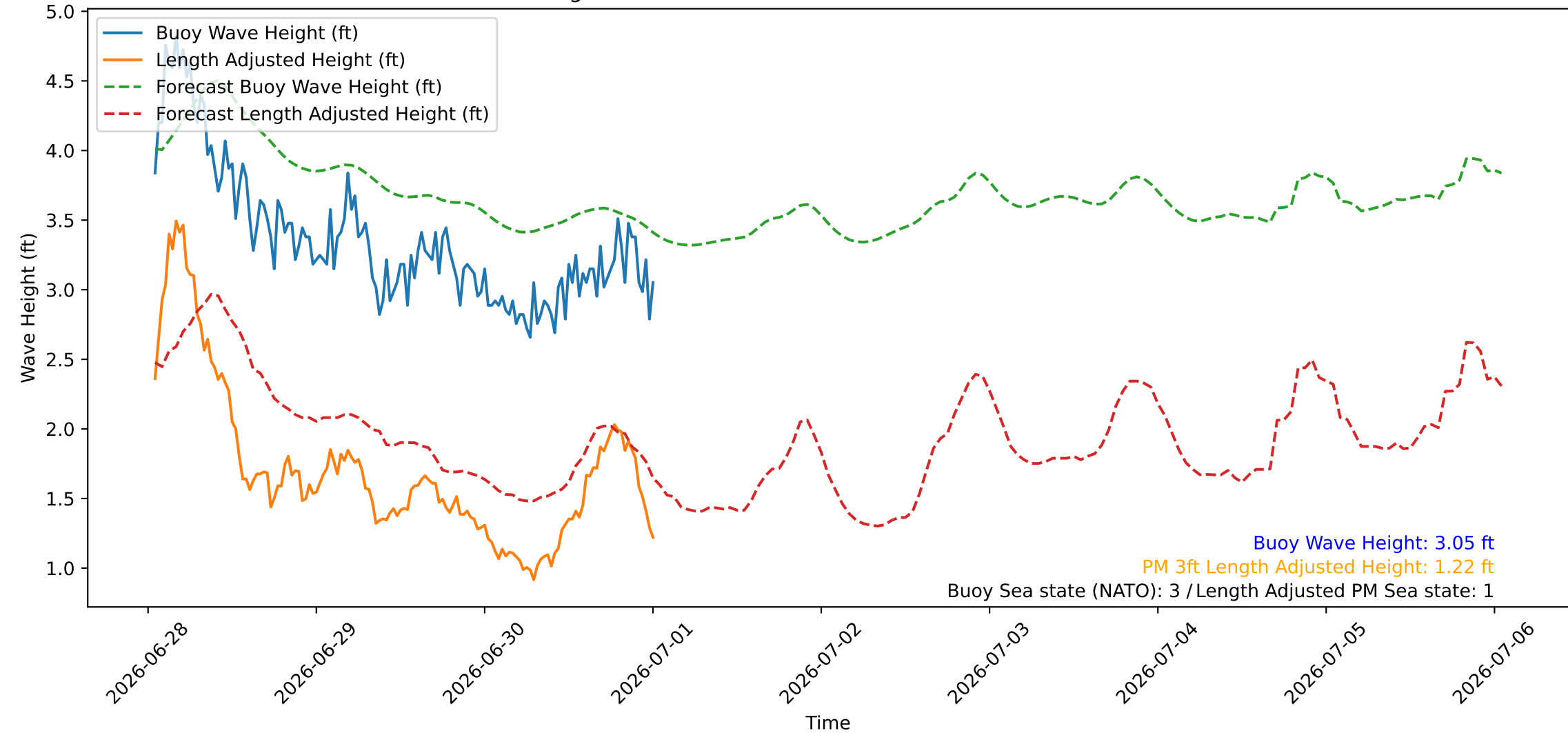
Wave Heights over Time for Green Beach at 2026-07-01 00:51:09
