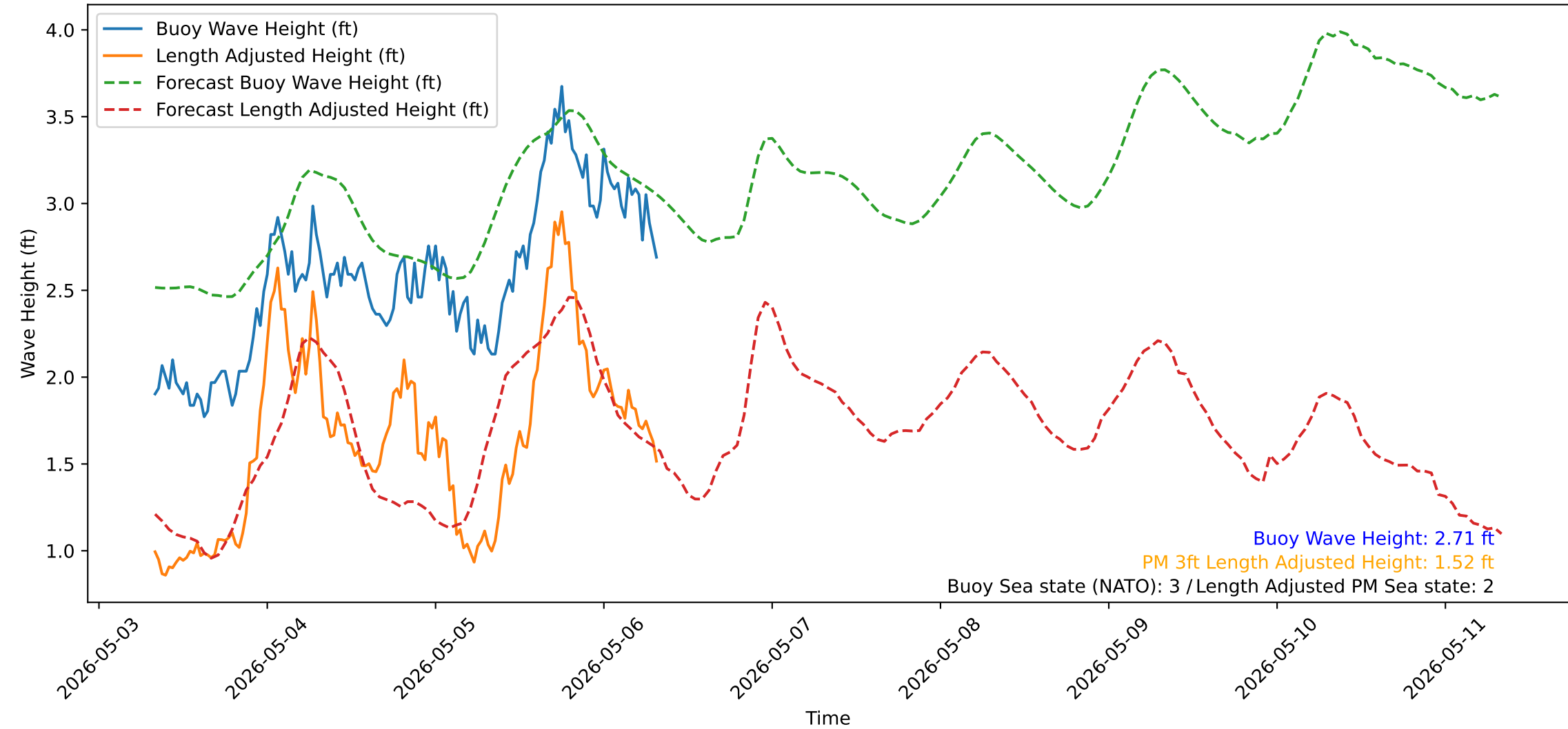
Wave Heights over Time for Green Beach at 2026-05-06 08:11:12
