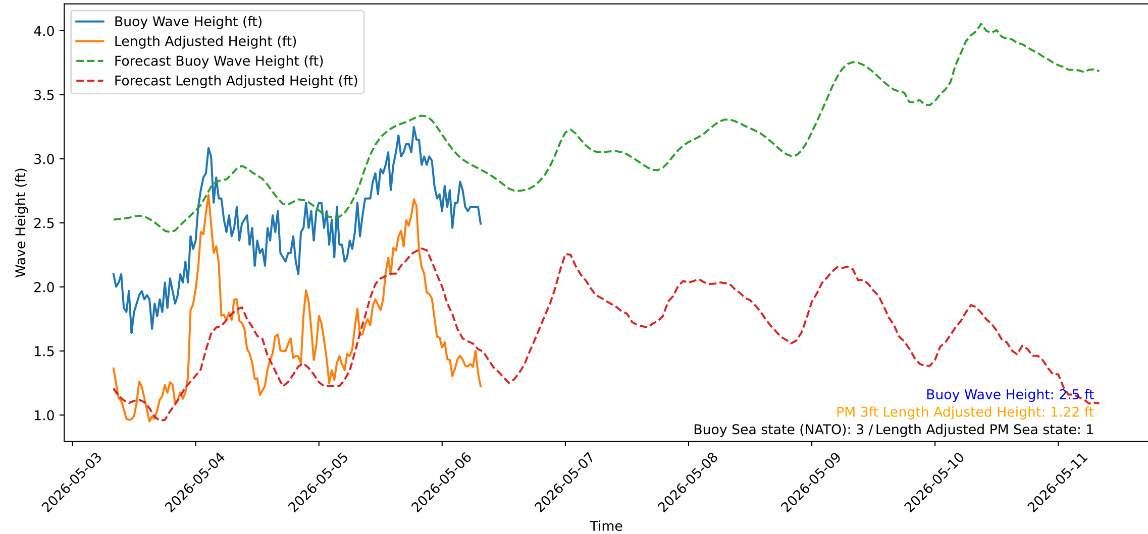
Wave Heights over Time for Oceanside Harbor at 2026-05-06 08:10:31
