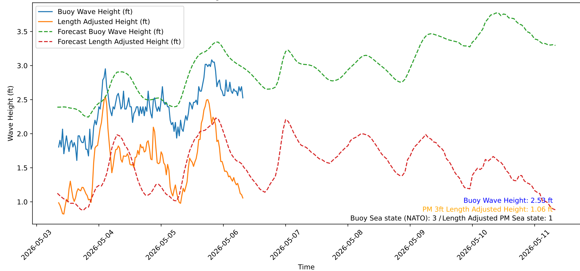
Wave Heights over Time for Red Beach at 2026-05-06 08:10:50
